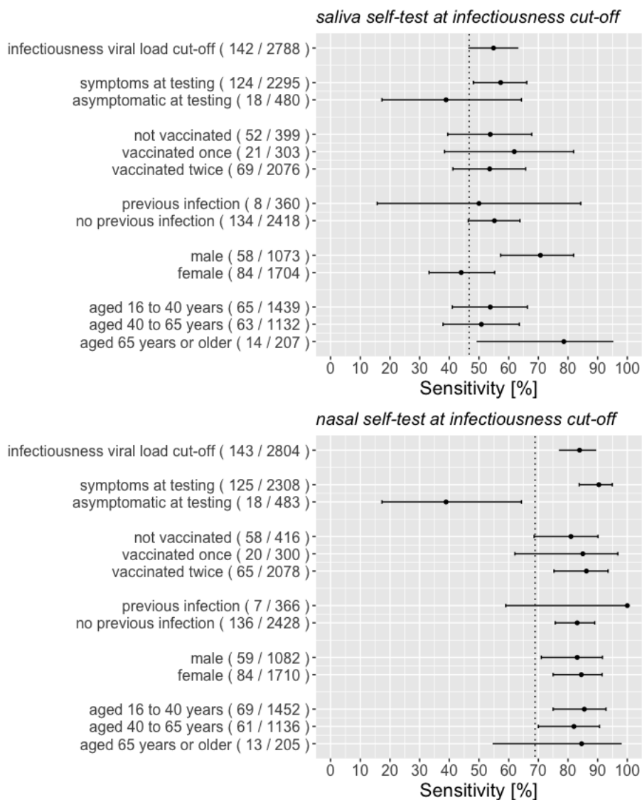
Figure S1 Sensitivities with 95% confidence intervals of the antigen rapid test-molecular reference standard test comparisons at viral load cut-off for infectiousness (i.e., viral load <5.2 \log_{10} SARS-CoV-2 E-gene copies/mL is considered as a negative reference test result), stratified according to symptomatology, COVID-19 vaccination status, previous infection status, sex, and age. The vertical line indicates the sensitivity of the Ag-RDT in the overall study population before application of a viral load cut-off (see Figure 2), and the number of positive molecular tests out of the total or subgroup between parentheses.
