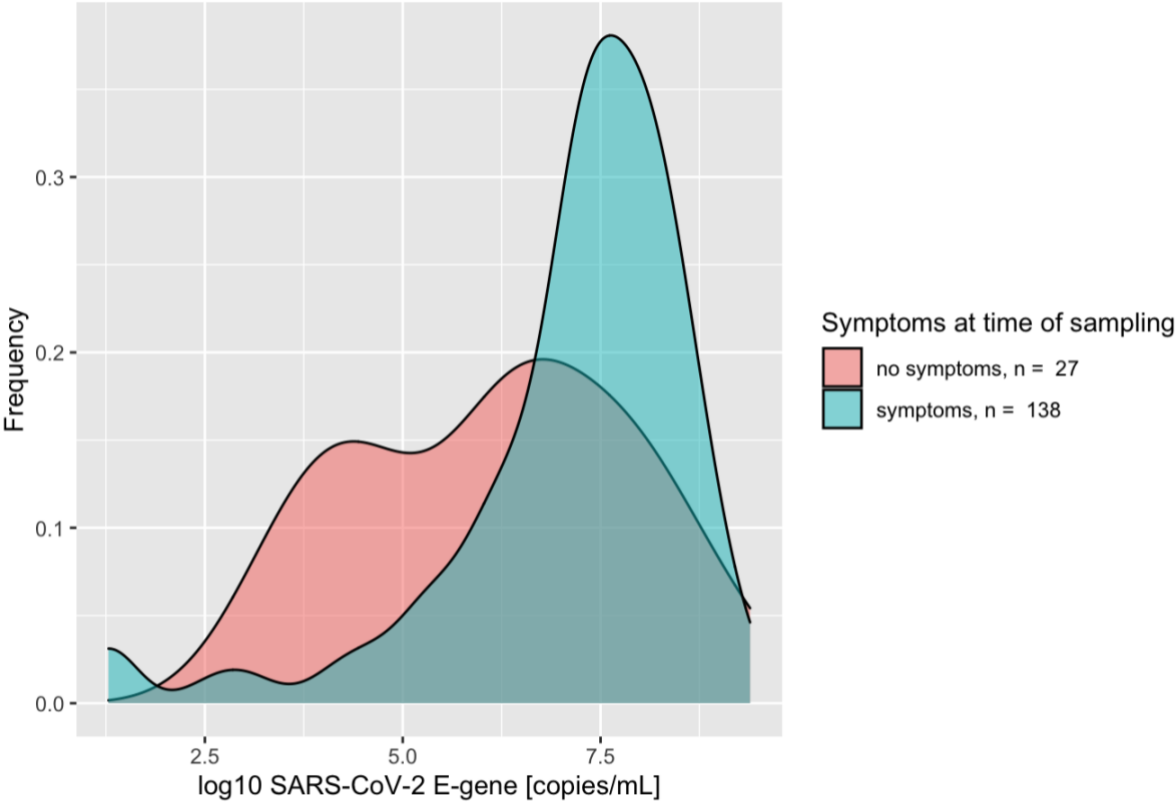
Figure S2 Distribution of viral loads in participants with a positive molecular reference test, stratified by symptomatology at time of sampling.
