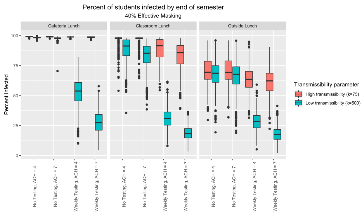
Figure 1: Box and whisker plots comparing scenarios with 40% masking effectiveness
