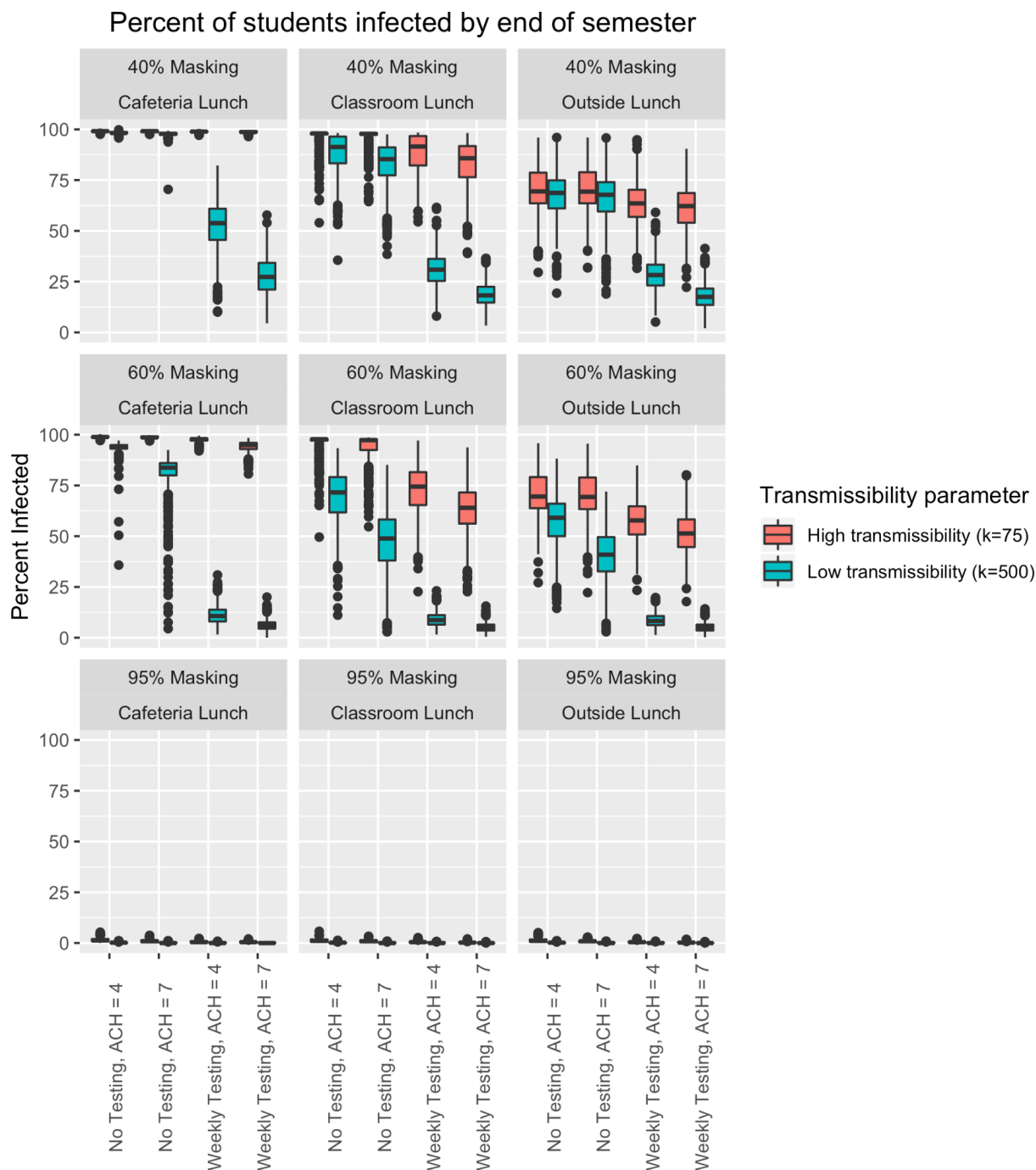
Figure 2: Box and whisker plots comparing scenarios with 40%, 60%, and 95% masking effectiveness
