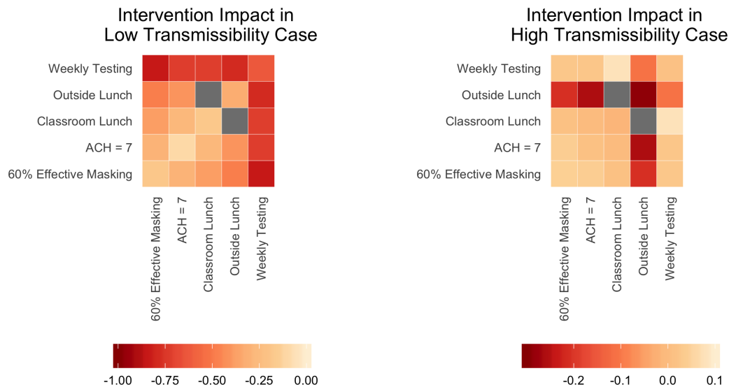
Figure 3: Cumulative impact of paired interventions by transmissibility case
