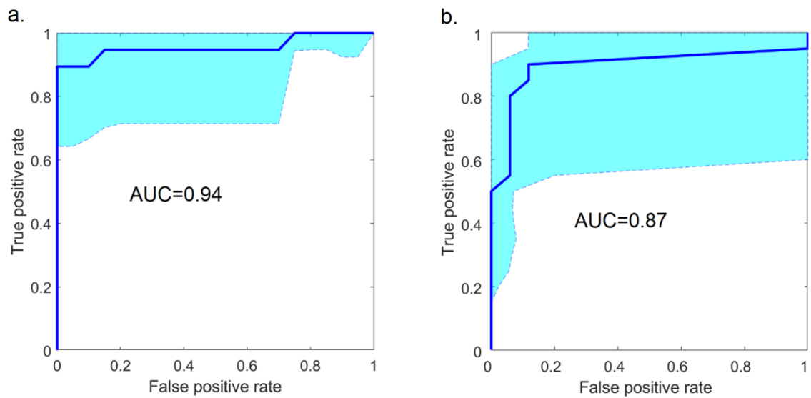
Supplementary figure2. (a) ROC corresponding to DFS to classify long vs. short survival time with AUC=0.94\pm 0.07 . 95% confidence interval shaded in blue (b) ROC corresponding to OS to classify long vs. short survival time with AUC=0.87\pm 0.17 . 95% confidence interval shaded in blue.
