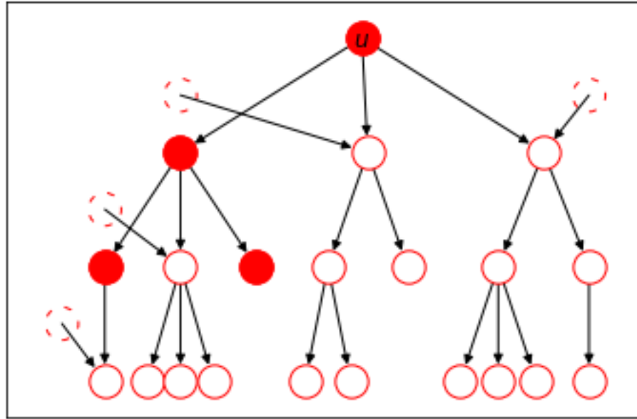
Figure 9: A schematic showing the descendants of u with filled circles showing those whose infections would be averted if u 's transmissions were prevented by u isolating. Dashed hollow circles denote infected individuals that are not descendants of u who provide additional transmission paths to some descendants of u . Hollow circles with solid edges denote the individuals whose infection is overdetermined.
