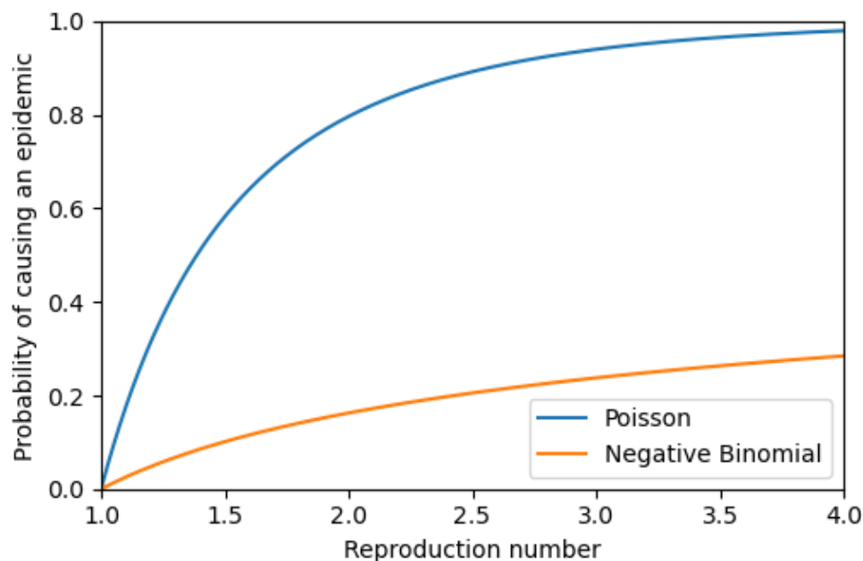
Figure 1: The probability a single infected individual entering a completely susceptible population causes an epidemic, assuming no other introductions. The offspring distribution follows either a Poisson distribution or a negative binomial distribution with a dispersion parameter of 0.16.
