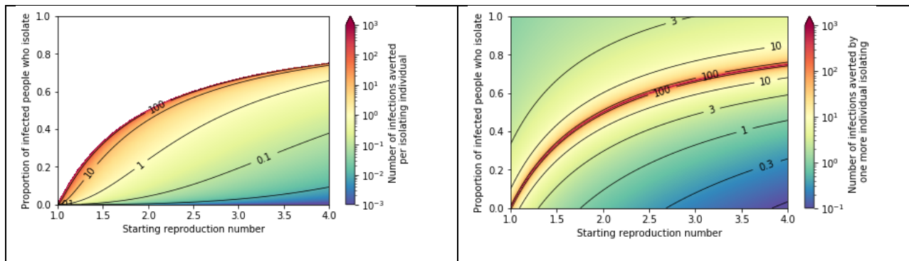
Figure 5: Measuring the effectiveness of many individuals isolating. Left The average impact assuming that others interventions set a starting value of \mathcal{R}_c , but in addition to that an additional fraction of the infected individuals isolate. Calculations are done in the limit of an infinite population. As the fraction of infections isolating increases, the size of the epidemic decreases. Eventually a larger fraction isolating translates to a smaller absolute number isolating due to the smaller epidemic. When enough isolate to drive the resulting \mathcal{R}_c close to 1 almost all infections are averted while only a small fraction of the total population isolate, so the number of infections averted per isolating individual diverges. Beyond this threshold (white region), epidemics are impossible and the number of infections averted per infected individual is infinite. Right The marginal benefit of one more infected individual isolating. That is, given the fraction isolating and the initial \mathcal{R}_c , this gives the number of infections averted if one additional infected individual who would not isolate is successfully identified and isolated.
