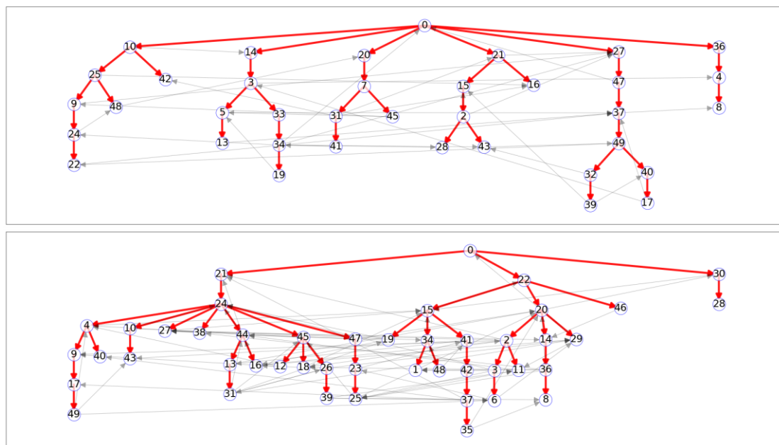
Figure 8 Two sample outbreaks with \mathcal{R}_c = 1.5 (top) and \mathcal{R}_c = 2.5 (bottom), each starting from a single infection in a population of 50 individuals. Only the eventually infected nodes are shown. The red lines denote successful transmissions while the gray lines denote transmissions from an infectious individual to one who had already been infected. Note that given the transmissions in the \mathcal{R}_c = 1.5 case, had individual 36 (second row on right) been the initial infection, only individuals 36, 4, and 8 would have been infected. Additionally, had individual 49 (fifth row on right) isolated after infection (or been effectively protected from infection), this would have prevented the infections of 32, 39, 40, and 17. In the \mathcal{R}_c = 2.5 case, there are many more (potential) transmission chains: more infections occur,
