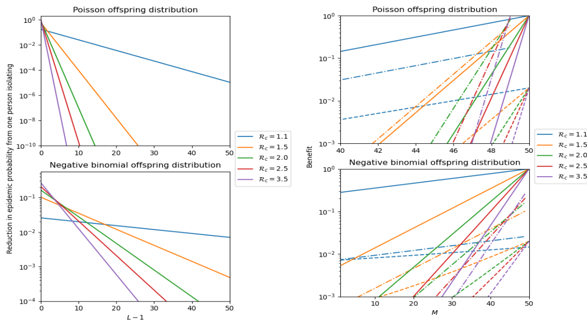
Figure 2 The benefit measured as the reduction in probability of an epidemic. We use a Poisson offspring distribution and a Negative Binomial offspring distribution with dispersion 0.16. We assume that L infected individuals enter the population of whom M isolate. Left (note different vertical scales): The reduction in epidemic probability if M = 1 (only one isolates) as a function of the number ( L - 1 ) who do not isolate. Due to overdetermination, this decreases as L increases. Right (note different horizontal scales): The reduction in probability if M isolate out of L = 50 introduced cases. This shows the total reduction in epidemic probability (solid line), the reduction averaged across the M isolating individuals (dashed line), and the marginal benefit of one more isolating individual, (i.e., the increased reduction in probability if one more were to isolate) (dash-dot line). As a consequence of overdetermination each additional individual who isolates increases the average impact of all isolating individuals.
