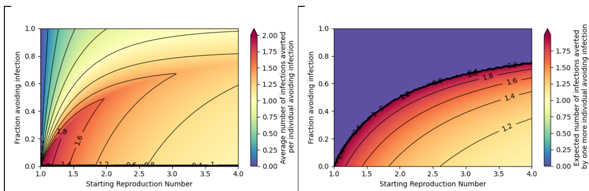
Figure 7: Measuring the impact of many individuals taking actions (such as a vaccine or prophylactic medication) to avoid infection. Left: The number of infections averted over the entire population taking protective action. Until enough individuals take action to prevent an epidemic, the average is greater than 1, and the average increases until the threshold is
