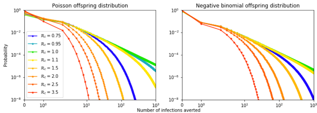
Figure 4: The distribution of the number of infections averted if a single individual isolates after infection. Calculated for Poisson and Negative binomial distribution (with dispersion parameter 0.16). For \mathcal{R}_c = 1 the result is a power law distribution. If \mathcal{R}_c is larger or smaller than 1, the distribution falls off quicker. For a given \mathcal{R}_c , both distributions have the same mean, but the Negative binomial distribution results in a more heterogeneous outcome.
