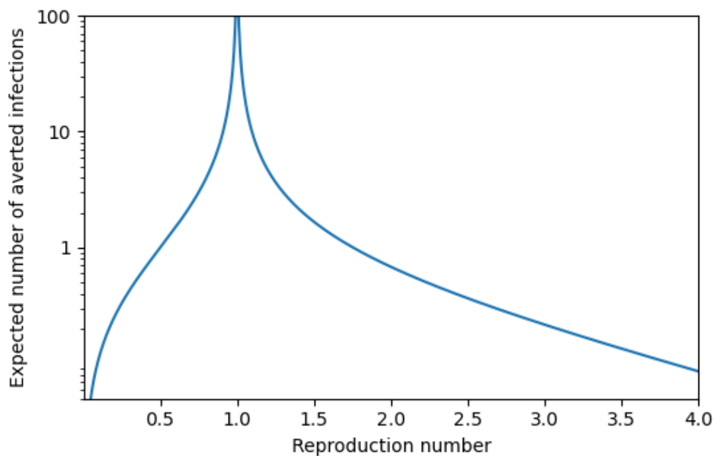
Figure 3 The expected number of averted infections, \mathcal{F}(\mathcal{R}_c) , due to a single infected individual isolating after infection and not transmitting, after accounting for overdetermination. The result is independent of the specific offspring distribution. This depends only on the average, \mathcal{R}_c . Note the divergence to \infty as the reproduction number \mathcal{R}_c \rightarrow 1 , and the decay to 0 as \mathcal{R}_c decreases towards 0 or increases towards \infty .
