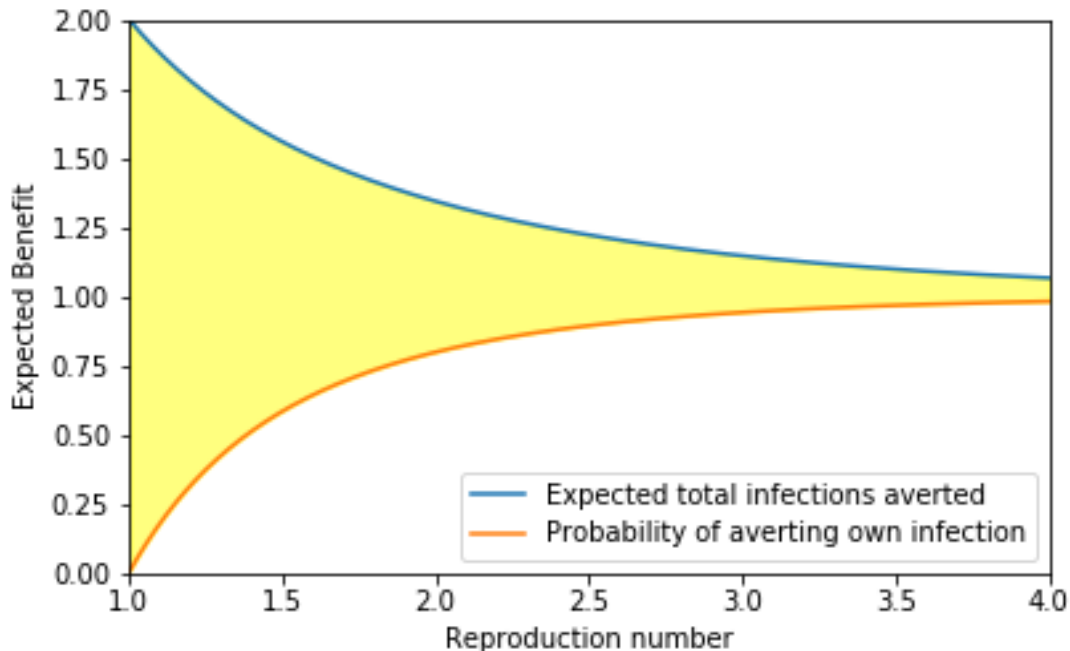
Figure 6: The expected number of infections averted by an individual taking sufficient action (such as a vaccine or prophylactic medication) to prevent her own infection (top blue curve). This is partly from the probability that she prevents her own infection [bottom orange curve, equal to \mathcal{A}(\mathcal{R}_c) ]. The difference between the two curves (shaded yellow) is \mathcal{F}(\mathcal{R}_c)\mathcal{A}(\mathcal{R}_c) ,
