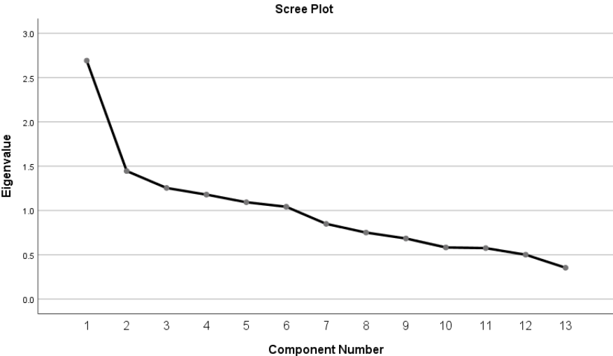
Figure 3: Scree plot
