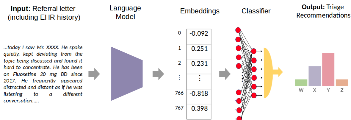
Figure 2: Data Pipeline for CHRONOSIG -- patients' free-text referral and historical EHR clinical data are used (without a priori human annotation) as input to a language model neural network. The resulting numerical representations of patients' data (denoted "embeddings" or longitudinal fingerprints) are the input to a moderately-sized downstream supervised neural network classifier that learns associations between treatment teams and the embedding representations.
