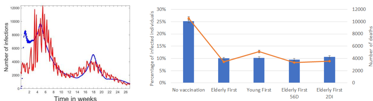
Figure 3: On the left, results for model validation. These results include the aggregated number of infected individuals for the area under study. Real and simulated data are shown in red and blue, respectively. The simulated curve corresponds to the baseline scenario. On the right, simulation results that include the percentage of infected population in blue bars and the number of deaths in orange, for each one of the vaccination strategies.
