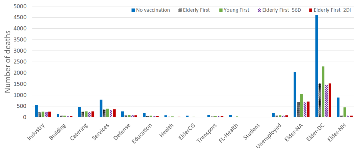
Figure 5: Number of deaths at the end of the simulation, broken down by groups. The acronyms are identical to those in Figure 4.
