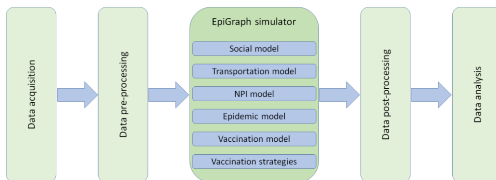
Figure 1: EpiGraph data flow: data acquisition and preprocessing to read and configure the input data, followed by agent-based simulation and output data post-processing and analysis
