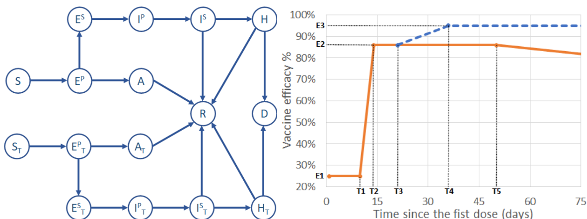
Figure 2: Left: Compartmental model used by EpiGraph that consists of the following states: susceptible ( S ), primary exposed ( E^P ), secondary exposed ( E^S ), asymptomatic ( A ), primary infected ( I^P ), secondary infected ( I^S ) hospitalized ( H ), recovered ( R ) and dead ( D ) individual. States with subindex T ( S_T , E_T^P , etc.) are related to vaccinated (treated) subjects. Right: Vaccination model with values corresponding to Pfizer-BioNTech vaccine. The efficacy of a single dose is displayed in a solid orange line. The second dose efficacy is represented as a dashed blue line. E_1 , E_2 and E_3 represent the minimum, first and second dose efficacies, respectively. T_1 is the time when the first dose starts increasing the efficacy, T_2
