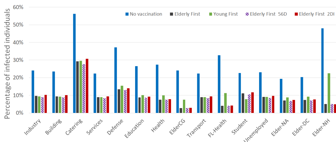
Figure 4: Percentage of infected population at the end of the simulation, by groups. The acronyms stand for: ElderCG - caregiver for elderly people; Health - non-front-line health professionals; FL-Health - front-line health professionals; Elder-NA - elderly that live by themselves; Elder-DC - elderly attended in daily centers; and Elder-NH - elderly that live in nursing homes.
