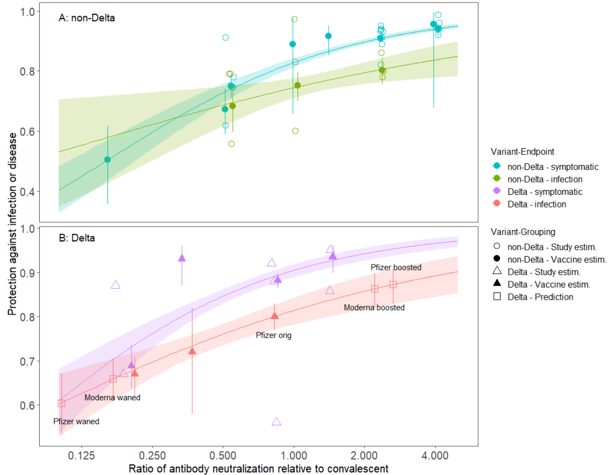
207 Fig. 1. Protection against symptomatic infections or all infections plotted against the ratio 208 of neutralizing antibody titers relative to convalescent sera. Each round point represents an 209 estimate of vaccine efficacy for a single vaccine & virus variant (from randomized control 210 trials) or vaccine effectiveness (from observational studies) or an estimate of protection 211 from previous infection from observational studies. Square points show predicted values 212 using the fitted model and measured neutralizing antibody titers after waning (Moderna: 6 213 months; Pfizer 8 months) or boosting. Colors show the SARS-CoV-2 variant (Delta or non- 214 Delta) and endpoint of the study (symptomatic infections or all infections). Closed symbols 215 and 95% CIs show aggregated data for each vaccine-variant-endpoint. Open symbols show 216 estimates from individual studies if there were more than one estimate for a vaccine- 217 variant-endpoint. Points have been jittered along the x-axis to facilitate presentation; all 218 points for the same vaccine-variant have the same x-value. Lines show fitted models with 219 protection as the response and an interaction between and neutralizing antibody ratio and 220 variant-endpoint as predictors (Table S3). Panel B shows data and relationships for the 221 Delta variant, with all points shifted 2.88-fold lower along the x-axis to reflect the lower 222 neutralizing antibodies observed with this variant across studies (Table S2).
