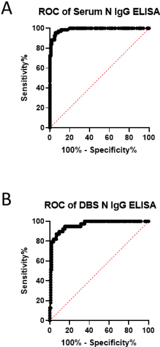
Supplemental Figure 3. Receiver-Operator Curves (ROC) of the validation of (A) the anti-N IgG ELISA in serum or of (B) the anti-N DBS ELISA.
