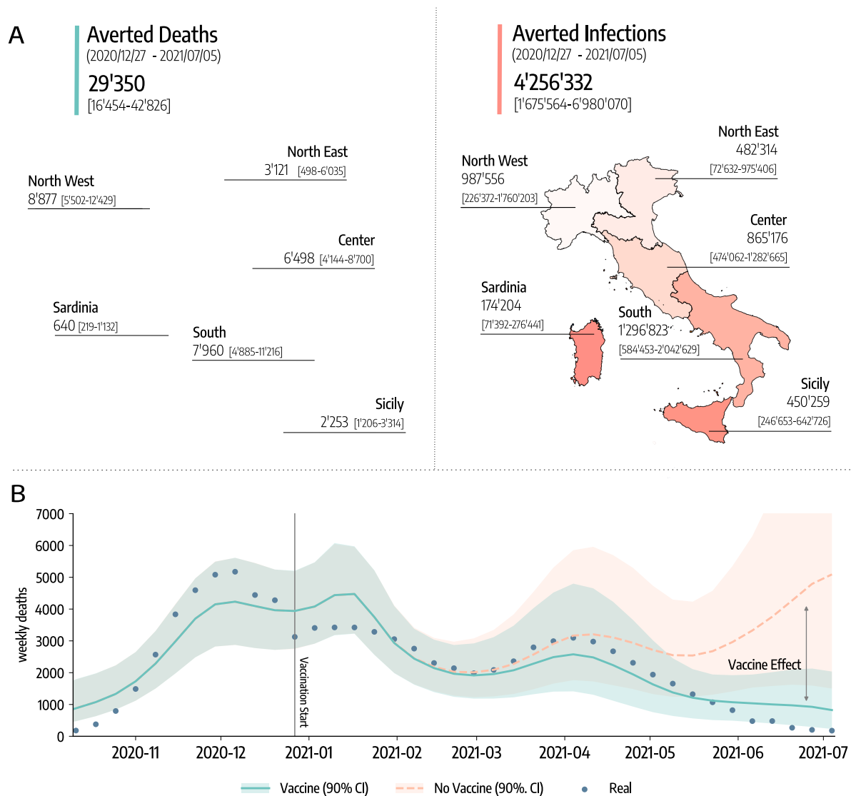
Figure 3: Averted deaths and infections. A) Estimated averted deaths and infections in different regions considered with respect to a baseline without vaccines. Median and interquartile ( IQR ) range are reported. B) Number of weekly deaths at the country level as reported by official surveillance and as estimated by our model with and without vaccines rollout (median and 90% confidence intervals displayed).
