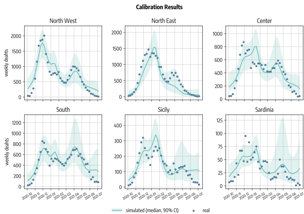
Figure 8: Calibration Results. Simulated (median and 90% CI) and observed cumulative number of deaths.
