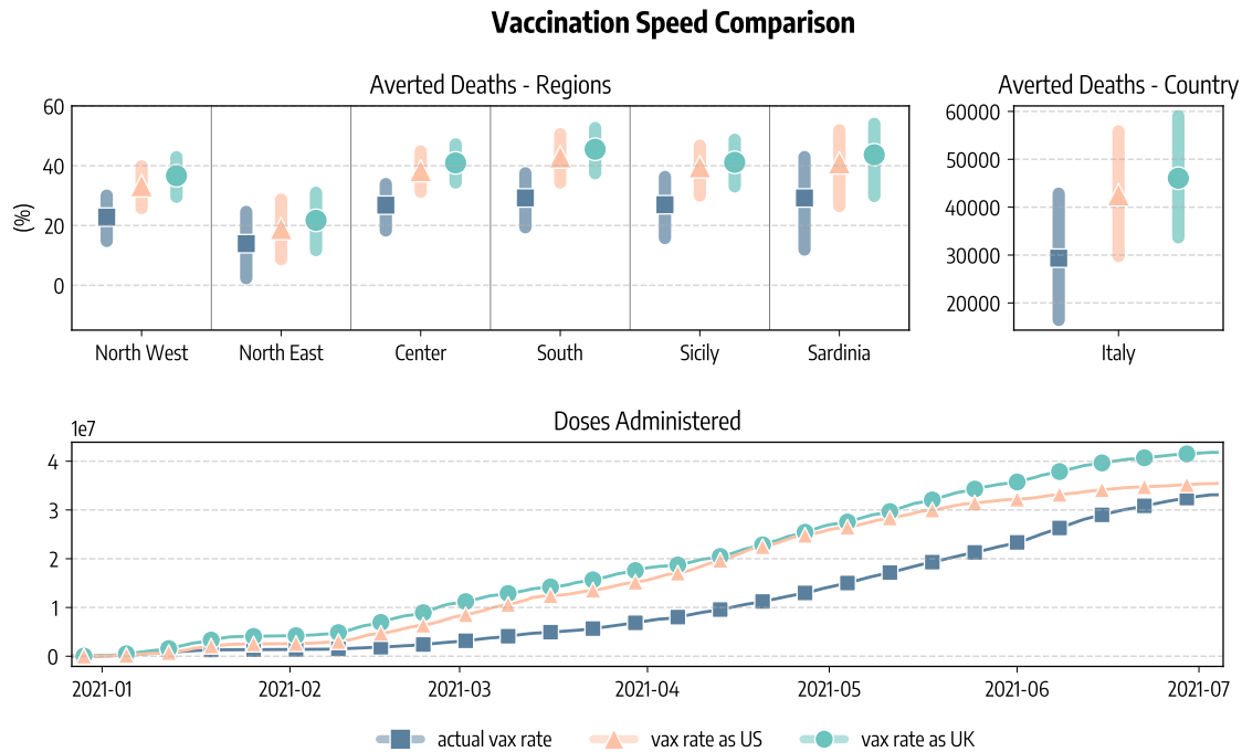
Figure 5: Comparison of vaccination speeds and doses. We show the percentage of deaths averted with respect to simulations without vaccines in different regions considering the real data-driven campaign, and rescaling the number of doses to match those administered in the United Kingdom and the United States. We also report the estimated total number of deaths (median and IQR) averted in Italy as well as the number of cumulative doses administered in the scenarios.
