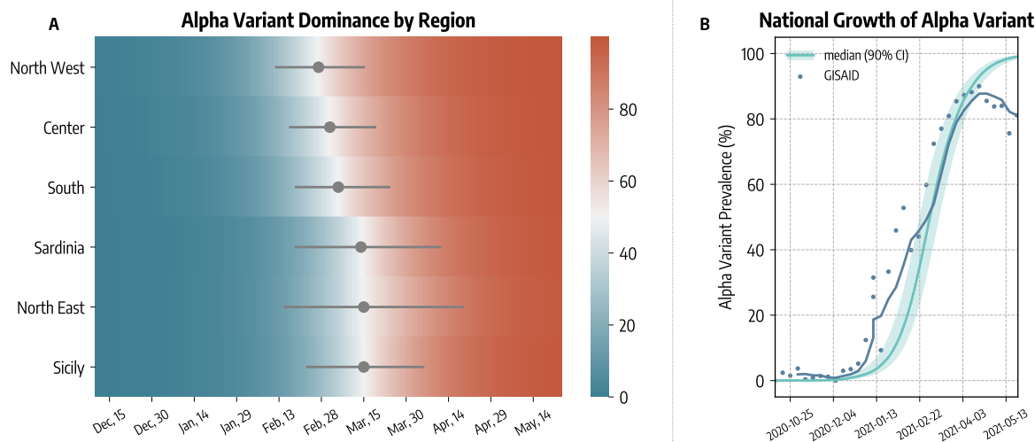
Figure 2: Alpha Variant Spreading and Dominance. A) Estimated date of dominance of the Alpha variant in different regions. B) Comparison between estimated and reported national prevalence of Alpha variant.
