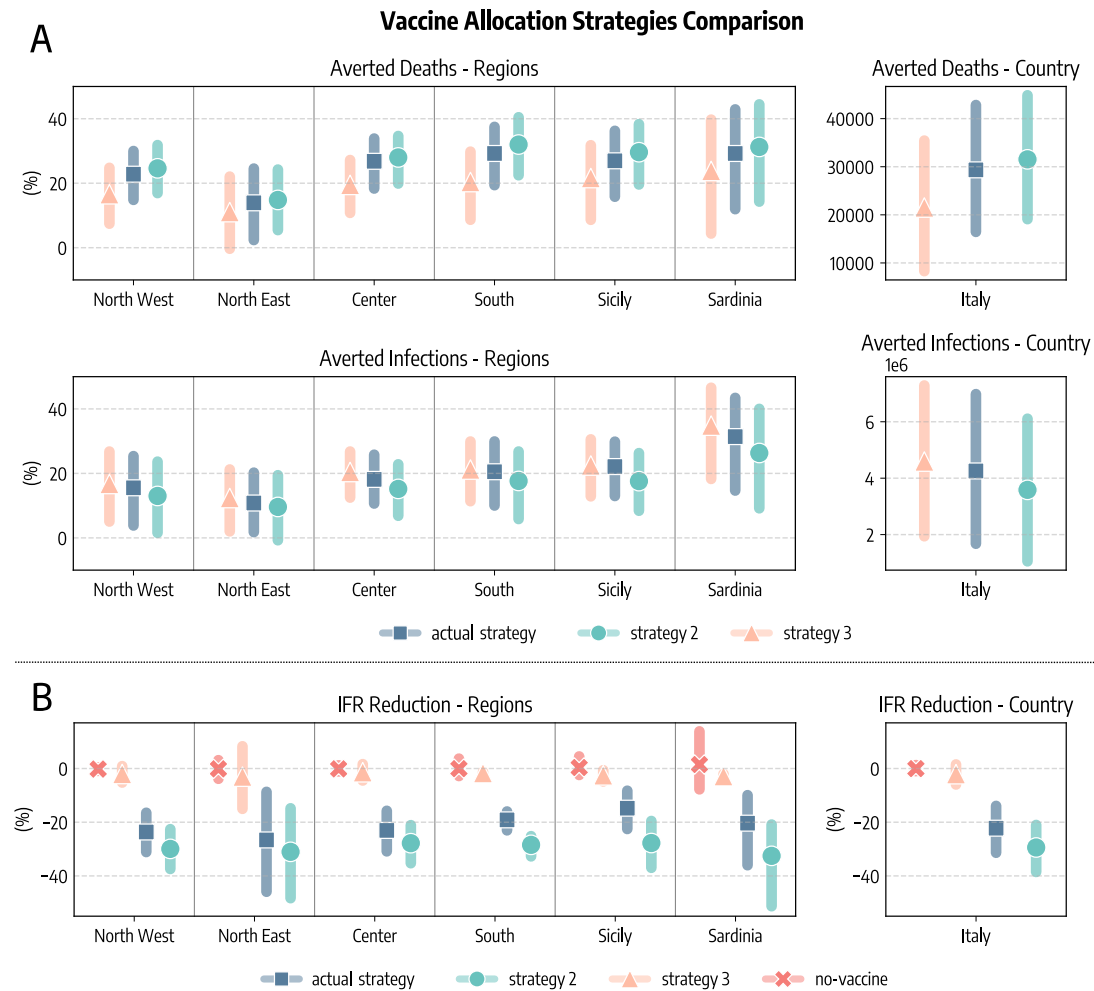
Figure 4: Comparison of vaccine allocation strategies. A) Averted COVID-19 deaths and infections, both at subnational and national level (medians and interquartile ranges are reported). B) Percentage reduction of the Infection Fatality Rate as of 2021/07/05. In all panels, actual strategy denotes an allocation strategy that follows the observed allocation as it unfolded during the pandemic, strategy 2 considers the case where vaccines are allocated in decreasing age order starting from the 80+, strategy 3 considers the case in which vaccines are first allocated to the age groups 20 – 49 and then homogeneously to the rest of the population, and no-vaccine denotes the counterfactual scenario in which vaccines were not administered.
