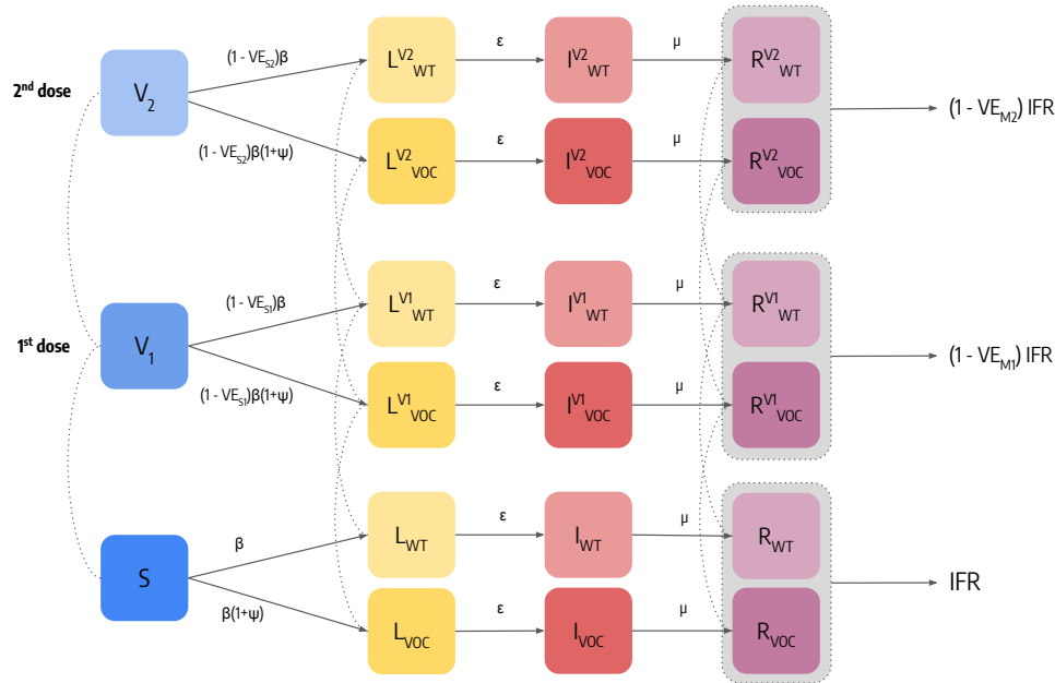
Figure 6: Schematic representation of the epidemic model and transitions between compartments. For simplicity, we represent the model for a single age group.
