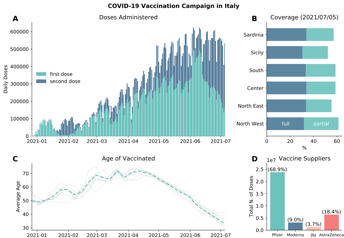
Figure 1: Vaccination campaign in Italy. A) Number of daily first and second administered daily in the country. B) Percentage of total population vaccinated with one/two dose in different regions considered. C) Average age of those who received the first dose of vaccines (dashed line). Grey lines indicate the average age of vaccinated in different regions considered. D) Total number of first doses administered between 2020/12/27 and 2021/07/05 by vaccine supplier.
