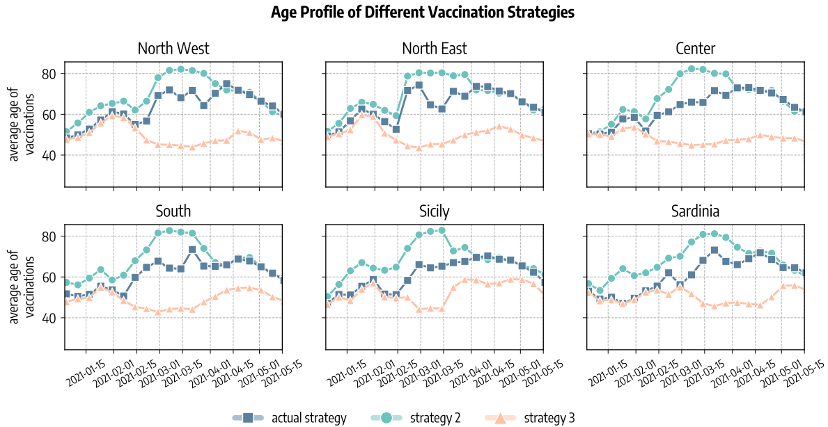
Figure 7: Average age of vaccinated in different allocation strategies. Actual strategy denotes the observed vaccine allocation as it unfolded during the pandemic, strategy 2 considers the case where vaccines are allocated in decreasing age order starting from the 80+, and strategy 3 considers the case in which vaccines are first allocated to the age groups 20 – 49 and then homogeneously to the rest of the population.
