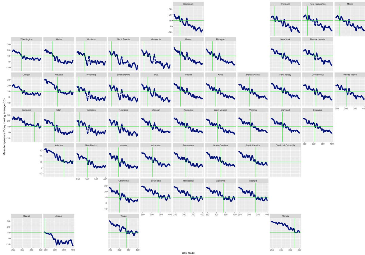
Fig. S2 Measuring the date when temperature reaches 10°C. The x-axis is day counts since January 1 st 2020, and the y-axis is the mean temperature 7-day moving average. Each figure represents a state which are organized roughly by their locations in the US geological map. Data for the District of Columbia and Hawaii were not available. The horizontal green line indicates the temperature threshold used in this example (10°C), and the vertical line indicates the day at which the state's curve reaches that threshold within +/-1°C.
