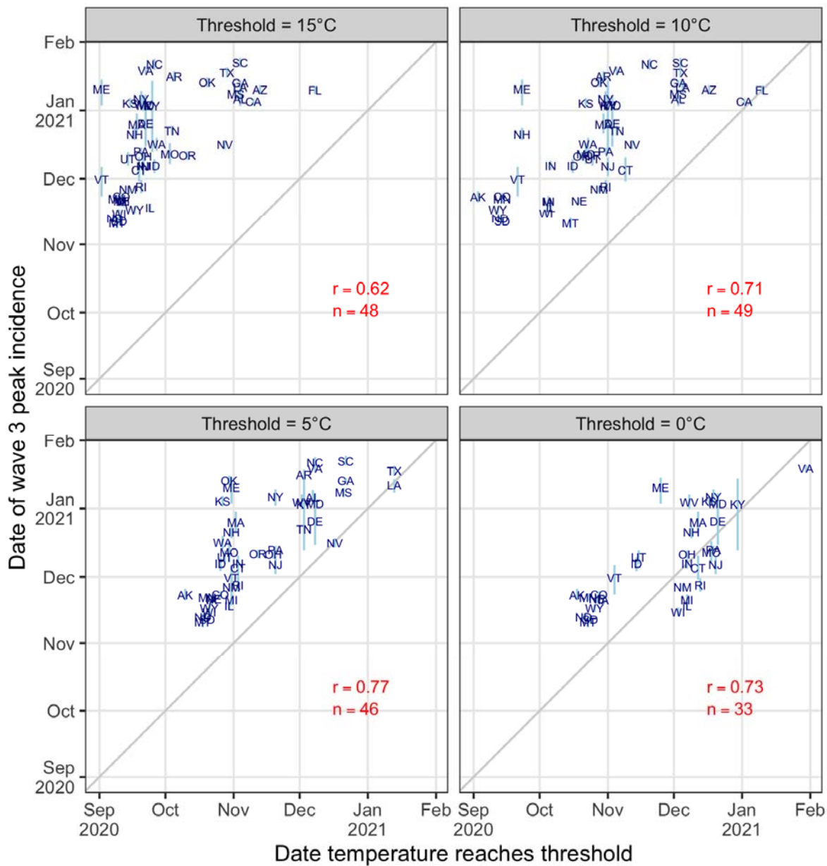
Fig. S3. Temporal association between average temperature and Wave 3 peak incidence. Each plot shows a specific temperature threshold. The x-axis displays the date on which the average temperature in each state reaches the specified threshold within \pm 1^\circ\text{C} , and the y-axis is Wave 3's peak incidence date. The 2-letter abbreviations represent the USA states. The light blue vertical lines are the 95% credible intervals for the peak dates, r is the correlation between the two dates across states, and n is the number of states that reach the temperature threshold. This analysis excludes Hawaii due to missing temperature data.
