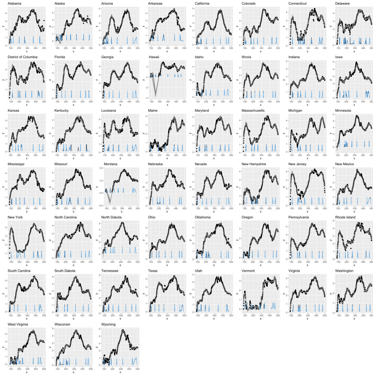
Fig. S1 Results of the multiple change point analysis by state. The x-axis is the days since January 1 st , 2020, and the y-axis is the log of 7-day moving average of case rates per 100,000. The gray lines are samples from the Bayesian posterior fitted piece-wise linear models, and the density plots at the bottom are the posterior densities of the seven change points. We used change points 1, 3, 5 and 7 to represent the days in which waves 1 through 4 peak, respectively.
