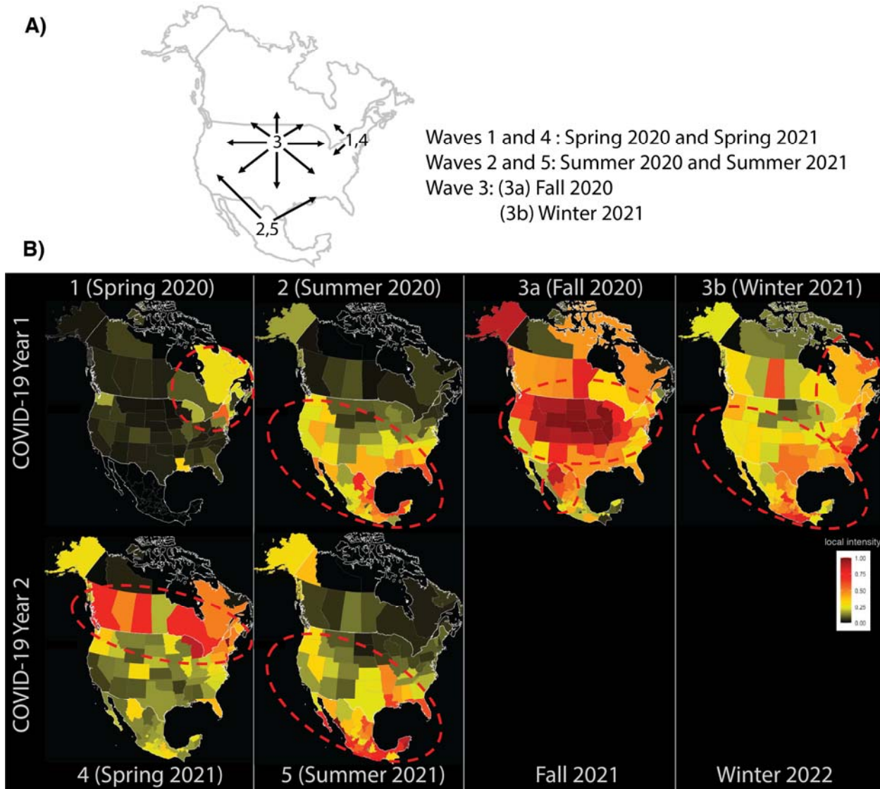
Fig. 3. Spatiotemporal patterns of COVID-19 waves in the US, Mexico, and Canada by season. Panel A is a diagram illustrating the three major seasonal waves that has spanned the continent. The arrows indicate the direction of the spread. Panel B shows frames taken from Movie 2 and reveals the geographical distribution of each wave and the similarity between the first and second year of the pandemic. The color scales represent the local intensity of cases on a scale from 0 to 1. As the movie shows, Wave 3a (fall 2020) continues through the winter months of 2021 (Wave 3b) as a travelling wave. The spring frames are for Apr 10, 2020 and 2021 (Waves 1 and 4), the summer frames are on July 28, 2020 and 2021, the fall frame represents Nov 20, 2020 (Wave 2 and 5), and the winter frame represents Feb 15, 2021 (Wave 3b). Mexico's state level data for Wave 1 was missing.
