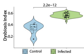
Figure S1: Centroid and Euclidian distance for dysbiosis index calculation in control and COVID-19 subjects. (A-B) Principal co-ordinate analysis centroid ordination of sample groups. Dysbiosis index calculated for each sample based on Euclidean distance from the centroid of the control sample. (C) The violin plot shows the dysbiosis indexes of samples from control and infected individuals (Wilcoxon rank sum test p value < 0.05 ).
