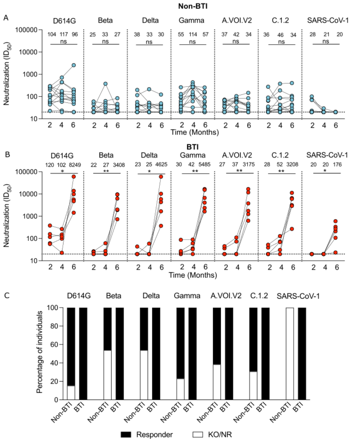
Fig. S2: Longitudinal neutralization responses over 6 months for BTI and non-BTI participants against SARS-CoV-2 variants and SARS-CoV-1. Neutralization ID 50 titers are shown for (a) Ad26.COVS2.S vaccinees that did not have breakthrough infection (non-BTI) and (b) BTI Ad26.COVS2.S vaccinees at 2-, 4- and 6-months, against D614G, Beta, Delta, Gamma, C1.2. and A.VOI.2 variants, and SARS-CoV-1. Significance is shown as per Friedman test, across all time points where ns denotes non-significant, *p<0.05; **p<0.01. (c) Percentage of individuals who are neutralization responders (Black; ID 50 >20), or are either non-responders or
