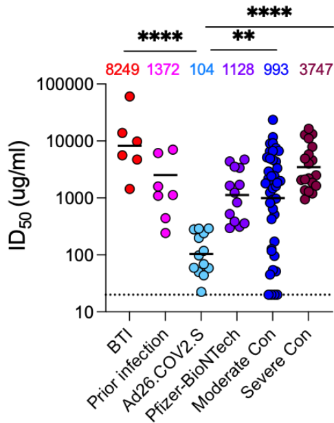
Fig. S3: BTI neutralization responses to the D614G variant compared to vaccinees and convalescent plasma. Neutralization ID 50 titers of two-dose Pfizer-BioNTech and one-dose Ad26.COVS2.S vaccinees (2-months post-vaccination) and hospitalised convalescent individuals with moderate and severe infection 10-days after a positive PCR test are shown compared to BTI individuals (1-month post-infection). Individuals who were previously infected by SARS-CoV-2 prior to Ad26.CoV2.S vaccination are shown 2-months post-vaccination. Limit of detection is indicated by a dotted line. GMT is indicated by the black bars and above the plot, while significant differences between groups, as calculated by Kruskal-Wallis ANOVA with Dunns correction, are shown above the graph with with ** denoting p<0.01 and **** denoting p<0.0001.
