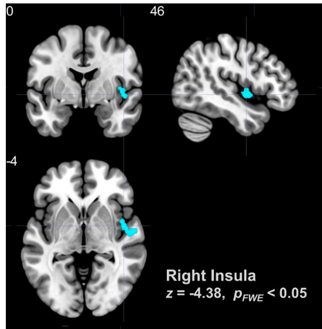
Figure. S1. Brain regions showing decreased GMV of patient vs healthy controls for studies pooled across GAD, FAD and MDD. Clusters were displayed at TFCE based FWE corrected p < 0.05 .
