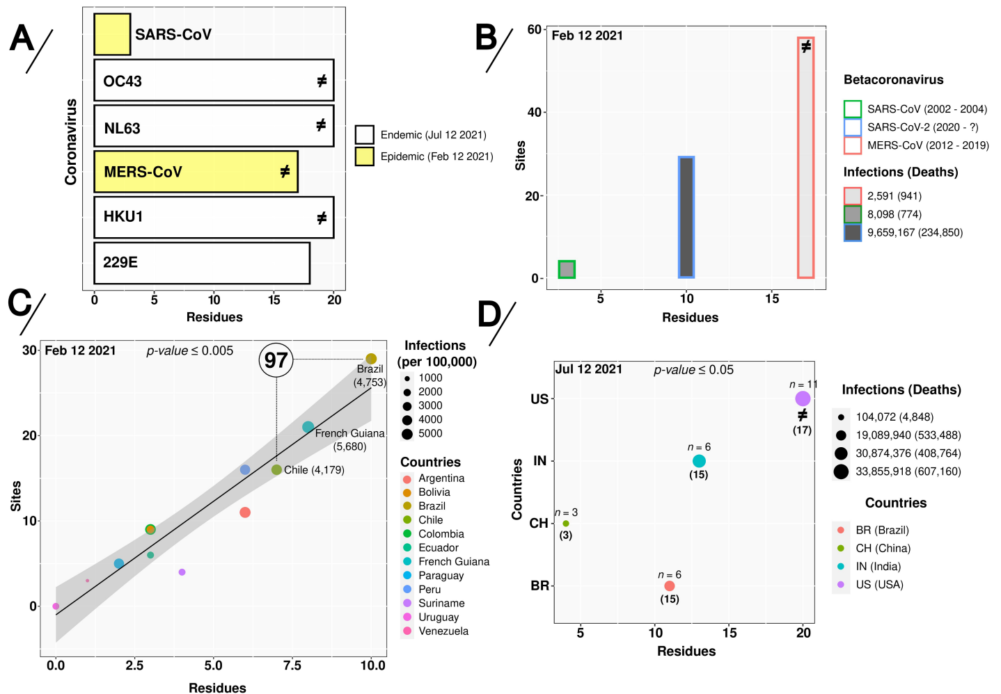
Figure 1. Directionally-evolving sites and residues in alpha- (229E and NL63) and beta- (OC43, HKU1, SARS-CoV, MERS-CoV and SARS-CoV-2) coronavirus sequences. (A) Directed-evolving residues in six different endemic and epidemic human coronaviruses (HCoVs), (B) Sites and residues vs infections in epidemic and pandemic coronaviruses (CoVs). (C) Linear-regression curve and co-relationship on the absolute amount of sites and/or residues under directional-positive selection given SARS-CoV-2 infections per 100,000 people from South America countries and (D) the total number of SARS-CoV-2 infections in Brazil, China, India and the USA. In panels A and B, the symbol \neq represents the presence of recombination breakpoints signals. In panel C, the number inside the circle represents the amount
