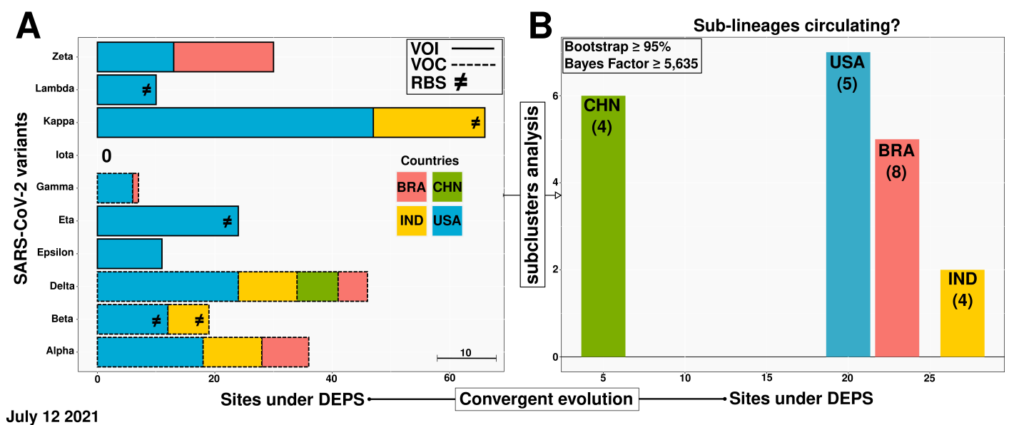
Figure 2. Transmission clustering and sub-clustering analyses on SARS-CoV-2 Variants of Concern (VOC) and Variants of Interest (VOI) sequences. (A) Model-based phylogenetic Maximum Likelihood (ML) method to infer transmission clustering and directional evolution in the VOC (dashed line) and VOI (non dashed line), and (B) sub-clustering and sub-lineage inferences in strains circulating in Brazil, China, India and the USA. Each color represents a particular country. RBS stands for recombination breakpoints signal (≠) and the scale bar shows the proportion of ten sites under positive selection (A). The numbers in parentheses indicate Spike-encoding protein sites under directional and convergent evolution (B).
