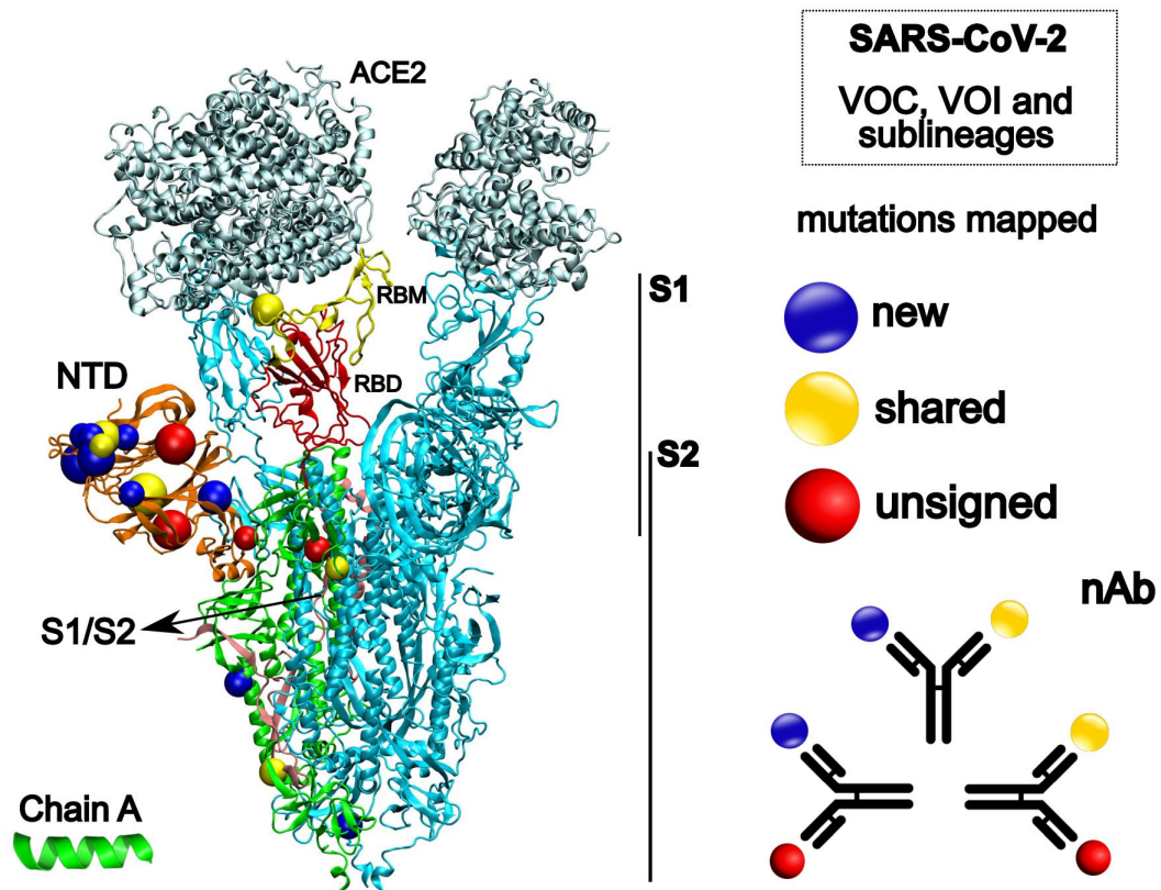
Figure 3. Structural representation of the SARS-CoV-2 Spike glycoprotein (PDB 7A98). On the left side, different colors represent ACE2, angiotensin-converting enzyme 2 (silver); NTD, N-terminal domain (orange); RBM, receptor binding motif (yellow); RBD, receptor binding domain (red) and S1/S2, cleavage site to S2 (pink). The structures in blue represent the chain B and C, respectively. Coloured spheres highlight the mutations mapped in the study. On the right side, our hypotheses about a linear perspective into the prospective vaccine efficacy against different SARS-CoV-2 strains. nAb, neutralizing antibody. Spike protein image was created with the Visual Molecular Dynamics (VMD) v.1.9.3 (Humphrey, Dalke, and Schulten1996).
