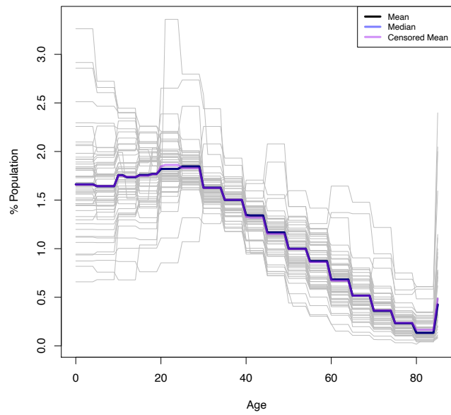
Figure 2. Various estimates of baseline age distribution (mean, median, and censored mean) plotted on age distribution for observed locations in gray.
