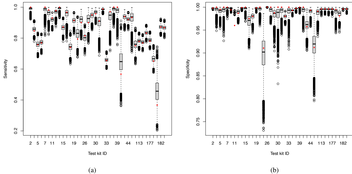
Figure 1. Boxplots showing the posterior distribution of the (a) sensitivity and (b) specificity for each test kit. Raw sensitivity/specificity based on the lab validation data is shown by a red point for each test kit.
