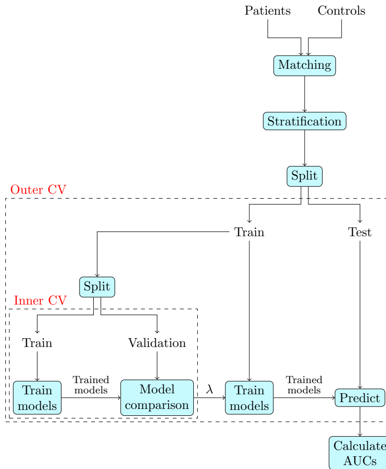
Supplementary Figure 5: The nested cross-validation (CV) scheme used for the clinical predictors. The outer CV ensures that the predictions used for the AUC calculations are on unseen data, while the inner loop optimizes the l_1 -penalty parameter \lambda . On each level the data was split into 5 stratified folds, and the same folds were used across the three different LASSO models.
