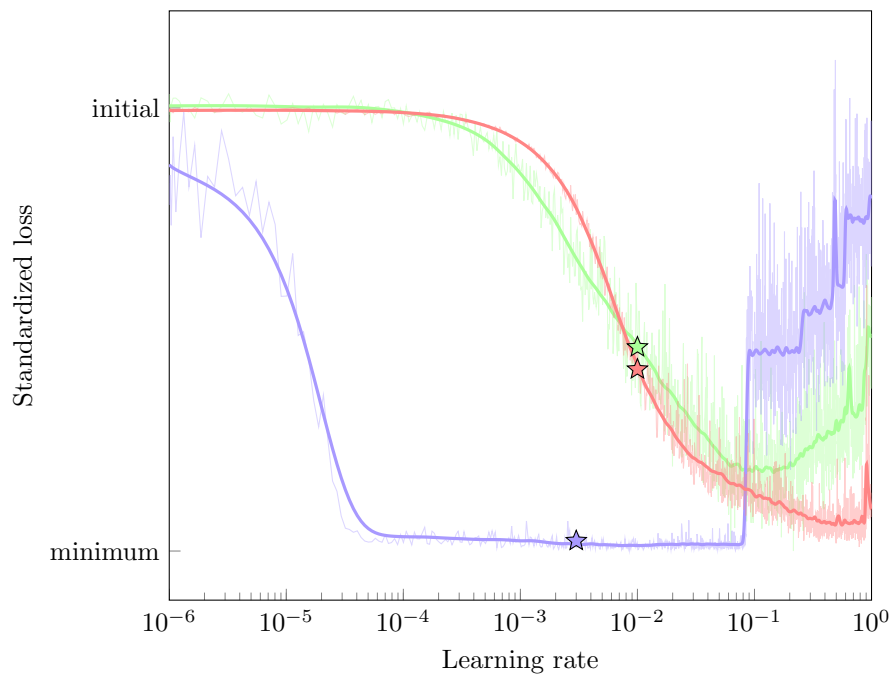
Supplementary Figure 7: Results of the learning rate sweep for the three model variants. The sweep investigated the models ability to learn at different learning rates, indicated by a step descent. The initial learning rates, denoted by the stars, were set manually based on this visualization.
