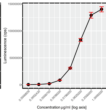
anti-IgG#5-HRP 0.09 mg/ml
