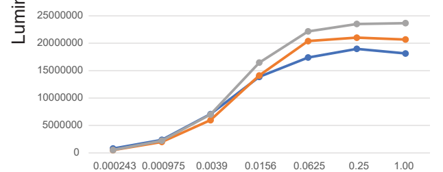
RBD antigen
