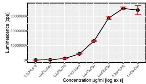
anti-IgG#5-HRP 0.18 mg/ml
