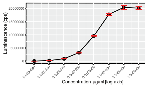
anti-IgG#5-HRP 0.09 mg/ml
