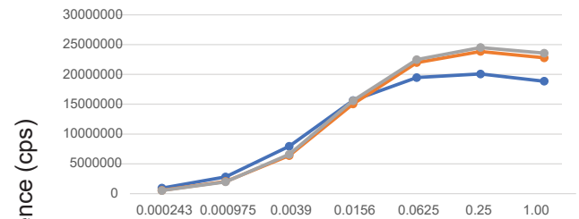
RBD antigen
