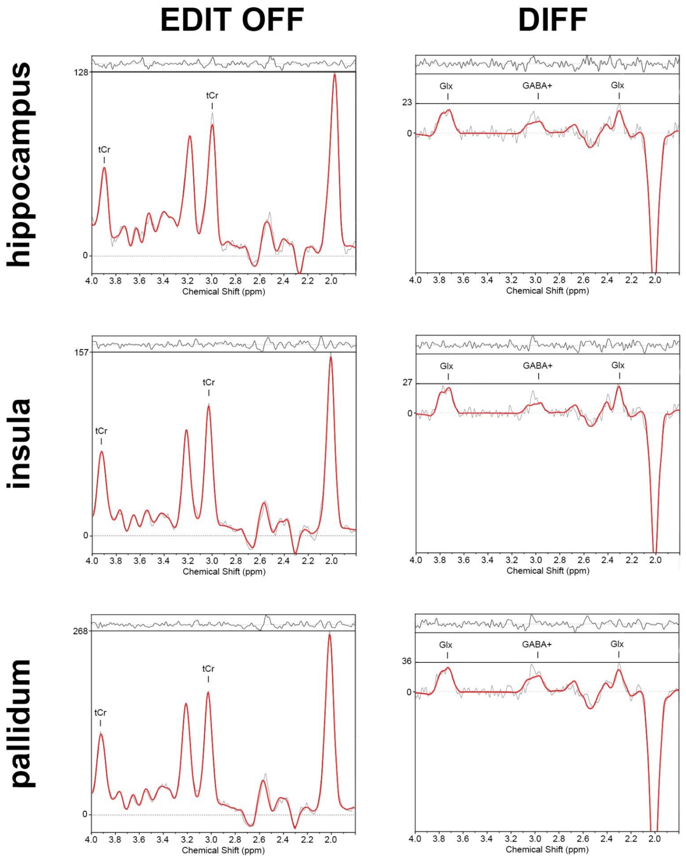
Supplement figure 1: LCMoel fits of exemplary non-edited (EDIT OFF) and difference spectra (DIFF) of the hippocampus, insula and pallidum.
