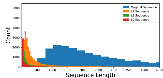
Figure 3. Histograms of sequence lengths of the original intervention sequence and Hi-RISE's L0, L1, and L2 sequence representations.
