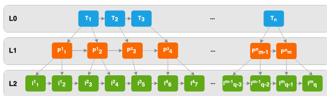
Figure 1. Illustration of Hi-RISE ( Hierarchical Representation of Intervention Sequences ). L0 represents the sequence of provider types ( T_1 \dots T_n ), L1 represents the sequences of actual provider encounters ( P_1^1 \dots P_m^m ), and L2 represents sequences of interventions ( I_1^1 \dots I_q^m ).
