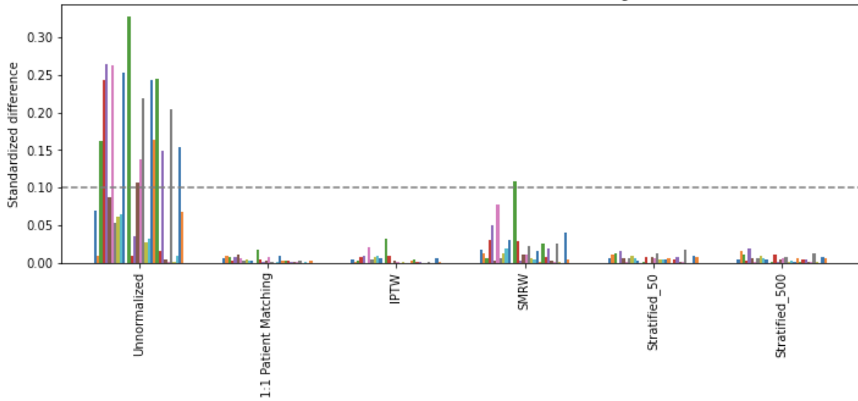
Feature standardized differences for different matching methods
