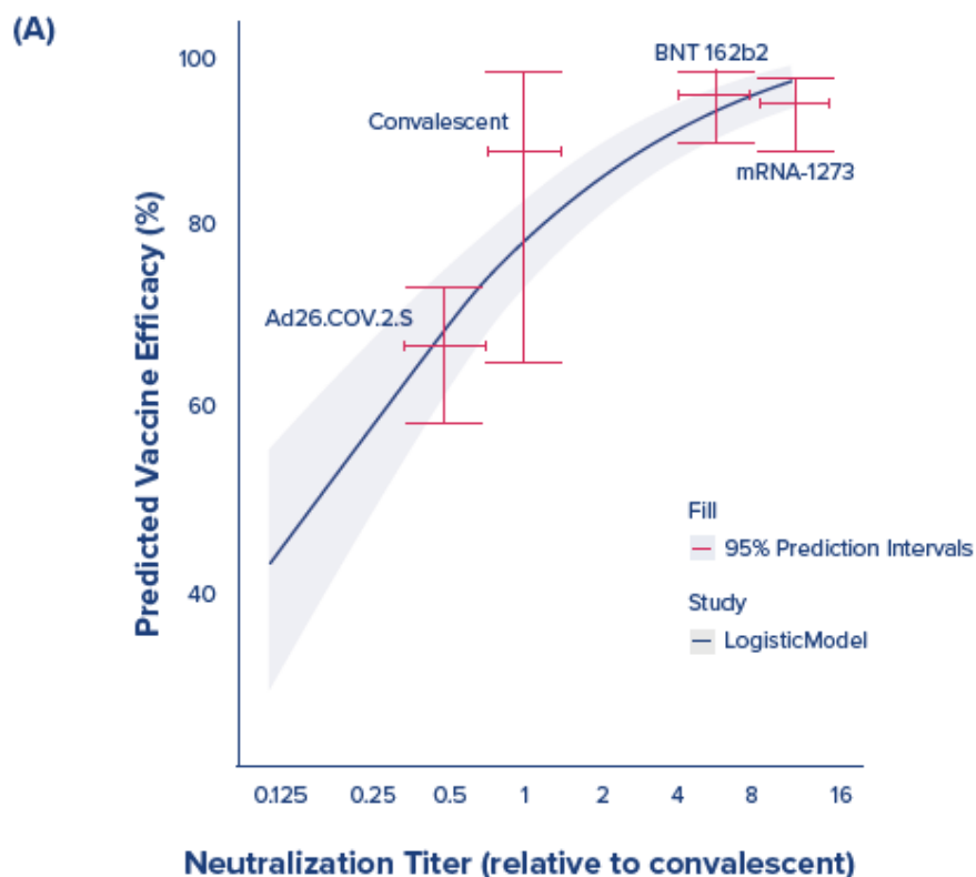
Figure 1: Vaccine Efficacy Against Symptomatic Infection is based on the logistic model developed by Khoury et al using calibration to mean NAb titer measured for Moderna, Pfizer, J&J and convalescent (former positive) subjects.
