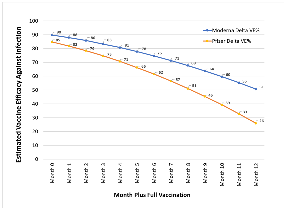
Figure 4: IAT VE Decay Model Estimated vaccine efficacy (VE) against symptomatic infection from the Delta variants of SARS-CoV-2 versus months post-full vaccination for Moderna and Pfizer vaccines.
