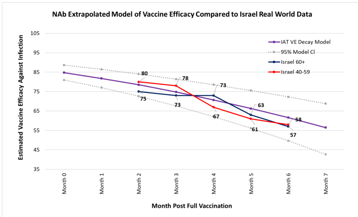
Figure 5. Estimated VE from the IAT VE Decay Model assuming Pfizer vaccination and protection from WT SARS-CoV-2 compared to reported VE from Israel. Dashed lines show 95% CI for the IAT VE Decay Model values.
