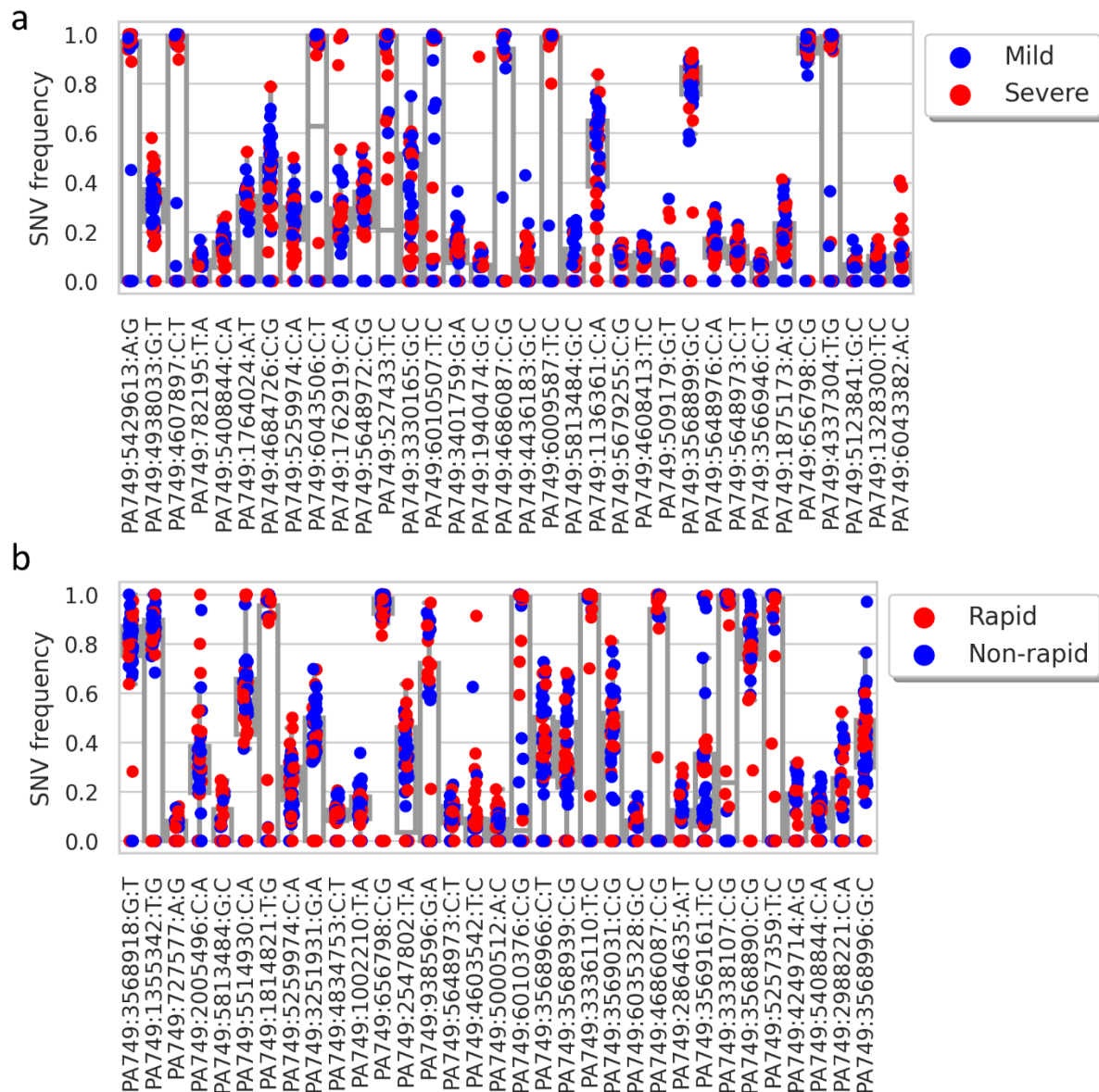
Supplementary Figure 1. Distribution of predictor SNV frequencies.
