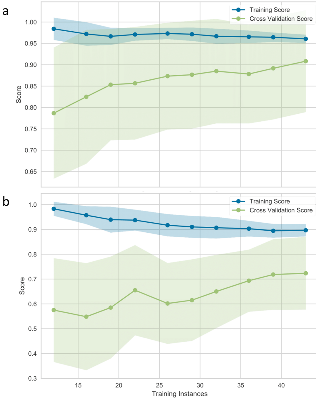
Supplementary Figure 5. Learning curve of logistic regression models for prediction of lung disease severity and progression.
