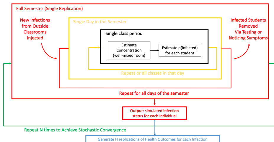
Fig 1. Overview of simulation model.
