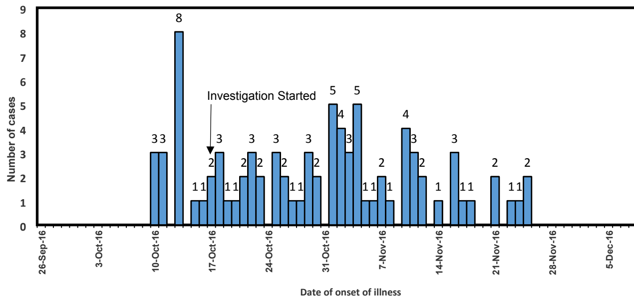
Figure 1: Epi curve – No. of cases by the date of onset of illness, union council Sohan Islamabad October-November 2019
