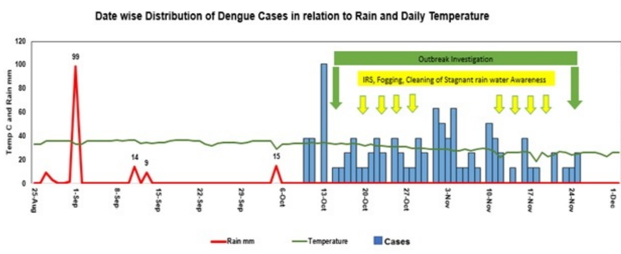
Figure 2: Epi curve with information on rain and temperature plots union council Sohan Islamabad October-November 2019
