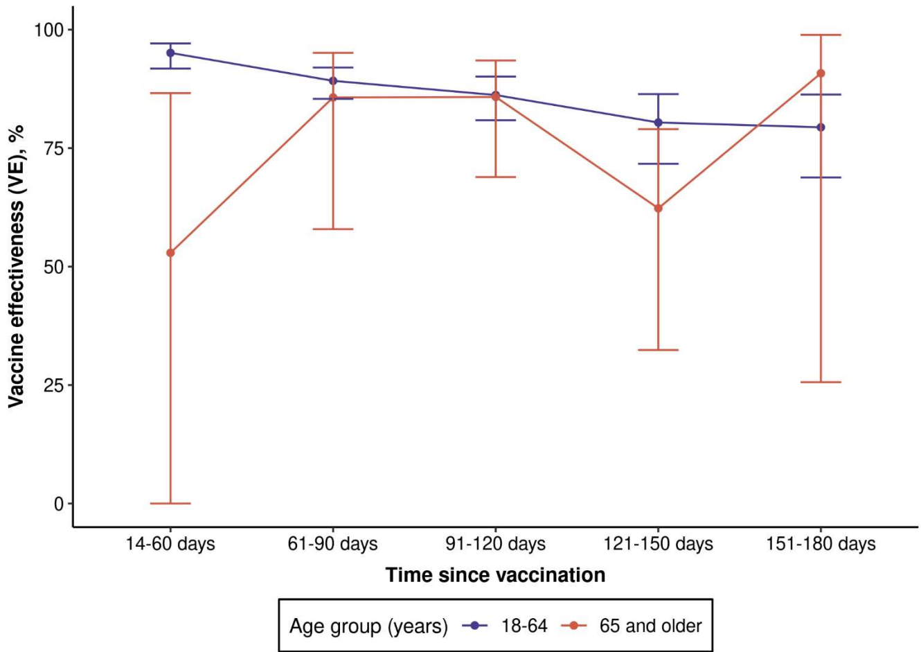
Figure S3. Vaccine effectiveness of 2 doses of mRNA-1273 against Delta infection by time since vaccination and age group
