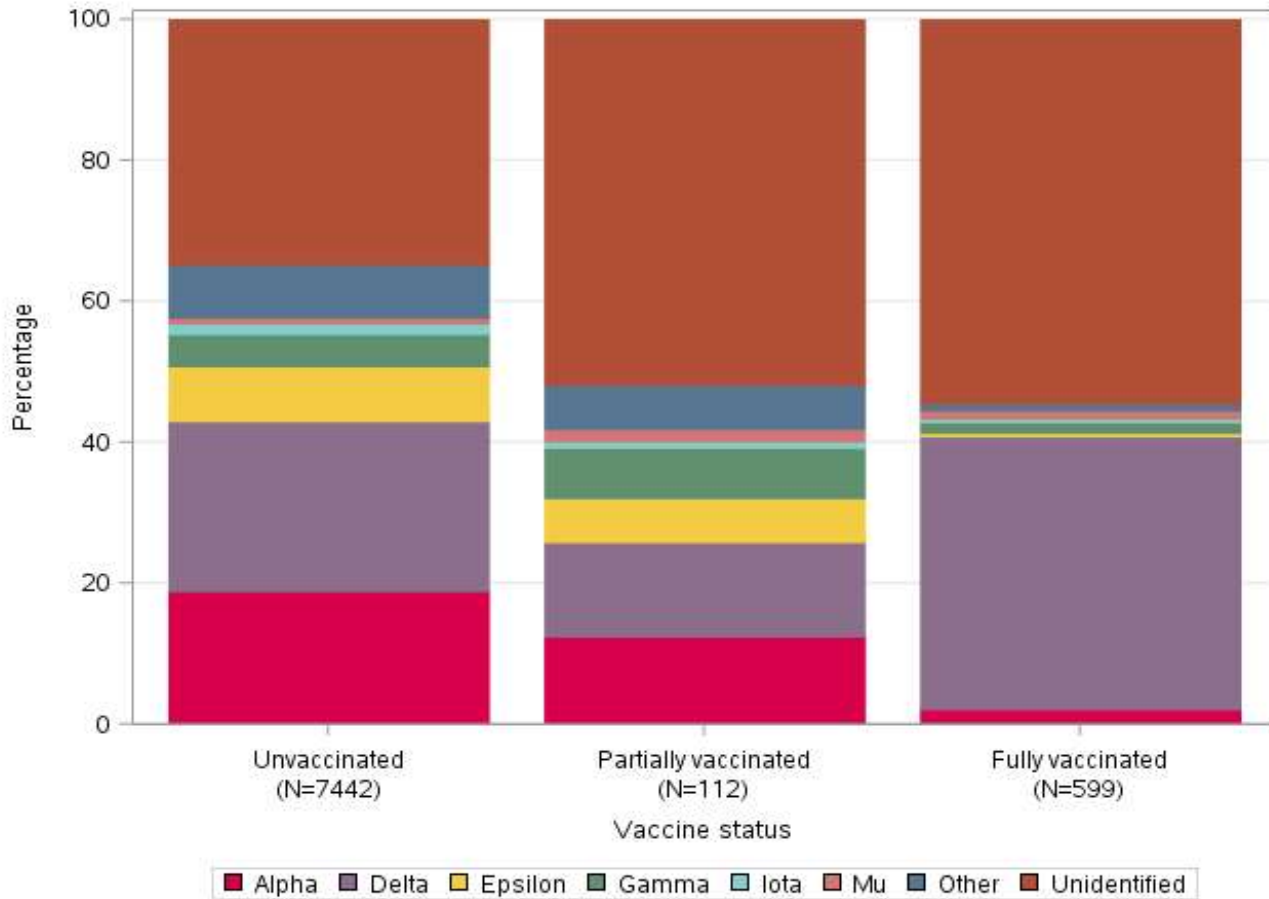
Figure S1. Distribution of SARS-CoV-2 variants by mRNA-1273 vaccination status
