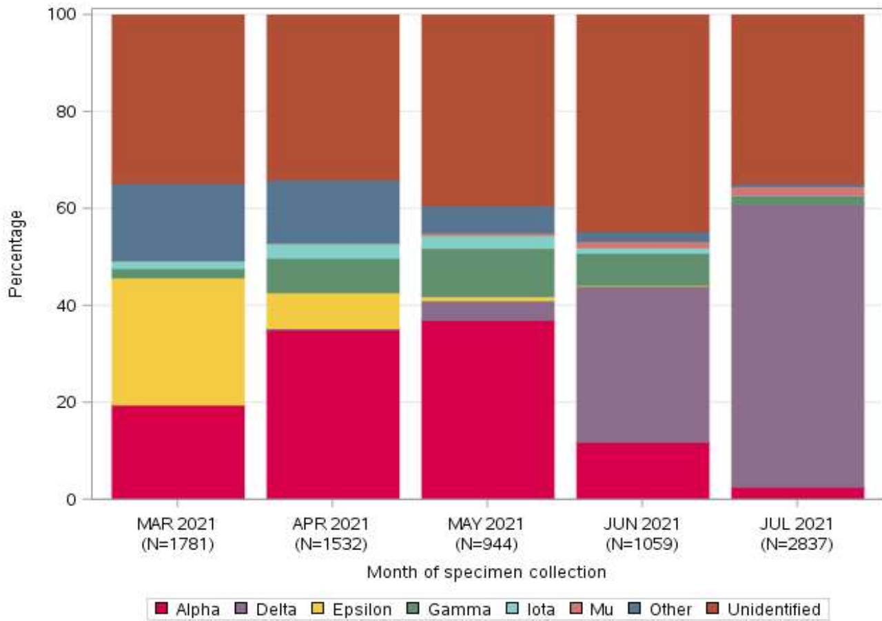
Figure S2. Distribution of SARS-CoV-2 variants by month of specimen collection
