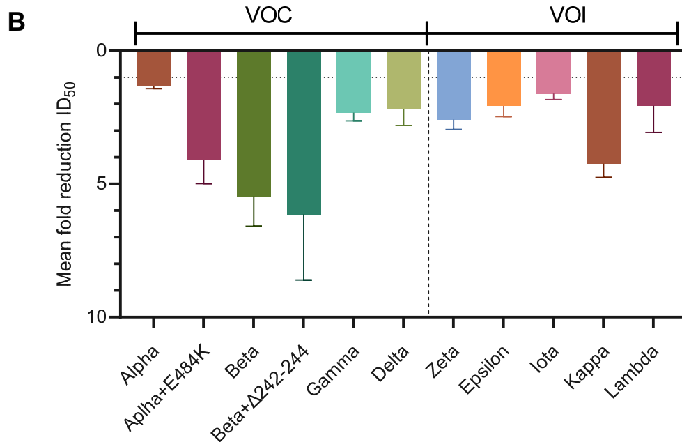
Figure S3: Binding and neutralization titers post-vaccination against VOCs and VOIs. (A) Median binding MFI of wild-type and VOCs plotted against the reported vaccine efficacy against symptomatic infection (REFS). Vaccine groups are indicated by colors with BNT162b2 in green, mRNA-1273 in purple, AZD1222 in orange and Ad26.COV2.S in blue. Circles represent WT data, squares for Alpha, nabla triangle for Gamma and delta triangle for Delta. Spearman's rank correlation coefficient with p value are indicated. The poor (10%) efficacy of AZD1222 against the Beta variant in the phase 3 trial conducted in South-Africa was not included (REF). MFI, mean fluorescence intensity. (B) Mean \pm SEM fold reductions in ID 50 titers for the serum pools combined against the VOCs and VOIs pseudoviruses in comparison to ID 50 titers against D614G pseudovirus.
