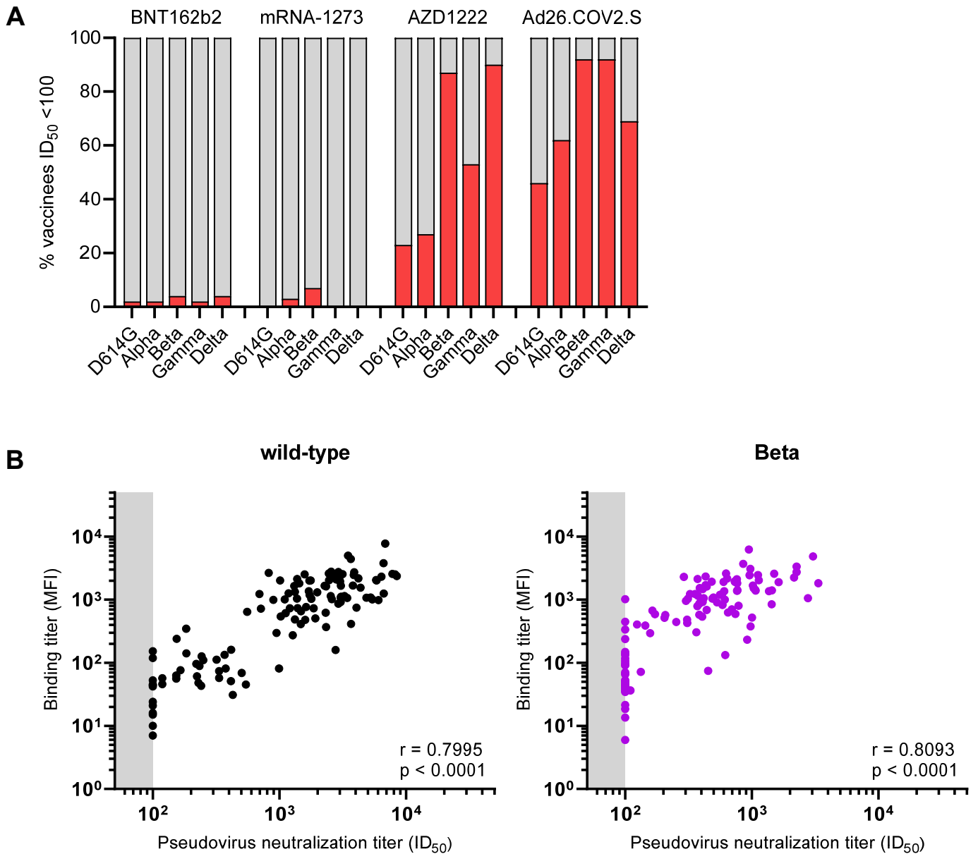
Figure S2: Binding and neutralization against VOCs. (A) Percentage of individuals (in red) in each of the vaccine groups that have no detectable serum neutralizing activity ( ID_{50} < 100 ) against the indicated pseudoviruses. (B) Correlation between wild-type and Beta binding (MFI) and neutralization titers ( ID_{50} ). Spearman's rank correlation coefficient with p value are indicated.
