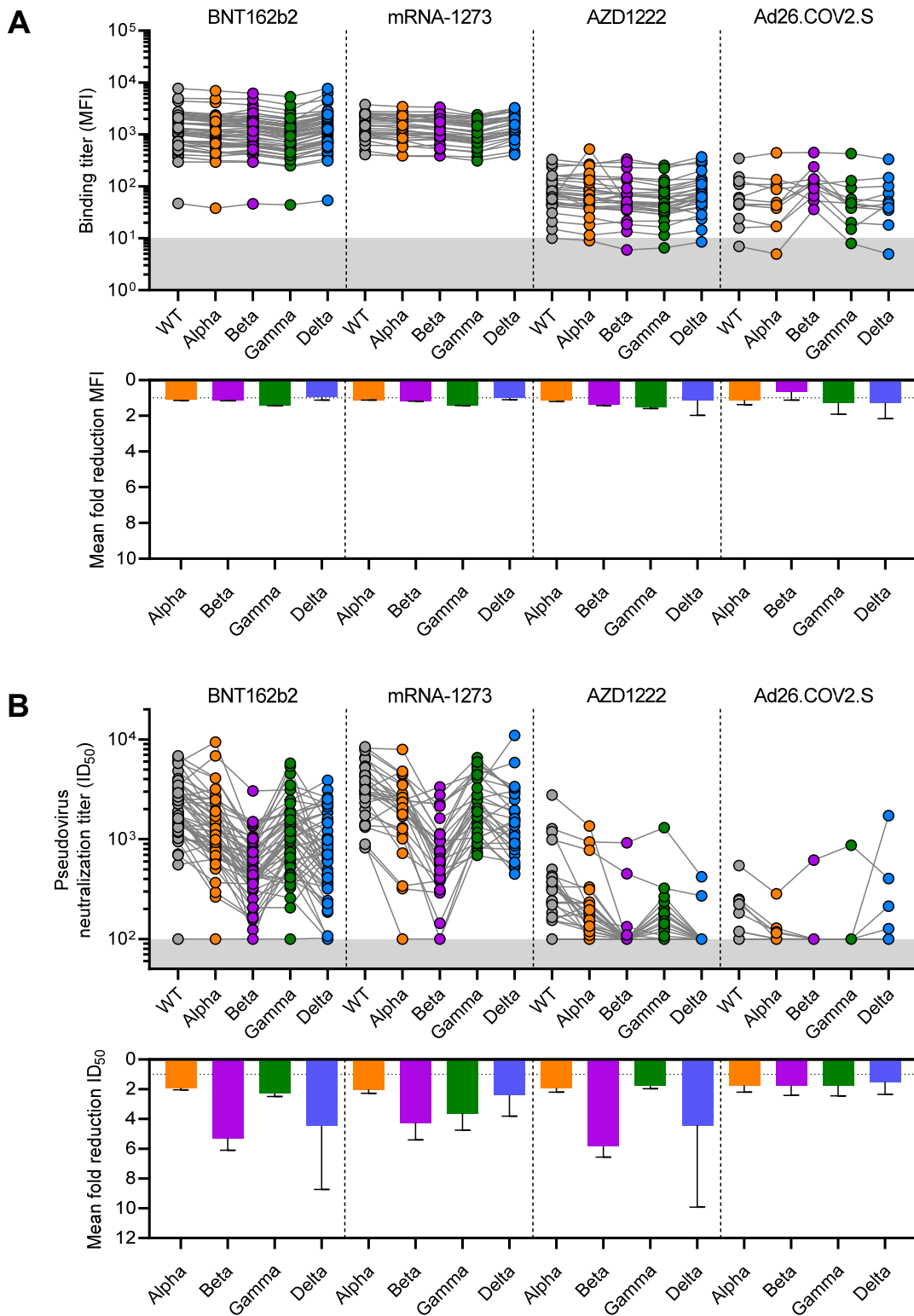
Figure S1: Binding and neutralization titers post-vaccination against the VOCs. (A) Paired binding titers to wild-type and VOCs S protein represented as mean fluorescence intensity (MFI) of 1:100,000 diluted sera collected post full vaccination for the four vaccination groups (upper plot). The lower cutoff for binding was set at an MFI of 10 (grey shading). Mean \pm SEM fold reductions in binding MFI against the VOCs in comparison to wild-type (lower plot). (B) Paired half-maximal neutralization ( ID_{50} ) titers of D614G and VOCs pseudoviruses for sera collected post full vaccination for the four vaccination groups (upper plot). Mean \pm SEM fold reductions in ID_{50} titers against the VOCs pseudoviruses in comparison to ID_{50} titers against D614G pseudovirus.
