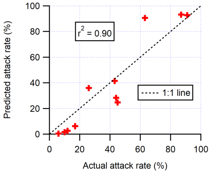
134 Figure S1: Attack rates of the COVID-19 outbreaks shown in Table 1 predicted according to the 135 fitted trend line in Figure 2b vs. actual attack rates of those outbreaks. The correlation 136 coefficient between the two types of attack rates and the 1:1 line are also shown.
