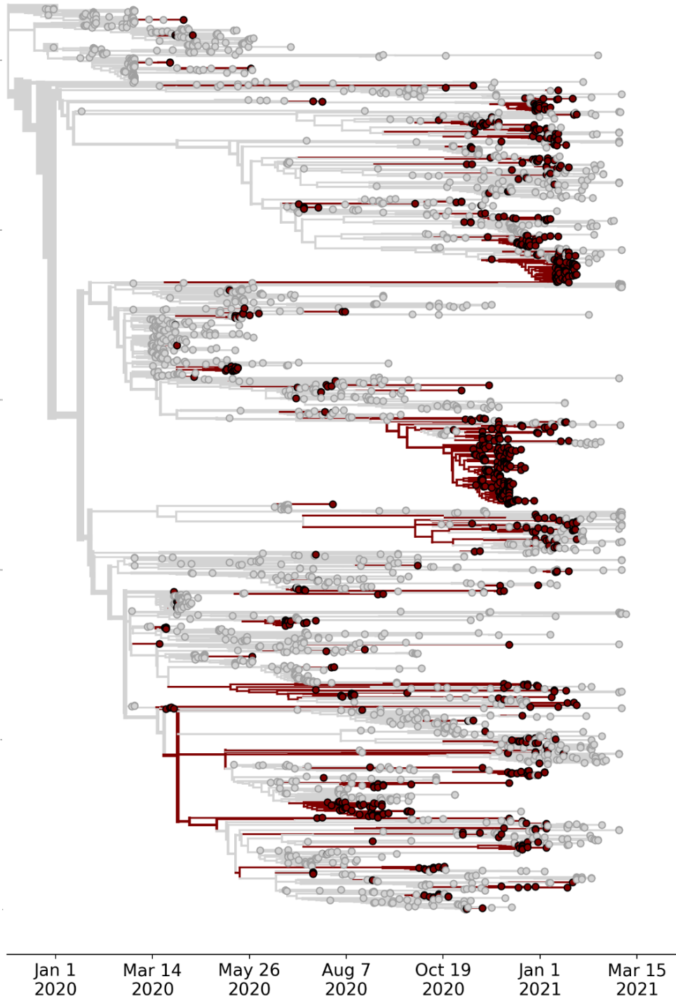
Supplemental Figure 2: Temporally-resolved phylogenetic tree of 2653 SARS-CoV-2 genomes, 853 of which were sampled from Humboldt County. Tips sampled from Humboldt County are indicated in maroon and tips sampled from other locations are colored in grey. Branches colored in maroon indicate inferred circulation within Humboldt County, and branches in grey indicate inferred transmission outside of Humboldt County.
