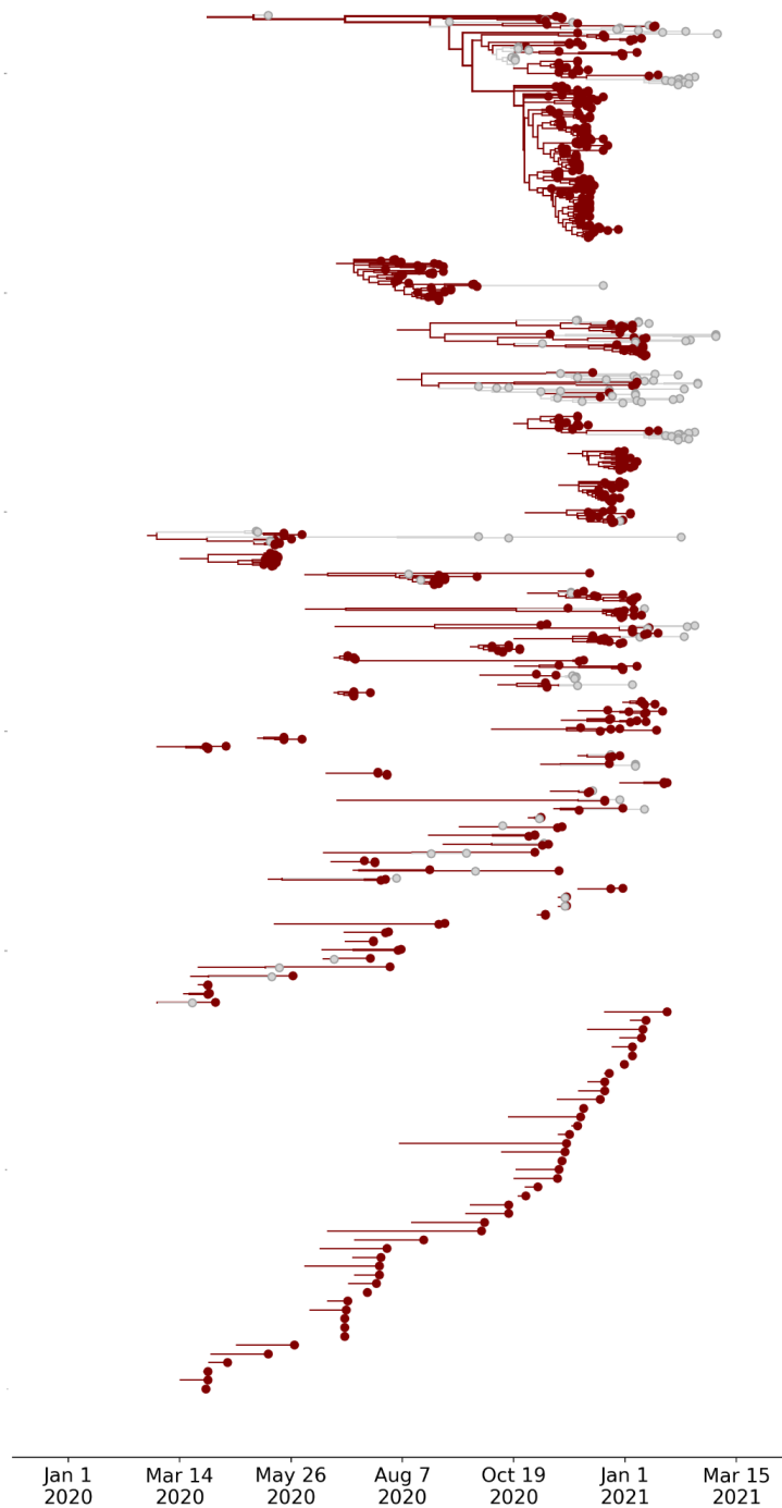
Supplemental Figure 1: Phylogenetic clades for 100 discrete lineages of SARS-CoV-2 introduced to Humboldt County. Each clade represents a unique introduction of the virus to the county, and the length of maroon branches indicate transmission duration within Humboldt County. Grey tips and branches represent descendents of that lineage that circulated outside of Humboldt County. Most introductions lead to limited transmission within Humboldt County, as evidenced by minimal genetic diversity of a clade sampled within the county.
