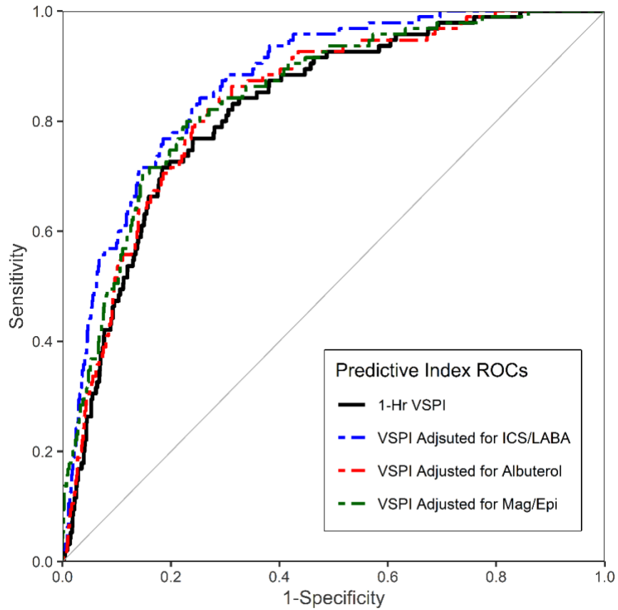
Supplemental Figure 1. Receiver-Operator Curves (ROC) of the predictive index using demographics and 1st hour vital signs to predict PICU admission (black), compared to the ROCs of the same vital signs predictive index (VSPI) adjusted for ICS/LABA use while inpatient (blue), albuterol administration in the ED (red), magnesium or epinephrine administration in the ED (green).
