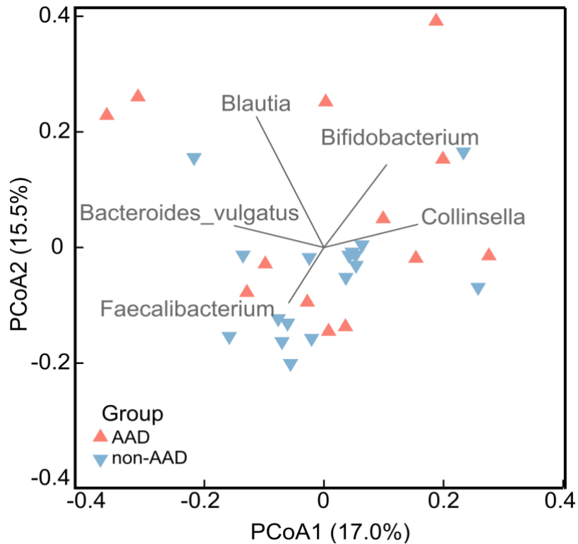
Figure S2. PCoA of baseline samples based on the ASV level bray-curtis dissimilarity.
