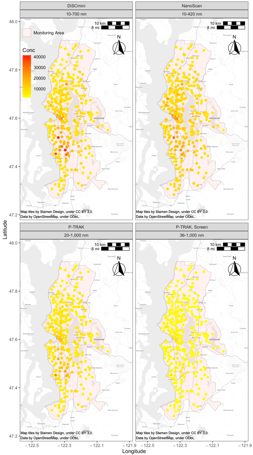
Figure S16. Annual average total UFP concentrations at monitoring sites ( N=309 ) for different UFP measures.
