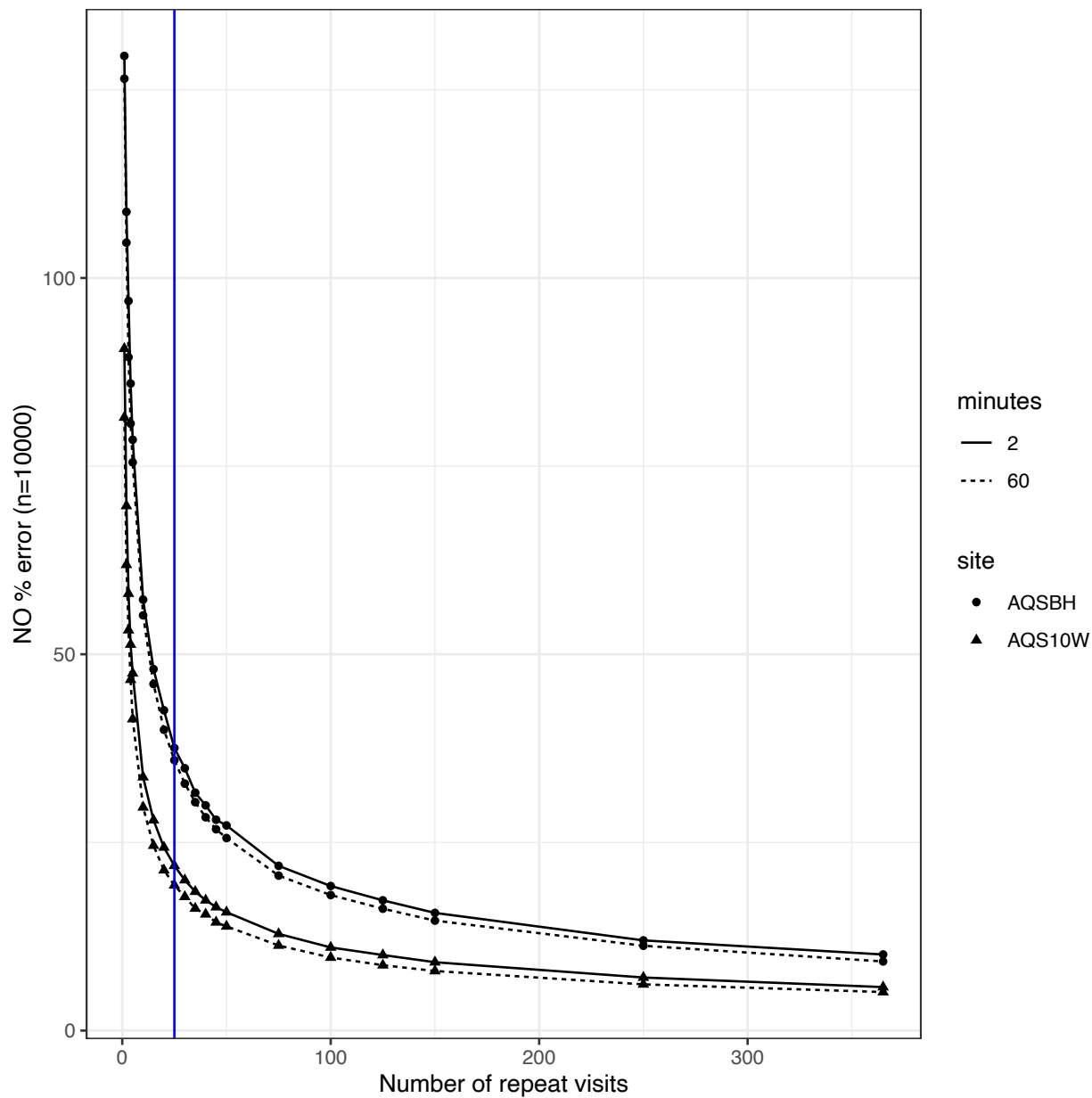
Figure S2. Mean percent error (\text{estimated\_conc} - \text{true\_conc}) / \text{true\_conc} * 100 in the estimated nitrogen monoxide (NO) annual average at the 10 th & Weller (AQS10W; near-road site) and Beacon Hill (AQSBH; background site) regulatory sites from repeated short-term random samples (2- and 60-min), when compared to the “true” annual average estimated from all the available 2019 data. Estimates are for 10,000 simulations of random sampling without replacement. The blue vertical line is for 25 repeat visits.
