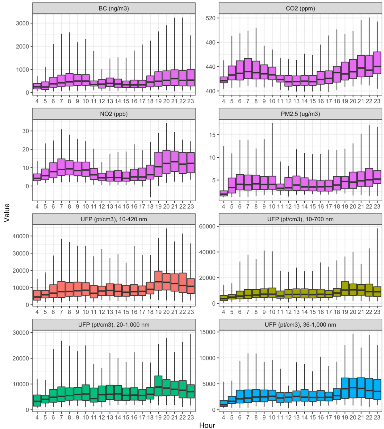
Figure S12. Median site visit concentrations by hour of the day. Lines connect median concentrations. Boxes show the 25 th , 50 th and 75 th quantile; whiskers show the 5 th and 95 th quantiles.
