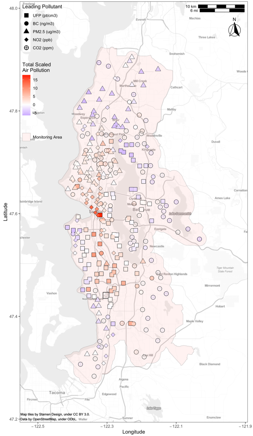
Figure S17. Annual average total scaled air pollution, defined at each site as: \text{Sum of scores} = \sum_{i=1}^n (x_{i,j} - \text{median}(X_i)) / \text{IQR}(X_i) , Where X is each individual pollutant ( n=5 ) and j indexes each individual pollutant measurement. Colors indicate where air pollution levels were higher or lower than the overall average (total scaled air pollution = 0). Shapes indicate the leading pollutant (highest score) at each site. UFP levels are for particles 20-1,000 nm (P-TRAK).
