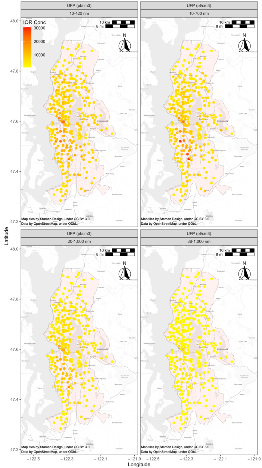
Figure S9. Interquartile range (IQR) of site of visit concentrations (N~29 visits per site) for UFP measures with different instruments and particle size ranges (nm).
