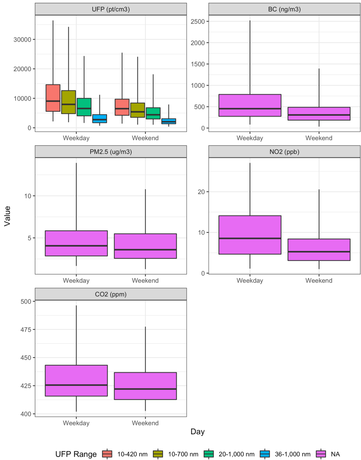
Figure S11. Median site visit concentrations by day of the week. Lines connect median concentrations. Boxes show the 25 th , 50 th and 75 th quantile; whiskers show the 5 th and 95 th quantiles.
