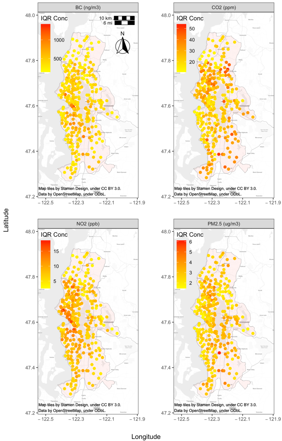
Figure S8. Interquartile range (IQR) of site visit concentrations for BC, CO 2 , NO 2 and PM 2.5 (N~29 visits per site).
