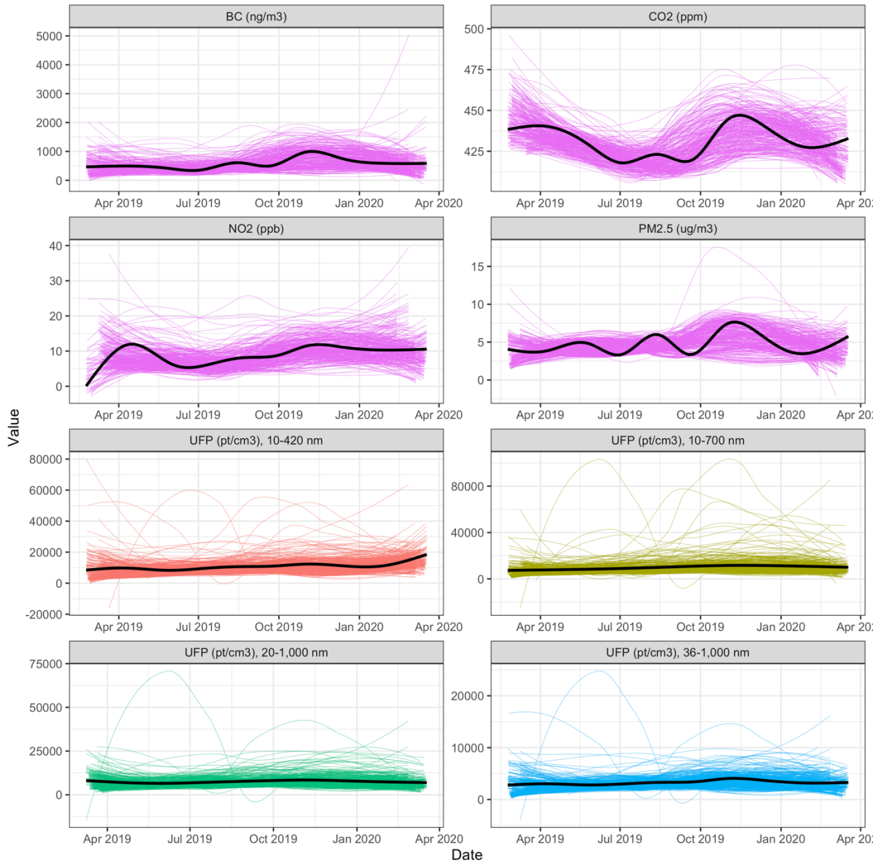
Figure S13. Site-specific pollutant concentrations over the course of the study. Thin lines show site-specific smooth (loess) fits for median visit concentrations ( N \sim 29 visits/site). Black lines show the overall smooth trends for all of the sites.
