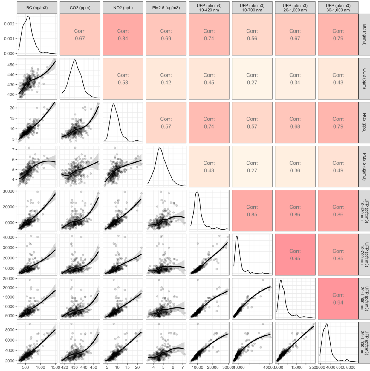
Figure S15. Annual average pollutant correlations ( N=309 sites). Lower panels show scatterplots with loess lines and 95% confidence intervals; upper panels show Pearson correlations ( R ), with higher values in darker reds; diagonal panels show density plots.
