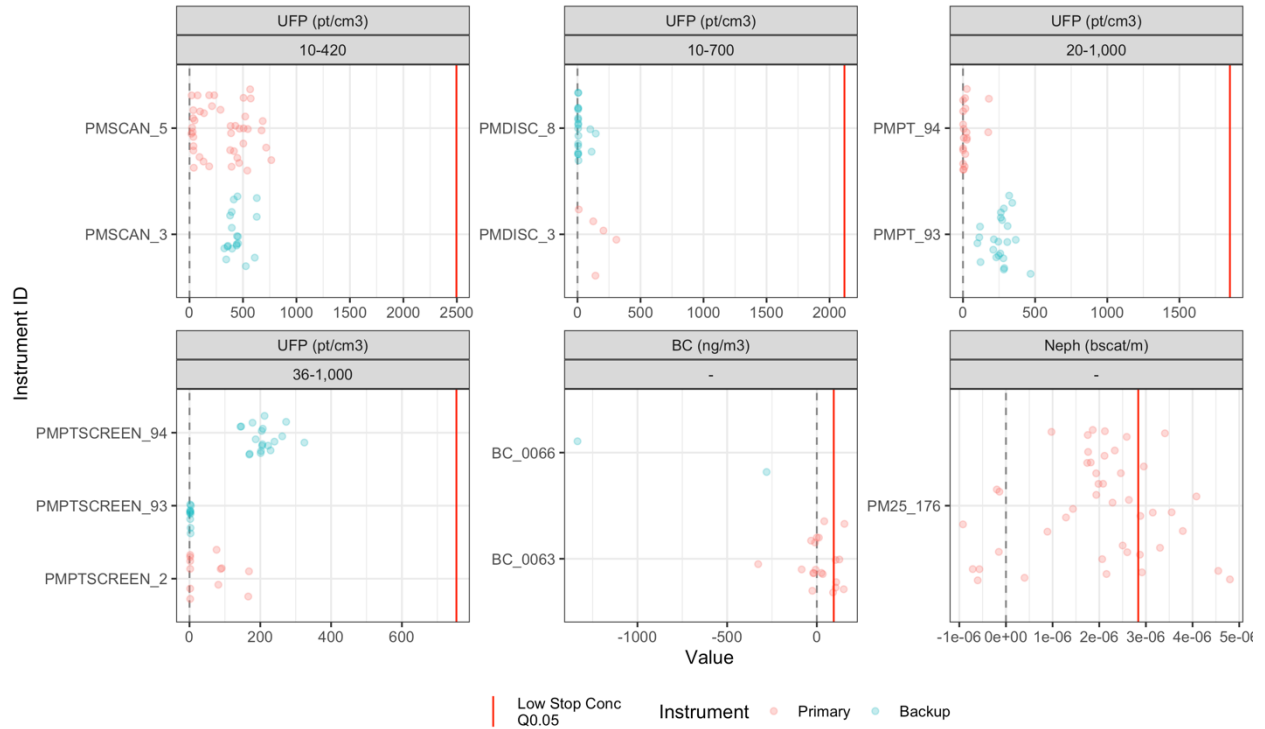
Figure S5. Particle instrument responses to filtered air (near 0 pt/cm 3 ). Dots show median, two-minute instrument readings. Red lines are “low” ambient concentration references, based on the 5 th quantile of stop concentrations for each pollutant. Responses for primary instruments are based on more instrument checks (data) throughout the study period.
