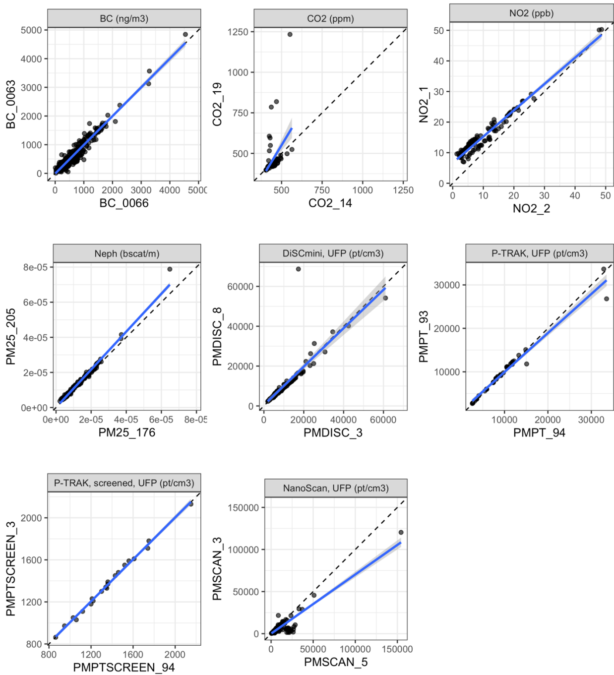
Figure S6. Comparison of two-minute median stop concentrations from instrument collocations. Gas values are post calibration. UFP instruments report number concentrations: particles (pt) per cm 3 .
