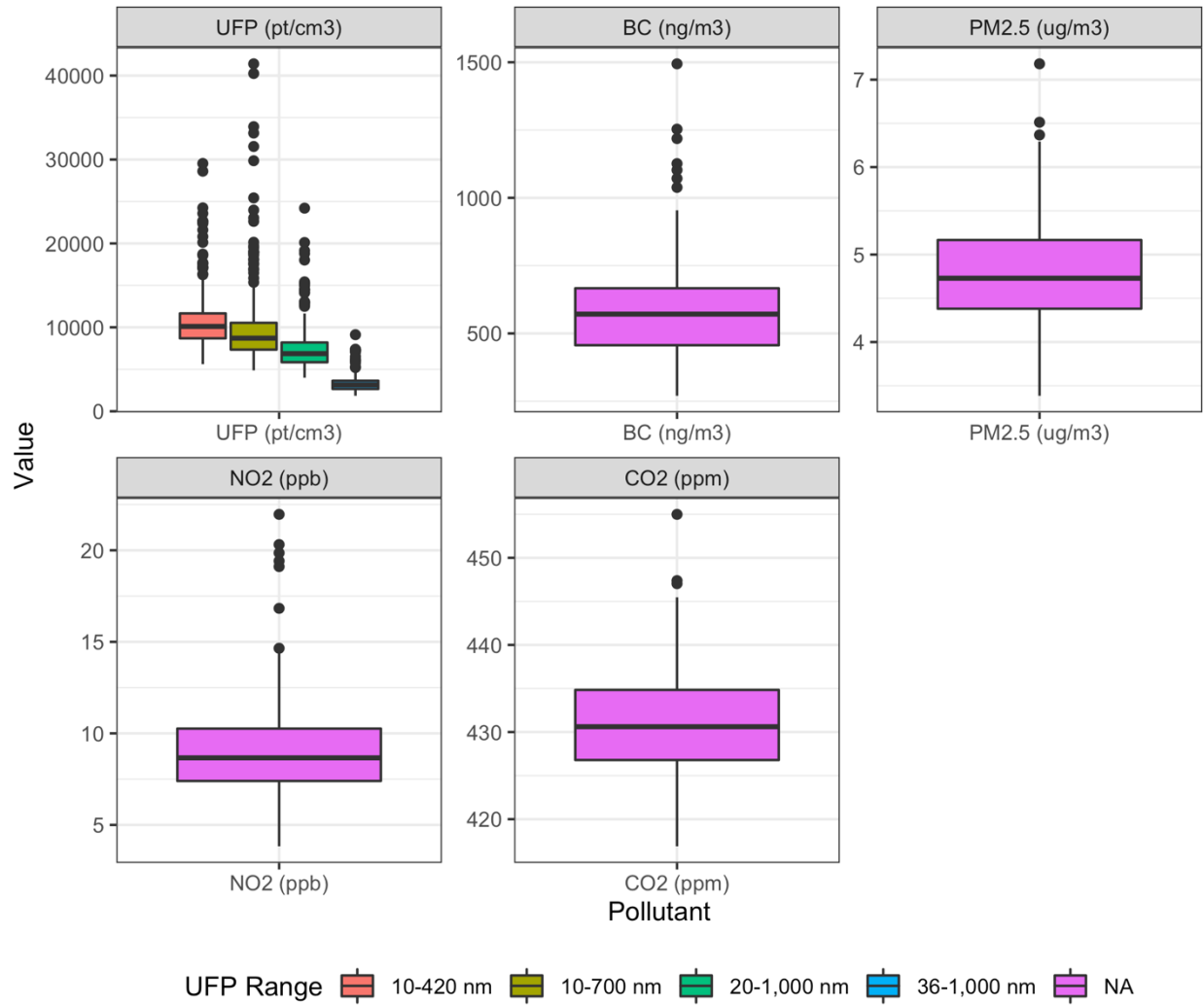
Figure S14. Annual average site concentrations (N=309). Boxplots are traditional and show all of the site averages such that boxes show the 25 th , 50 th and 75 th quantile (Q); whiskers show a 1.5*(Q75-Q25) distance away from the 25 th or 75 th quantile, and dots are outliers.
