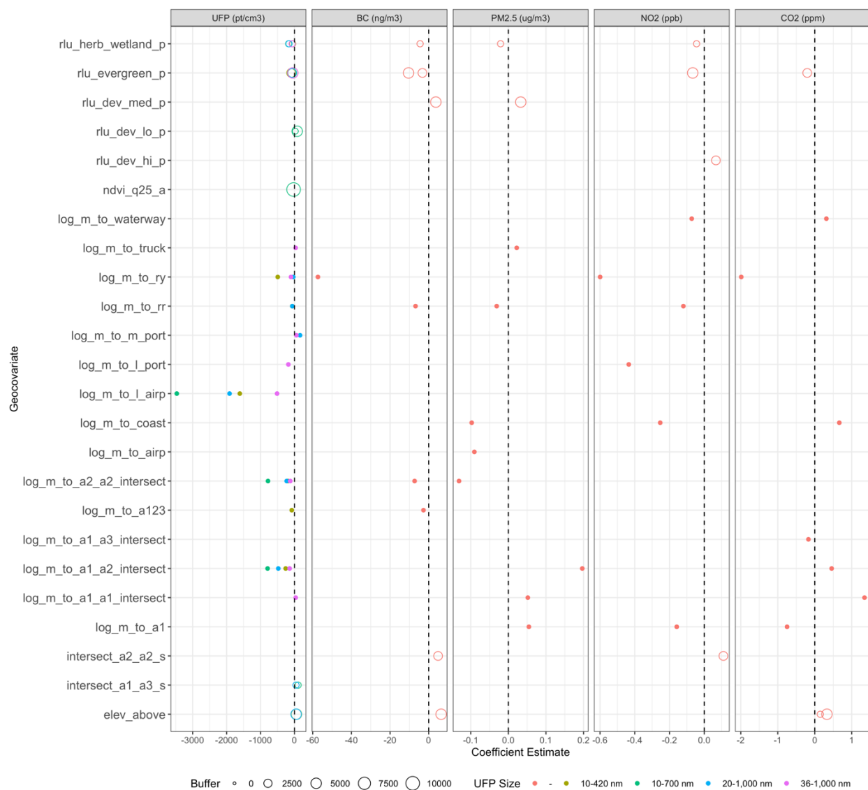
Figure S18. Lasso regression coefficient estimates for annual average pollutant concentrations. Covariates without buffer values (shown in the legend as “0” (m)) are for proximity and elevation variables rather than values for a buffered radius. Showing the top 10 covariates with the largest coefficient estimates for each pollutant. See SI Table S8 for covariate definitions.
