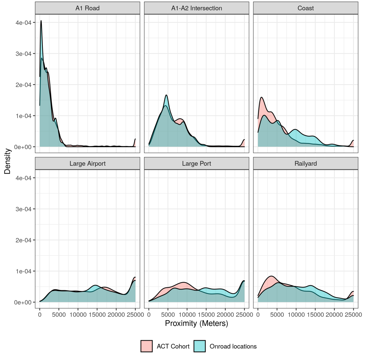
Figure S1. Covariate distributions of mobile monitoring road segments ( n=6,786 100 m segments) and ACT cohort locations ( n=10,330 ). Note that Figure 2 in the main text shows the distribution of stop monitoring locations rather than road segments.
