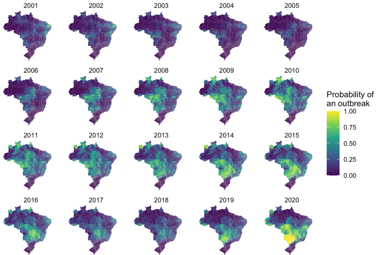
Fig S10: The probability of an outbreak estimated from the model for each year 2001 - 2020. The mean probability of an outbreak estimated by taking 1000 simulations from the posterior distribution of the response and transforming the outcome using a probit function
