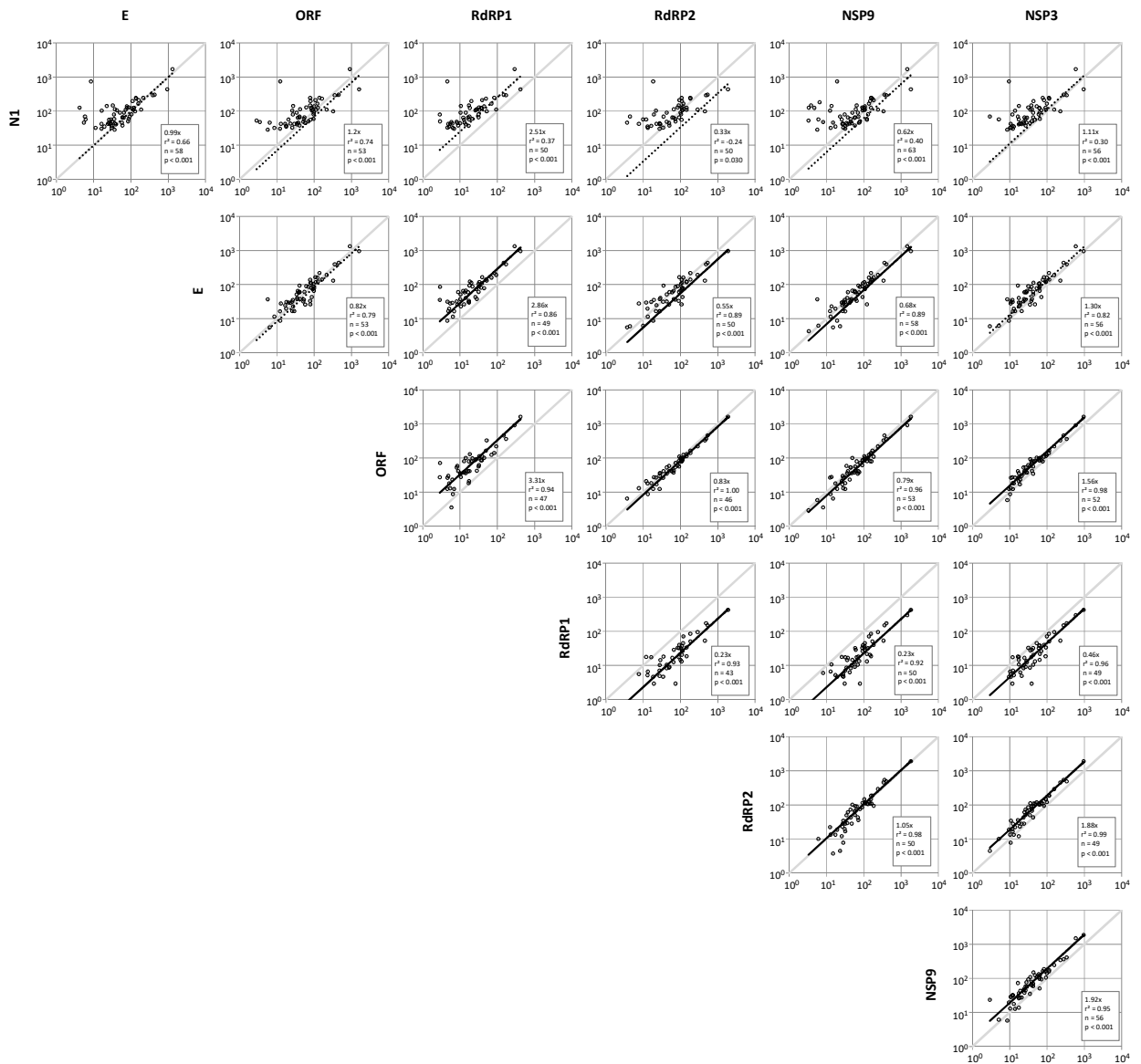
Fig. S3. Linear regressions of seven different primer/probe assays using a selection of 64 samples. Charts show gene copies per mL wastewater.
