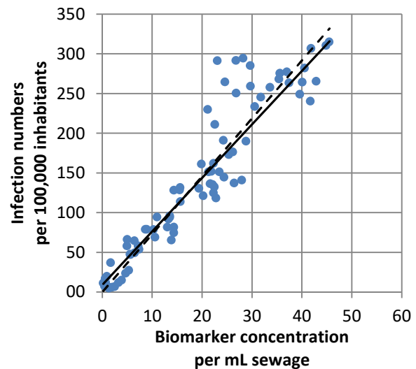
Fig. S2. Linear regression for infection data and ddPCR values (E and ORF gene as sliding average of three values). Left: original data, right: infection numbers were time-shifted by 16 days. Statistical analysis above each plot for each trend line with and without intercept. P values with Bonferroni-correction were below 0.001 for all correlations.
