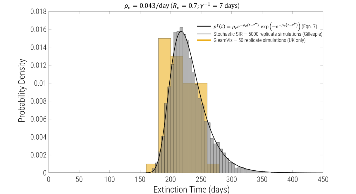
Figure 2: Probability density of extinction times for the same parameters as in Fig.1. Grey bars are a histogram of 5000 replicate simulations of Gillespie simulations normalised to give an estimate of the probability density, and the black curve is the prediction of the analytical calculation given in Eqn.7, which we see matches the simulations extremely well. The yellow bars are histograms from the GlemViz spatial epidemic simulator with 50 replicates, which we see gives similar results to the predictions of the stochastic SIR model.
