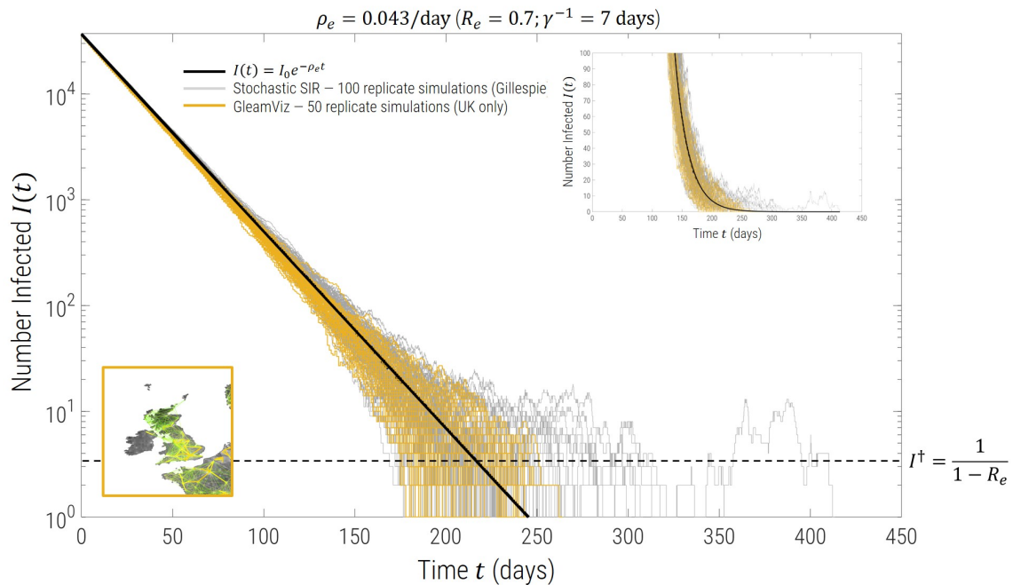
Figure 1: Simulation trajectories on log-linear scale (inset: linear-linear scale) for a decay rate of \rho_e = 0.043/\text{day} , corresponding to R_e = 0.7 , 1/\gamma = 7 days, I_0 = 3.7 \times 10^4 and an initial recovered population of R(0) = 6 \times 10^6 . The solid black line is the deterministic prediction from Eqn.5, grey trajectories are 100 replicate Gillespie simulations of a standard SIR model, whilst the yellow trajectories are from 50 replicates using the spatial epidemic simulator GleanViz (33, 34) restricted to the United Kingdom with a gravity model between heterogeneous sub-populations as shown in the inset map of the UK. The dashed black line is the threshold number of infected individuals I^\dagger , below which changes in infected number of individuals is mostly stochastic.
