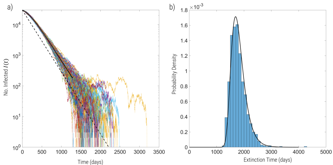
Figure 4: a) Trajectories of numbers infected I(t) for simulations with R_e = 0.99 > R_e^* for I_0 = 3 \times 10^4 , N = 67 \times 10^6 and assuming 10% of population recovered at time t = 0 , which gives R_e^* \approx 0.97 ; the solid line is the mean of the simulations, while the dashed line shows the decline of infections if R_e = R_e^\infty from t = 0 , where we see the slope is the same as the mean at longer times. b) Histogram of extinction time distributions of the same simulations with prediction given by Eqn7, but with R_e \rightarrow R_e^\infty and \tau^\dagger \rightarrow \tau^\dagger + 1/\rho_e^\infty , as detailed in the text.
