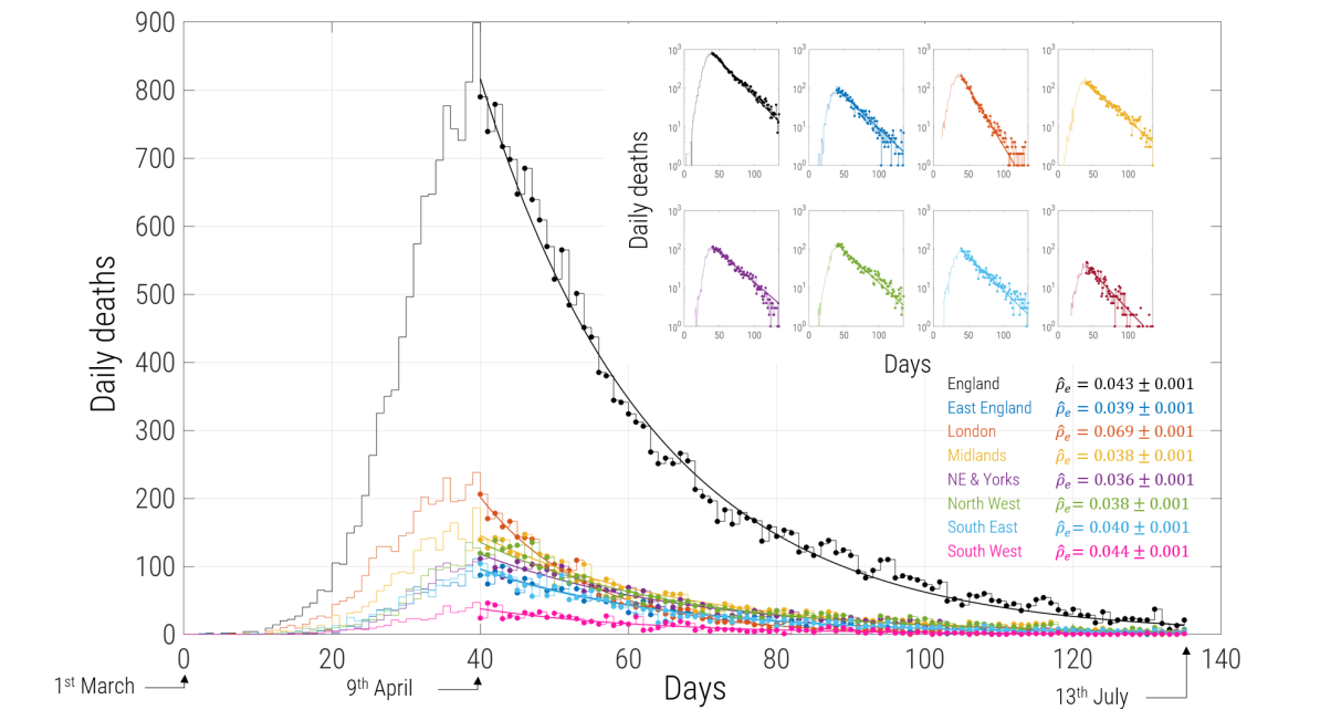
Figure S1: Data from NHS England (S1) on daily deaths within hospitals in England and different regions within England. Each region is fit using a simple decaying exponential from 40 days after the 1st March 2020, where each region first shows a clear decline in number of daily deaths.
