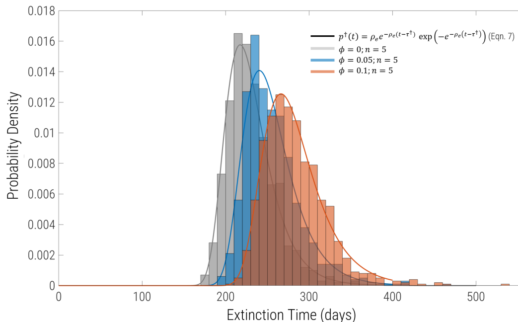
Figure 3: Probability density of extinction times for the same parameters as in Fig.1, but including migration and sub-division into equal sized populations. Each histogram comprises 1000 replicates for n = 5 regions connected by uniform migration with probability \phi . Grey bars are \phi = 0 (complete isolation), blue correspond to \phi = 0.05 and \phi = 0.1 are the red bars. For \phi = 0 the solid line grey line is exactly the solid black line in Fig.2, showing that the extinction time distribution of identical to the single global well-mixed population of same aggregate size. The solid blue and red lines are fits to the histogram using Eqn.7 with a single free parameter R_e (with \gamma and I_0 constrained to the values used to run the simulations).
