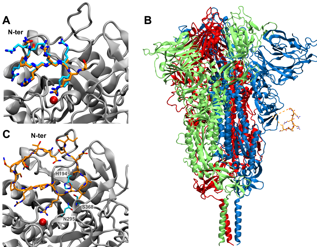
Figure S1 - (A) Structural motif 679-NSPRRARS-686 (orange, licorice representation) of protein S modeled based on an inhibitor (cyan, licorice representation) that was co-crystallized with the furin enzyme (silver, cartoon representation, \text{Ca}^{2+} ion in red) (PDB 6HLB). (B) The modeled 679-NSPRRARS-686 motif (orange, licorice representation) was aligned to the full-Spike homotrimer (chains A, B and C represented in cartoon colors in blue, red and green, respectively) and the remaining residues were modeled to close the loop. (C) Initial input used in calculations with the loop comprising native residues 675-QTQTNSPRRARSVASQSI-692 (orange, licorice representation) in the conformation of interaction with the furin enzyme (cartoon representation, silver). Active site residues His194, Ser368 and Asn295 are shown in licorice representation (nitrogen atoms in blue, carbon atoms in cyan and oxygen atoms in red) and \text{Ca}^{2+} ion is represented as a red sphere.
