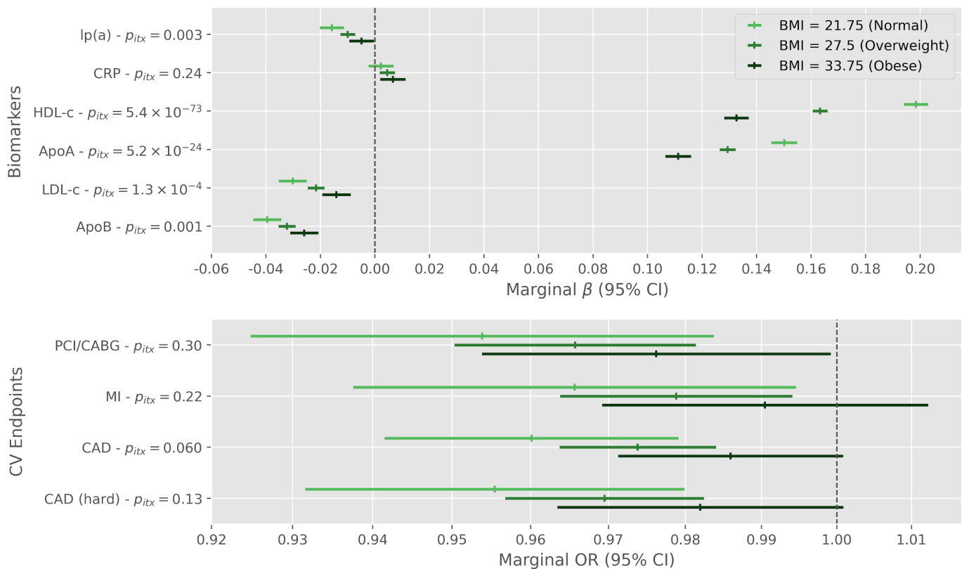
Figure 3. Effect modification by body mass index of a 1 standard deviation decrease in the CETP concentration genetic score on biomarkers and cardiovascular outcomes in the UK Biobank. Displayed p -values ( p_{itx} ) are for the two-sided test of the product term between the CETP score and standardized body mass index.
