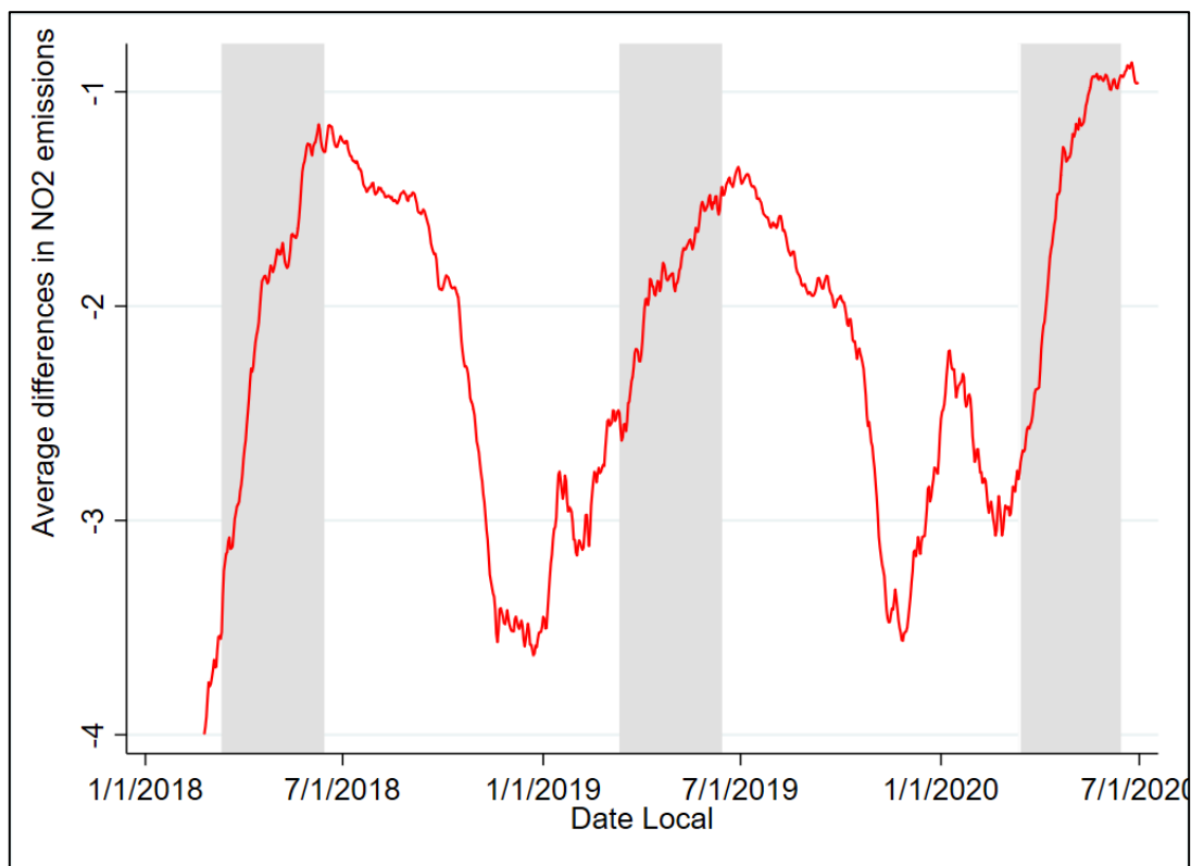
Figure 3. Differences in Republican-Democratic NO 2 average levels
