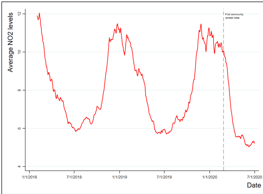
Figure 2: Evolution of average NO 2 levels
