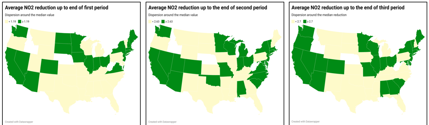
Figure 4. Average pollutants reduction in the three periods
