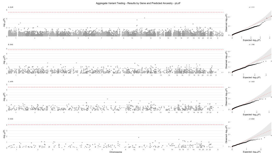
Figure 23: Gene-level manhattan and Q-Q plots per predicted ancestry for the pLof mask. Each point in the manhattan plot represents a gene. Panels from top to bottom are for EUR (A), SAS (B), AFR (C) and EAS (D). The red dashed lines indicate Bonferonni corrected "gene-wide" P -values (see Table 4).
