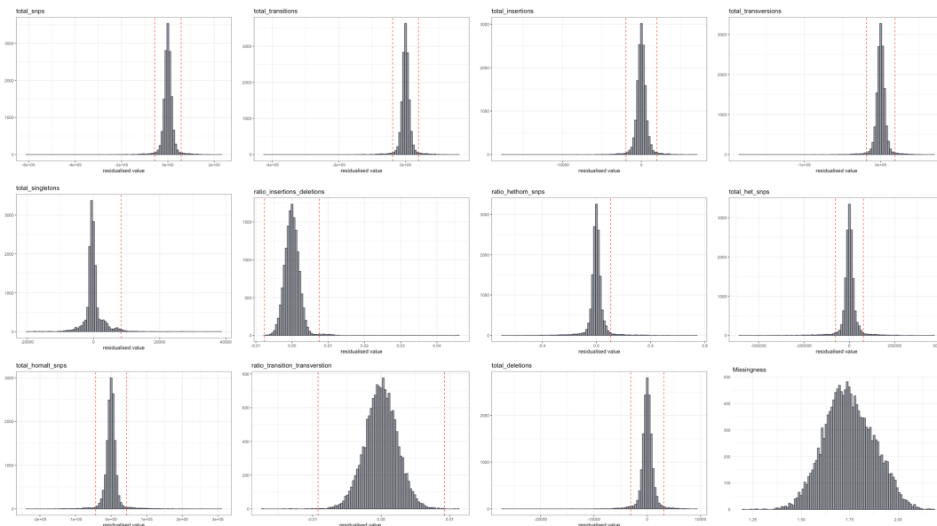
Figure 2: Each histogram shows the distribution of samples in the aggCOVID v4.2 data-set for a particular VCF-level quality metric, following adjustment for sequencing platform and the first three ancestry assignment principal components (as described in Methods). All metrics are calculated from autosomal bi-allelic SNVs. The dashed red lines indicate the threshold for sample exclusion. Samples were removed that were four median absolute deviations (MADs) above or below the median for the following metrics: ratio heterozygous-homozygous, ratio insertions-deletions, ratio transitions-transversions, total deletions, total insertions, total heterozygous snps, total homozygous snps, total transitions, total transversions. For the number of total singletons (snps), samples were removed that were more than 8 MADs above the median. For the ratio of heterozygous to homozygous alternate snps, samples were removed that were more than 4 MADs above the median. For sample-missingness (bottom-right panel), a hard cut-off of 0.05 was applied (no adjustment for sequencing platform or ancestry).
