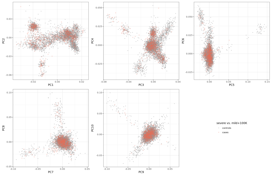
Figure 6: SAS PCs 1-10 for severe (cases) and mild + 100K individuals (controls).
