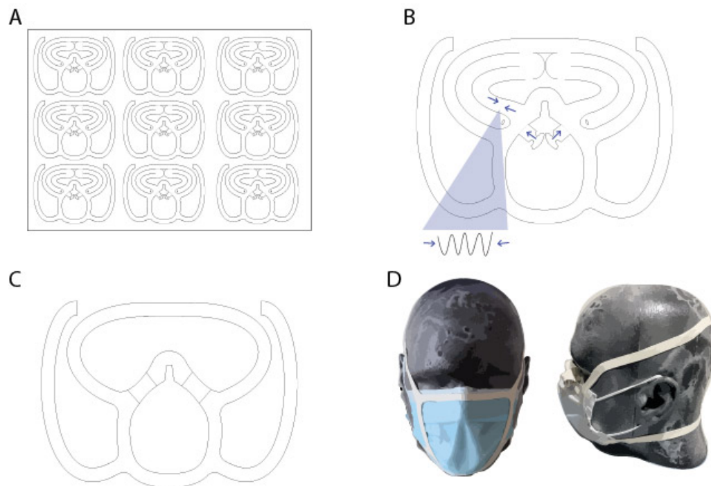
Figure 2: Harness designs production. Both harness designs 1, 2 and 2.1 were laser-cut using the epilog machine on a silicone material with a 1/32 inches in thickness (A). Harness Design 2 has more material in the nasal sidewalls area. The additional material is then folded multiple times (B) and secured around the nasal sidewalls (C). Once the material is secured, the harness is positioned over the surgical mask to improve the seal around the nose, cheeks and chin (D).
