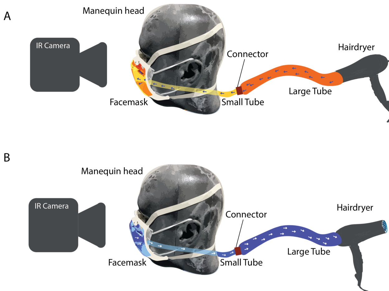
Figure 3: Mannequin Heads breathing simulation of exhalation (A) and Inhalation (B). Hairdryer introduces warm air into a large tube, which connects to a smaller tube directly in contact with the mannequin mouth. Warm air propagates inside the mask, and the seal efficiency is assessed using an IR camera. The protocol is performed for different mannequin sizes.
