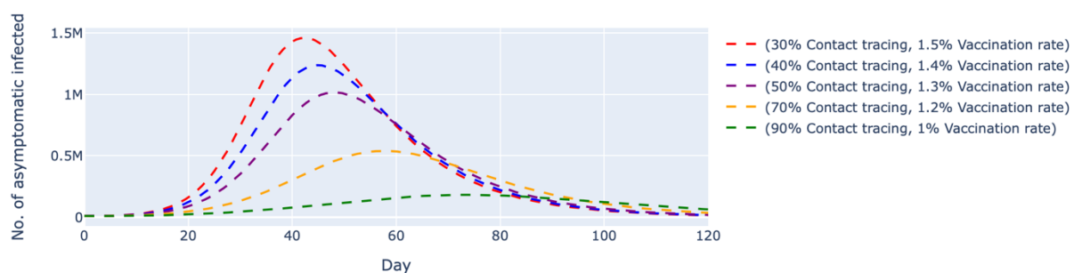
Figure 3a: Simulated number of untraced, COVID-19 asymptomatic cases with varied vaccination rates and contact tracing effectiveness. The vaccination rates per day were varied between 1% and 1.5%, which translates to approximately 320,000 and 480,000 doses of vaccine, respectively. The contact tracing effectiveness varied between 30% and 90%. The dashed lines represent the simulated number of untraced COVID-19 asymptomatic cases for five different contexts over 120 days.
