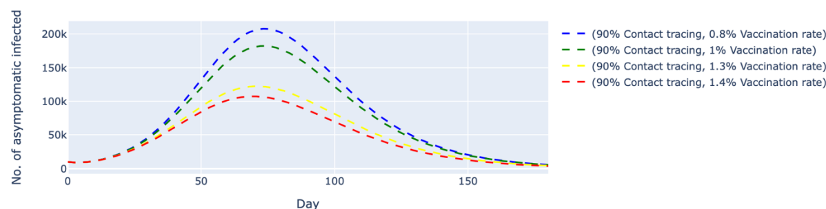
Figure 4a: Simulated number of untraced, COVID-19 asymptomatic cases with fixed contact tracing effectiveness at 90% and varied vaccination rates. The contact tracing effectiveness was fixed at 90% and the vaccination rates per day were varied between 0.8% and 1.4%, which translates to approximately 260,000 and 450,000 doses of vaccine, respectively. The dashed lines represent the simulated number of untraced COVID-19 asymptomatic cases for five different contexts over 160 days.
