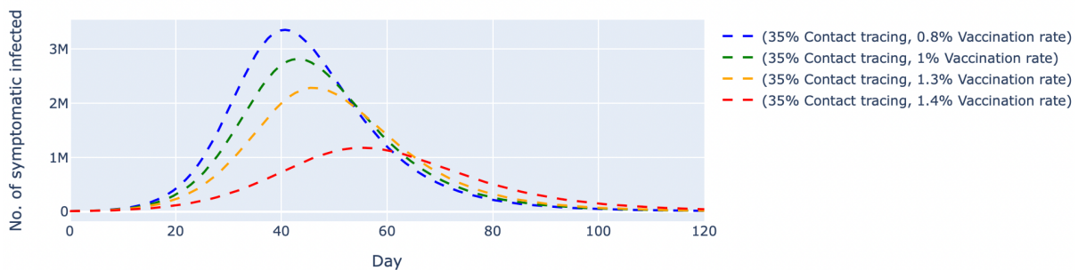
Figure 5b: Simulated number of untraced, COVID-19 symptomatic cases with fixed contact tracing effectiveness at 35% and varied vaccination rates. The contact tracing effectiveness was fixed at 35%, and the vaccination rates per day were varied between 0.8% and 1.4%, which translates to approximately 260,000 and 450,000 doses of vaccine, respectively. The dashed lines represent the simulated number of untraced COVID-19 symptomatic cases for five different contexts over 120 days.
