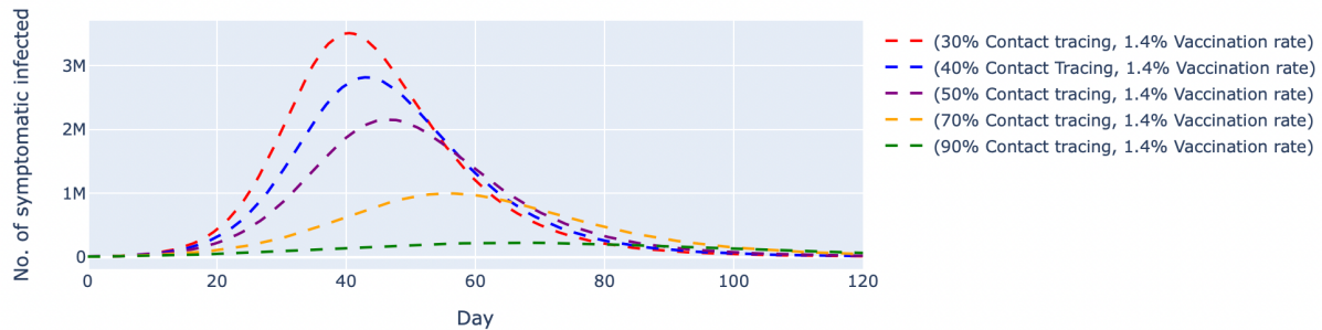
Figure 2b: Simulated number of untraced, COVID-19 symptomatic cases with fixed vaccination rate and varied contact tracing effectiveness. The vaccination rate per day was fixed at 1.4%, which translates to approximately 450,000 doses of vaccine, and the contact tracing effectiveness varied between 30% and 90%. The dashed lines represent the simulated number of untraced COVID-19 symptomatic cases for five different contexts over 120 days.
