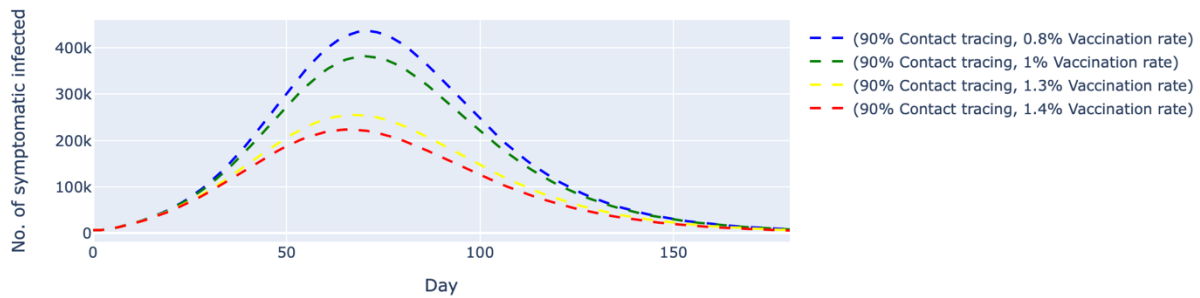
Figure 4b: Simulated number of untraced, COVID-19 symptomatic cases with fixed contact tracing effectiveness at 90% and varied vaccination rates. The contact tracing effectiveness was fixed at 90% and the vaccination rates per day were varied between 0.8% and 1.4%, which translates to approximately 260,000 and 450,000 doses of vaccine, respectively. The dashed lines represent the simulated number of untraced COVID-19 symptomatic cases for five different contexts over 160 days.
