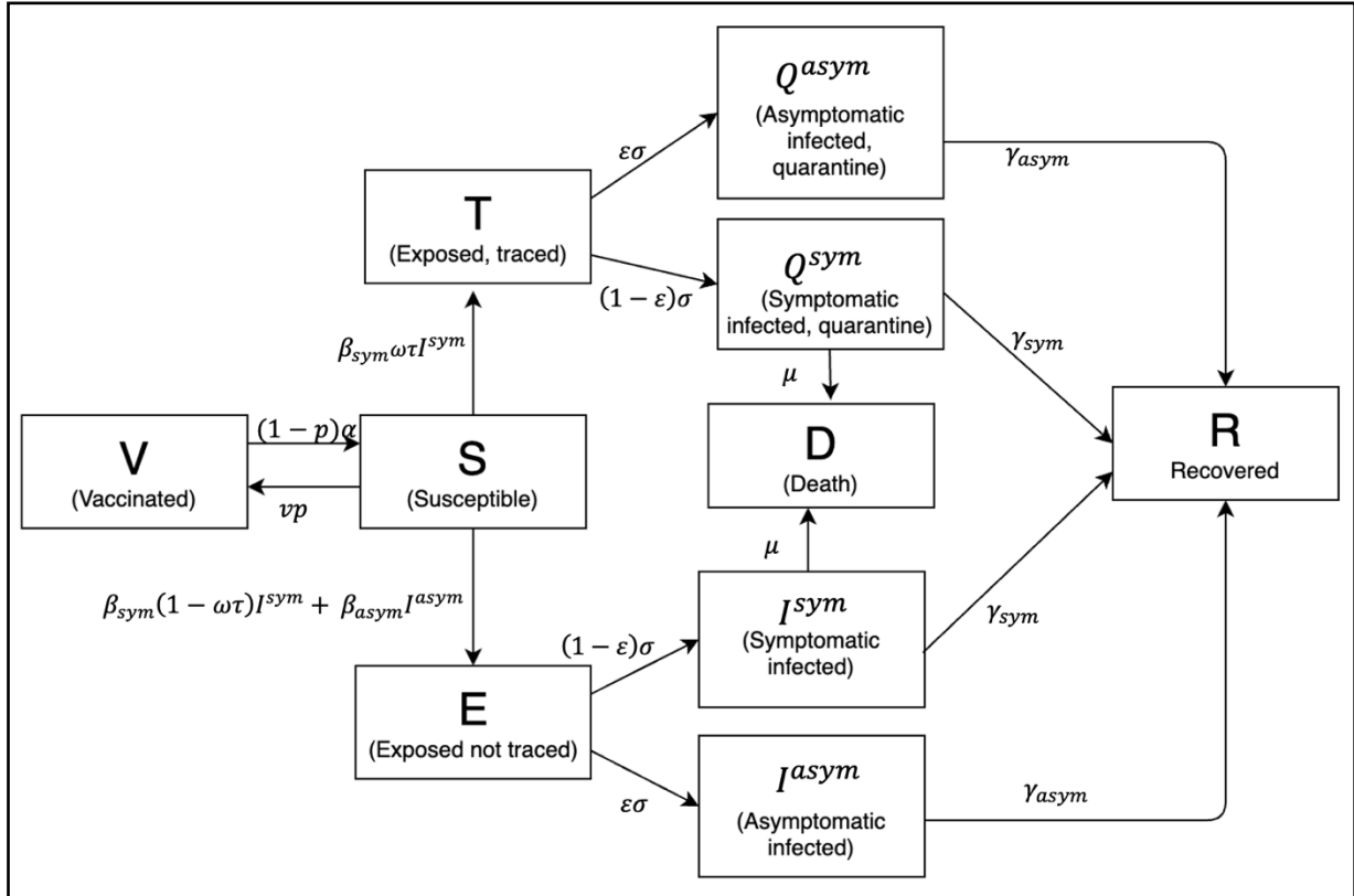
Figure 1: Transmission diagram of the SEIRV model.
