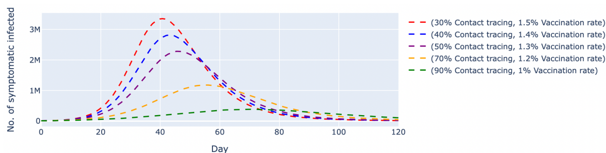
Figure 3b: Simulated number of untraced, COVID-19 symptomatic cases with varied vaccination rates and contact tracing effectiveness. The vaccination rates per day were varied between 1% and 1.5%, which translates to approximately 320,000 and 480,000 doses of vaccine, respectively. The contact tracing effectiveness varied between 30% and 90%. The dashed lines represent the simulated number of untraced COVID-19 symptomatic cases for five different contexts over 120 days.
