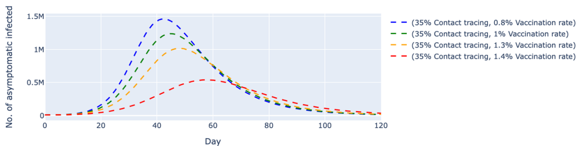
Figure 5a: Simulated number of untraced, COVID-19 asymptomatic cases with fixed contact tracing effectiveness at 35% and varied vaccination rates. The contact tracing effectiveness was fixed at 35%, and the vaccination rates per day were varied between 0.8% and 1.4%, which translates to approximately 260,000 and 450,000 doses of vaccine, respectively. The dashed lines represent the simulated number of untraced COVID-19 asymptomatic cases for five different contexts over 120 days.
