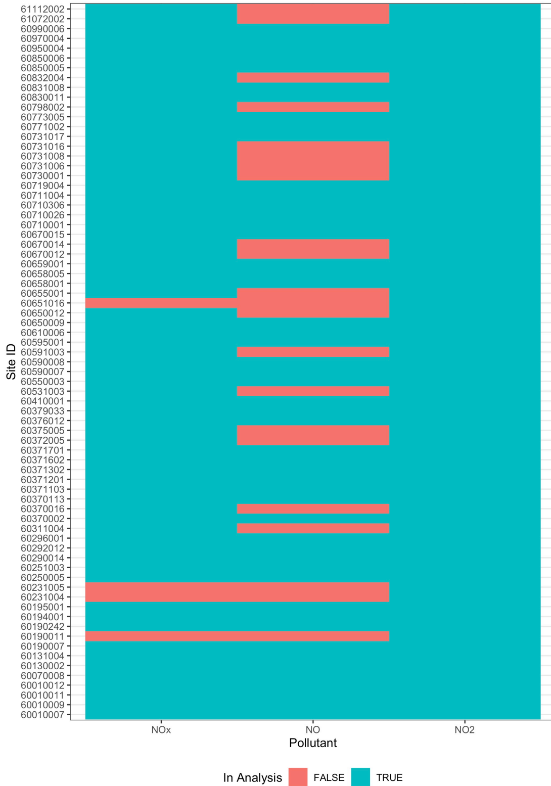
Figure S3. AQS sites included in the analysis of each pollutant (N=69 NOx, 51 NO, 73 NO 2 ). Site ID is a compilation of the CA state ID (6, the first digit), county ID (next 3 digits), and AQS site ID (last 4 digits).
