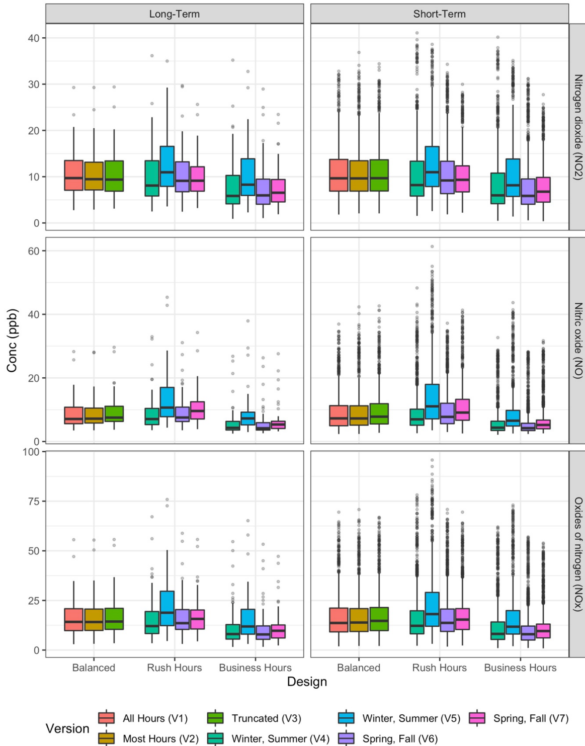
Figure S7. Annual average site concentration estimates for different pollutants and design versions. N=30 campaigns per design version \times 69 sites for short-term approaches; N = 1 campaign per design version \times 69 sites for long-term approaches. Short-term approaches appear to be more variable (less precise), in large part because all 30 campaigns are represented in the boxplots.
