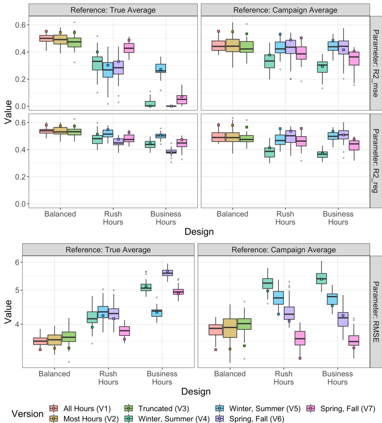
Figure S15. \text{NO}_2 Model performances ( R^2_{\text{MSE}} , R^2_{\text{reg}} , and RMSE), as determined by each campaign's cross-validated predictions relative to: a) the true averages (long-term Balanced Version 1), and b) its campaign averages. Boxplots are for short-term approaches (30 campaigns), while squares are for long-term approaches (1 campaign).
