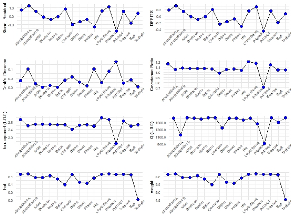
Fig. 11a) Influence analysis. Fully vaccinated, any positive PCR. Influential analysis subplot graphs included the influence estimates for each study in fully vaccinated meta-analysis. No study exceeded the cut-offs to define an influential case; however, "Pritchard" study needed further investigation.[21]
