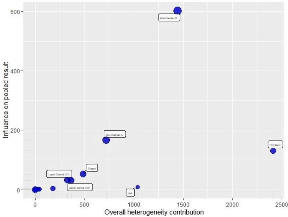
Fig.7b) Baujat plot. Partially vaccinated, any positive PCR. Contribute to overall heterogeneity Q(x) and effect size (y) . “Pritchard”, “Abu Raddad B” and “Hall” were the most influential on the overall heterogeneity. “Abu Raddad B” contributed the most to the pooled result.
