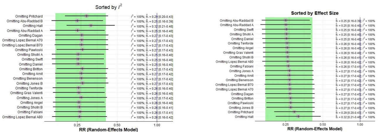
Fig.8) Leave-One-Out Analysis. Partially vaccinated, any positive PCR. The first plot shows that by omitting “Abu-Raddad B” study, the I^2 is slightly reduced. Moreover, “Swift”, “Daniel” and “Britton” contributed to the overall heterogeneity. In the second plot the overall effect estimate changed with two studies removed. In particular, by removing “Pritchard” the RR increased to 0.29, while RR increased to 0.32 after removing “Hall”.
