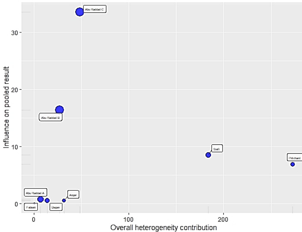
Fig.23b) Baujat plot. Fully vaccinated, symptomatic PCR. Contribute to overall heterogeneity, Q(x) and effect size (y). “Pritchard” and “Swift” studies contributed to the pooled imbalance. “Abu Raddad C” was the most influential on the pooled effect size.
