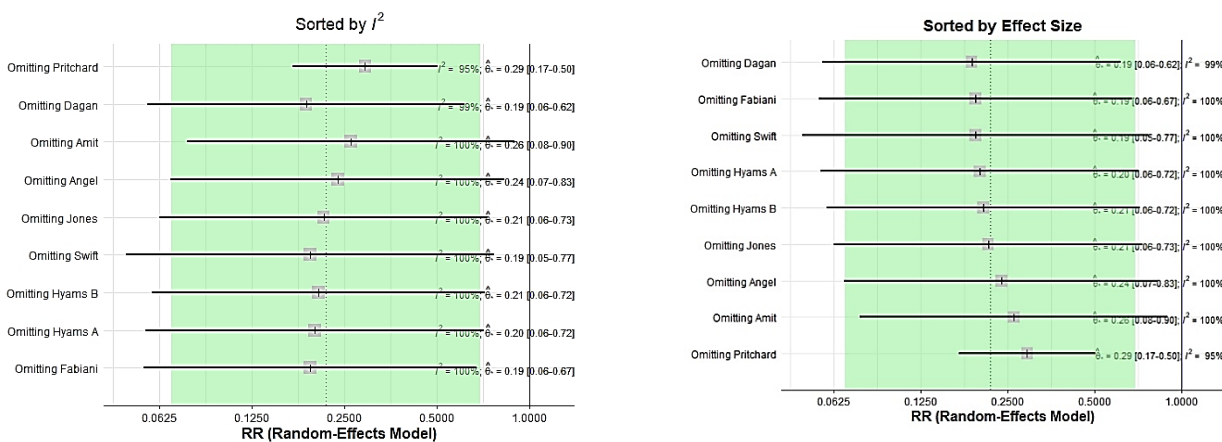
Fig.20) Leave one out analysis. Partially vaccinated, symptomatic PCR. The first plot displays the change on the I2 heterogeneity attained by removing one study at each step. The best result on the pooled imbalance was achieved by omitting “Pritchard”. The second plot indicates how the omission of “Dagan” influenced the overall RR estimate.
