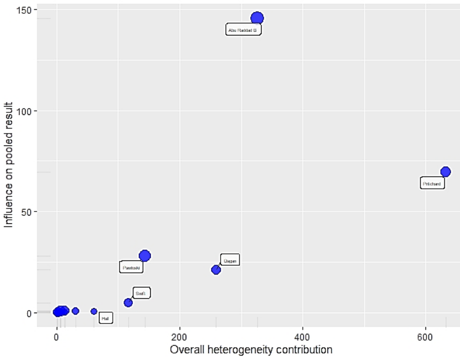
Fig. 11b) Baujat plot. Fully vaccinated, any positive PCR. Contribute to overall heterogeneity (Q) and effect size. “Pritchard” and “Abu-Raddab B” contributed to the pooled imbalance. “Abu Raddad B” was the most influential on pooled effect size.
