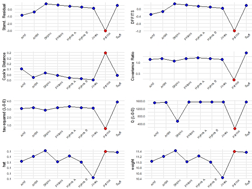
Fig.19a) Influence analysis. Partially vaccinated, symptomatic positive Sars-Cov-2 PCR. “Pritchard” (red dot) results as the most influential study as it exceeds the cut-offs defined by Viechtbauer and Cheung in any subplot. [21]
