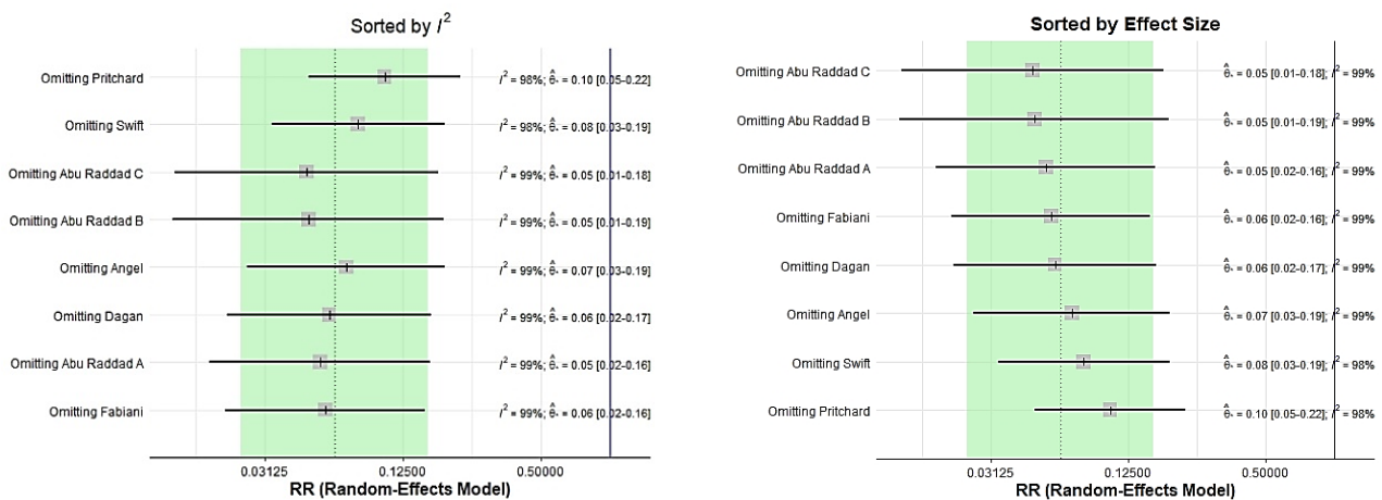
Fig.24) Leave one out analysis. Fully vaccinated, symptomatic PCR. The first plot displayed the change on the I^2 heterogeneity attained by removing one study at each step. “Pritchard” was the most influential on the pooled imbalance, while “Abu Raddad” affected the overall RR estimate.
