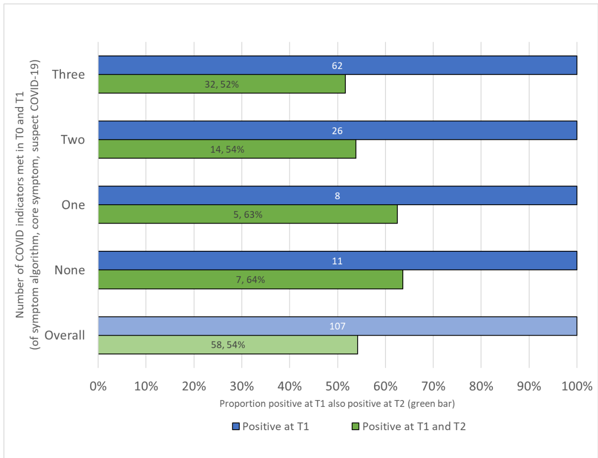
Figure S5 Numbers and proportion of those reporting 0, 1, 2 or 3 COVID indicators who were positive at two time-points
