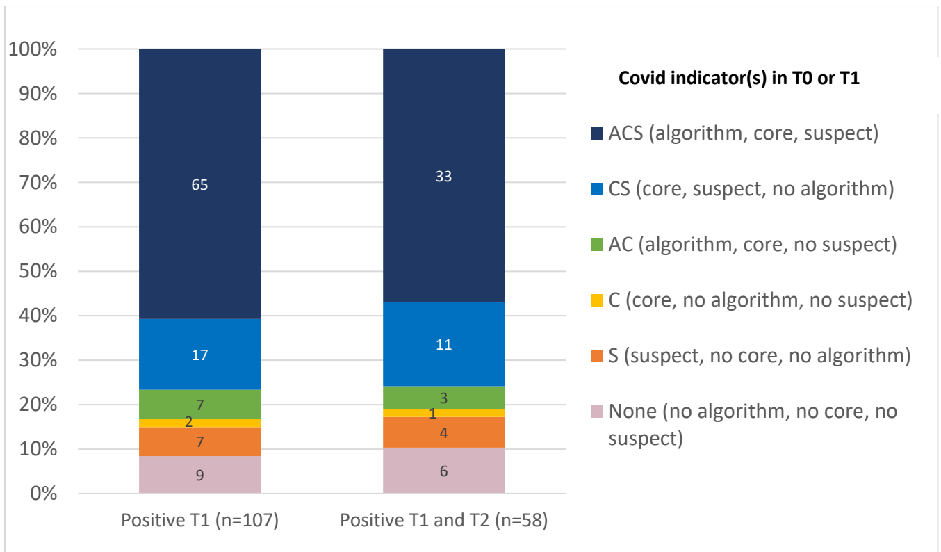
Figure S4 Profile of COVID indicators reported in T0 to T1 in those who were positive for antibodies at T1 and those positive at both T1 and T2
