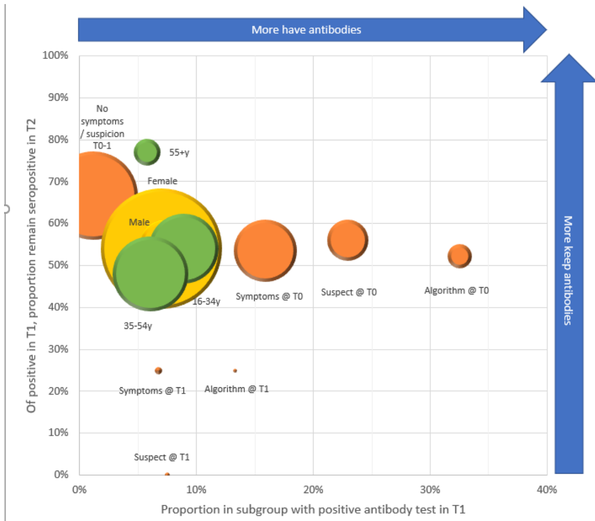
Figure S3 Bubble chart of the relationship of probability seropositive at T1 versus remaining seropositive at T2, according to (1) symptoms or suspicion status, orange; (2) gender, yellow; (3) age, green. Size of bubble reflects number of people in subgroup.
