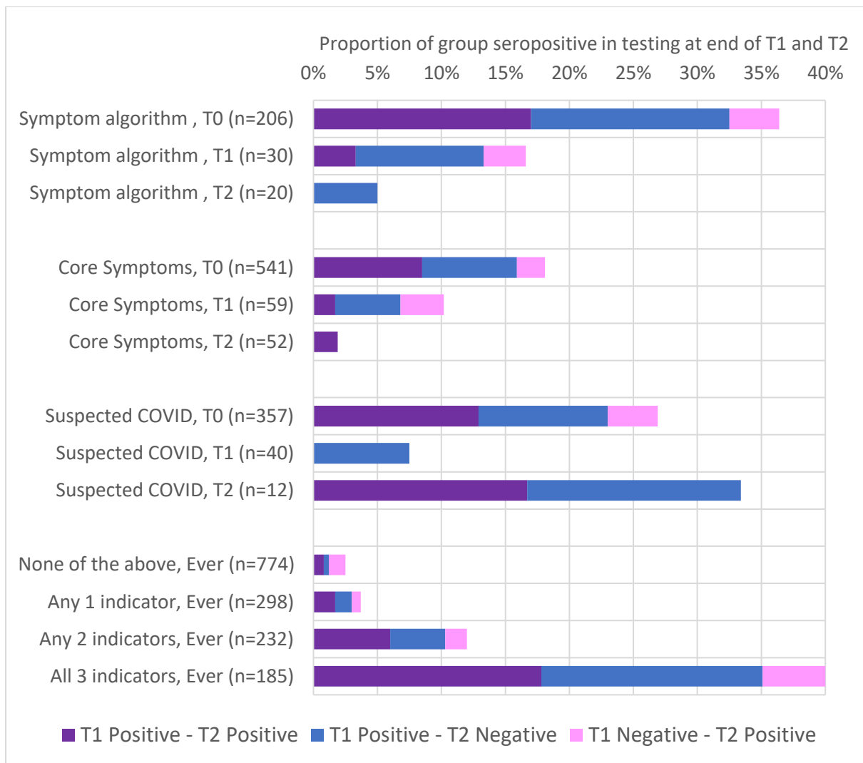
Figure S2 Proportion of group seropositive and sequence of tests by COVID-19 indicators and timing (see table 3 for numbers)
