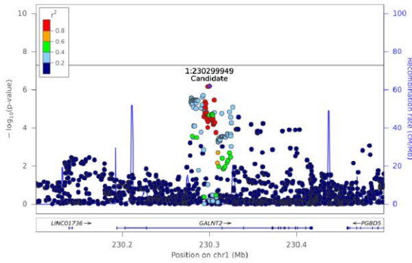
TG(54:2) [NL-18:0] - Chr 1 (230100836-230499925)
