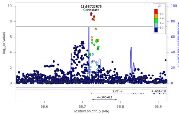
DG(18:1_20:4) - Chr 15 (58524080-58923206)
