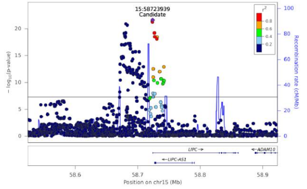
PE(38:5) (a) - Chr 15 (58524080-58923790)
