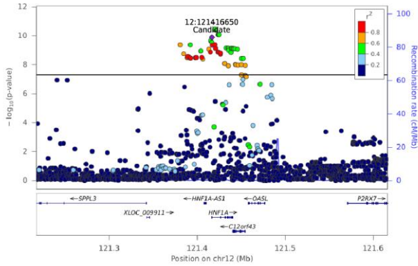
PC(36:0) - Chr 12 (121216911-121616464)
