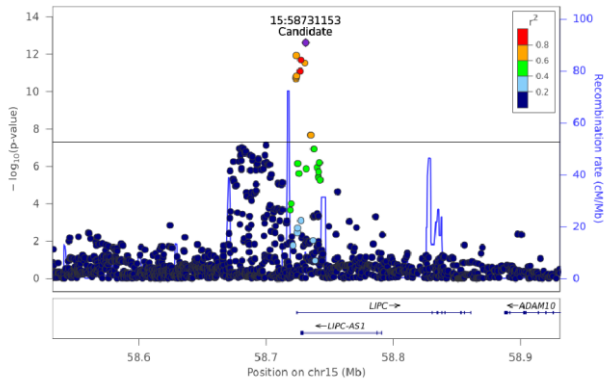
TG(56:6) [NL-20:4] - Chr 15 (58532076-58931039)
