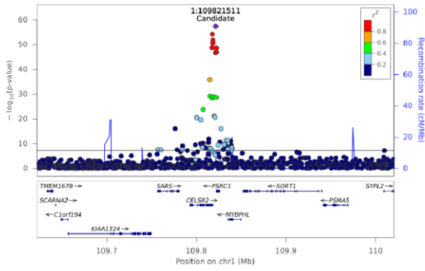
Total HexCer - Chr 1 (109621861-110020621)
