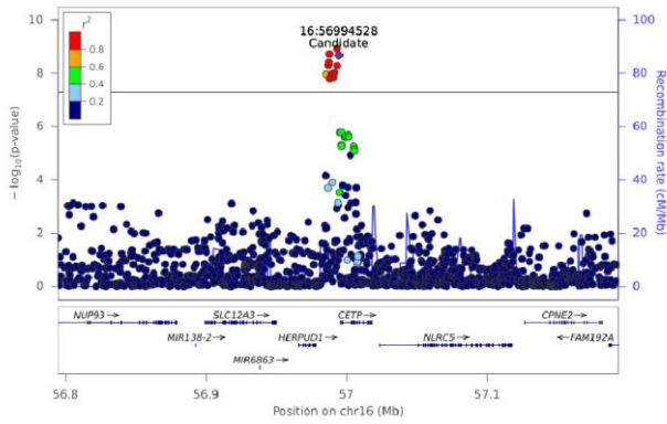
TG(O-50:1) [NL-16:0] - Chr 16 (56794590-57193448)
