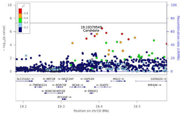
LPC(20:3) [sn1] - Chr 19 (19179819-19579046)
