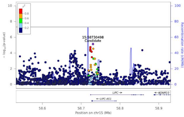
Total PC - Chr 15 (58532076-58930416)
