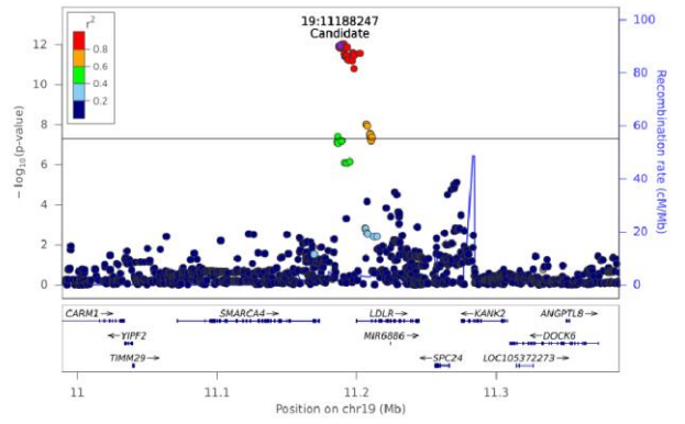
Total COH - Chr 19 (10988818-11388151)
