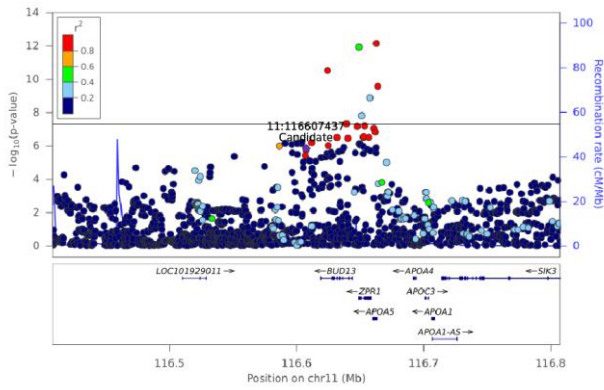
TG(54:4) [NL-18:0] - Chr 11 (116407583-116807368)
