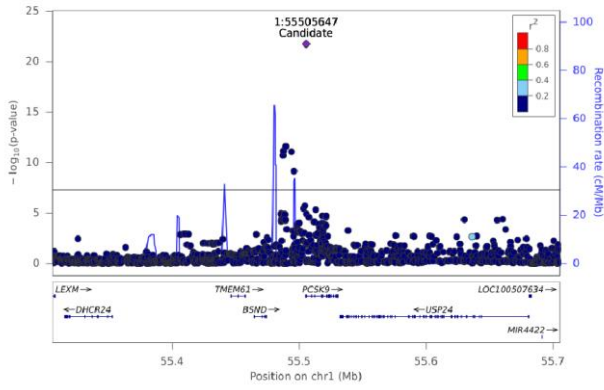
Total CE - Chr 1 (55305731-55705623)
