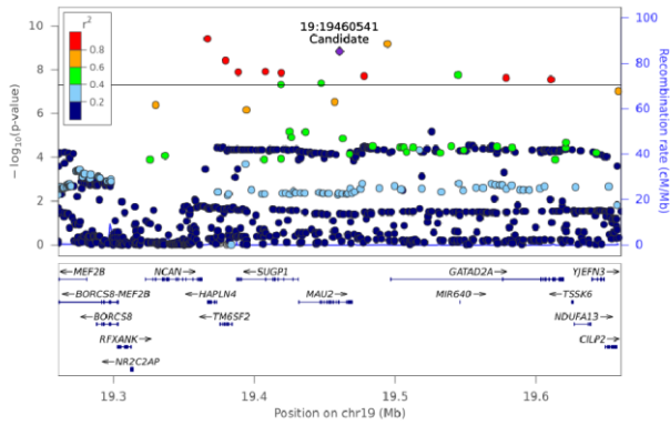
TG(50:2) [NL-18:1] - Chr 19 (19260686-19660523)
