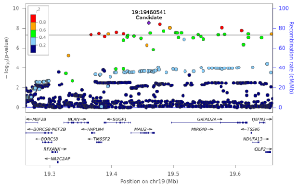
TG(50:2) [NL-18:1] - Chr 19 (19260686-19660523)
