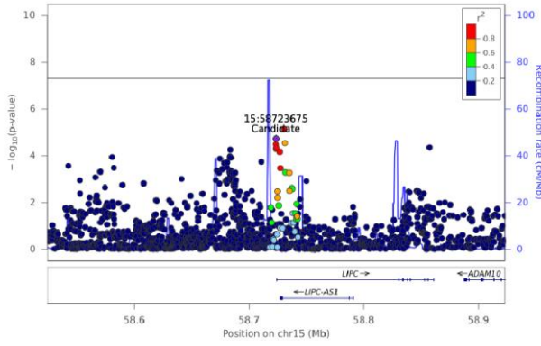
LPE(20:4) [sn1] - Chr 15 (58524080-58923206)
