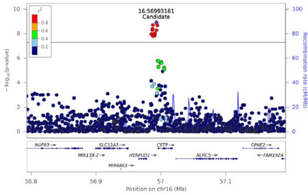
TG(O-50:1) [NL-16:0] - Chr 16 (56793346-57192310)
