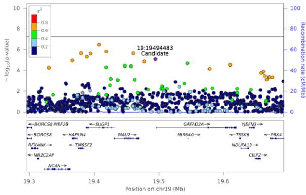
Total Cer - Chr 19 (19295556-19693426)
