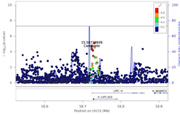
PG(34:2) - Chr 15 (58524080-58923790)
