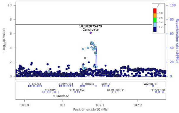
LPC(16:1) [sn1] - Chr 10 (101875936-102275471)
