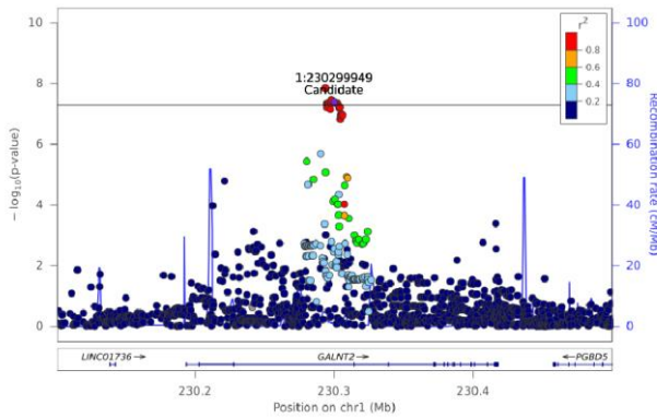
TG(54:3) [NL-18:1] - Chr 1 (230100836-230499925)
