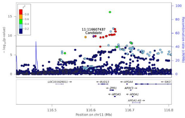
TG(54:4) [NL-18:2] - Chr 11 (116407583-116807368)
