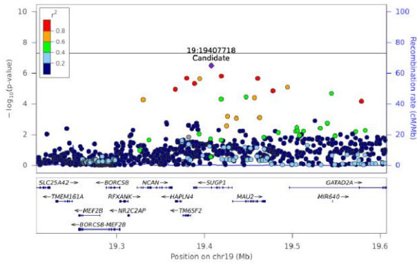
DG(18:1_20:4) - Chr 19 (19208076-19607564)
