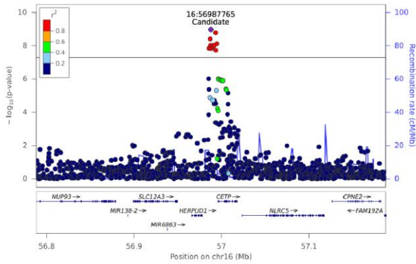
TG(O-52:2) [NL-16:0] - Chr 16 (56787882-57187761)
