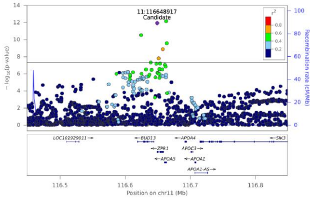
TG(54:2) [NL-18:0] - Chr 11 (116448927-116848857)
