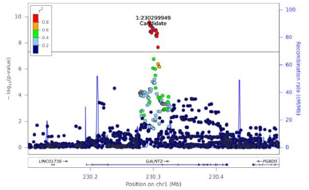
DG(16:0_18:1) - Chr 1 (230100836-230499925)
