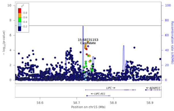
LPE(20:4) [sn1] - Chr 15 (58532076-58931039)
