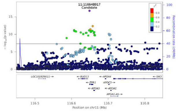
TG(54:4) [NL-18:0] - Chr 11 (116448927-116848857)
