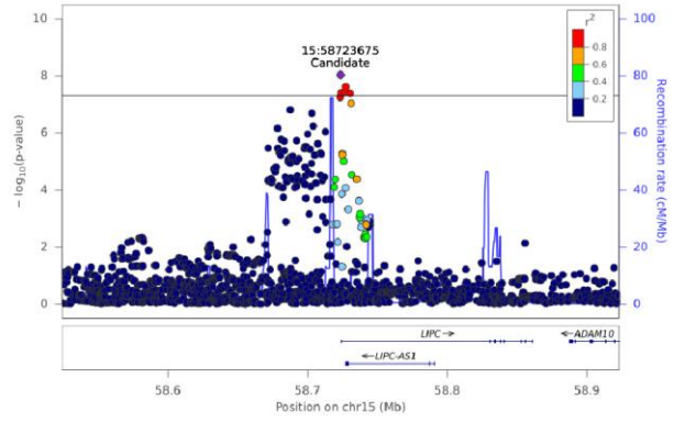
LPE(22:6) [sn2] - Chr 15 (58524080-58923206)
