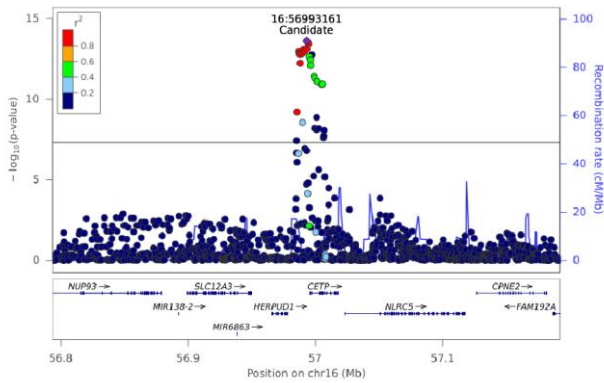
Total TG(O) - Chr 16 (56793346-57192310)
