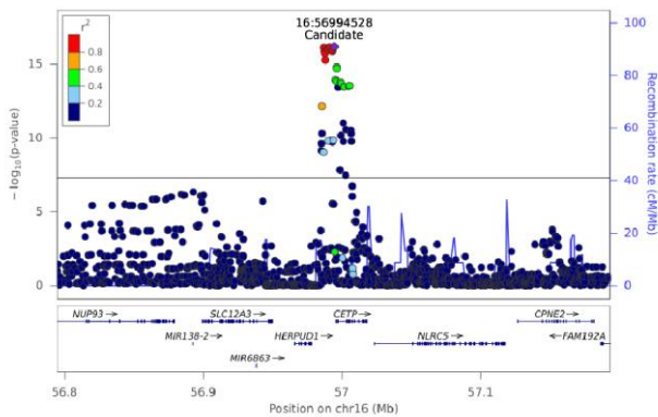
Total TG(O) - Chr 16 (56794590-57193448)
