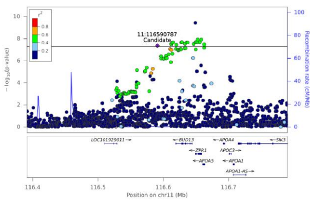
TG(54:1) [NL-18:1] - Chr 11 (116391073-116789849)
