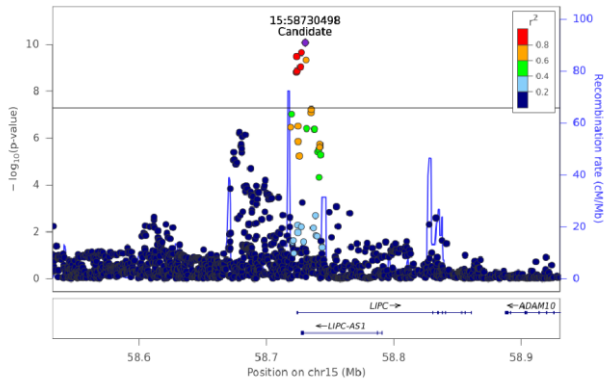
PC(16:0_18:1) - Chr 15 (58532076-58930416)
