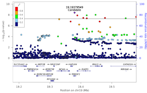
PC(18:1_20:3) - Chr 19 (19179819-19579046)
