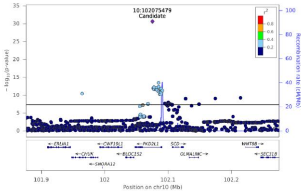
LPC(16:1) [sn2] - Chr 10 (101875936-102275471)
