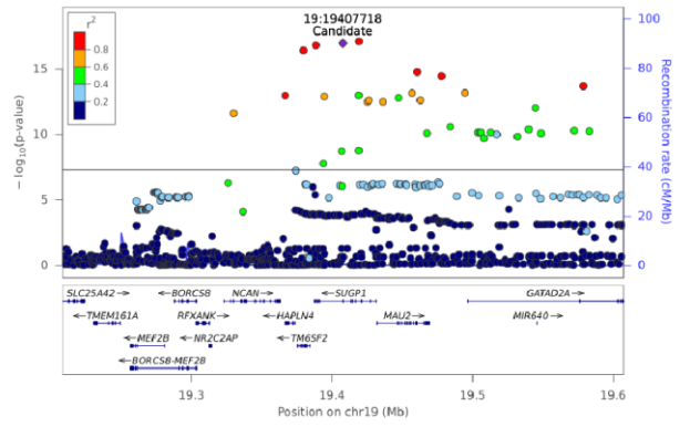
PC(14:0_20:4) - Chr 19 (19208076-19607564)
