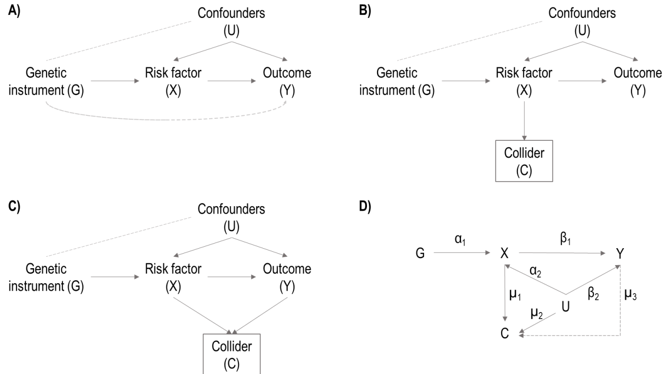
Figure 1. Directed Acyclic Graphs (DAGs) illustrating relationships between the variables.
