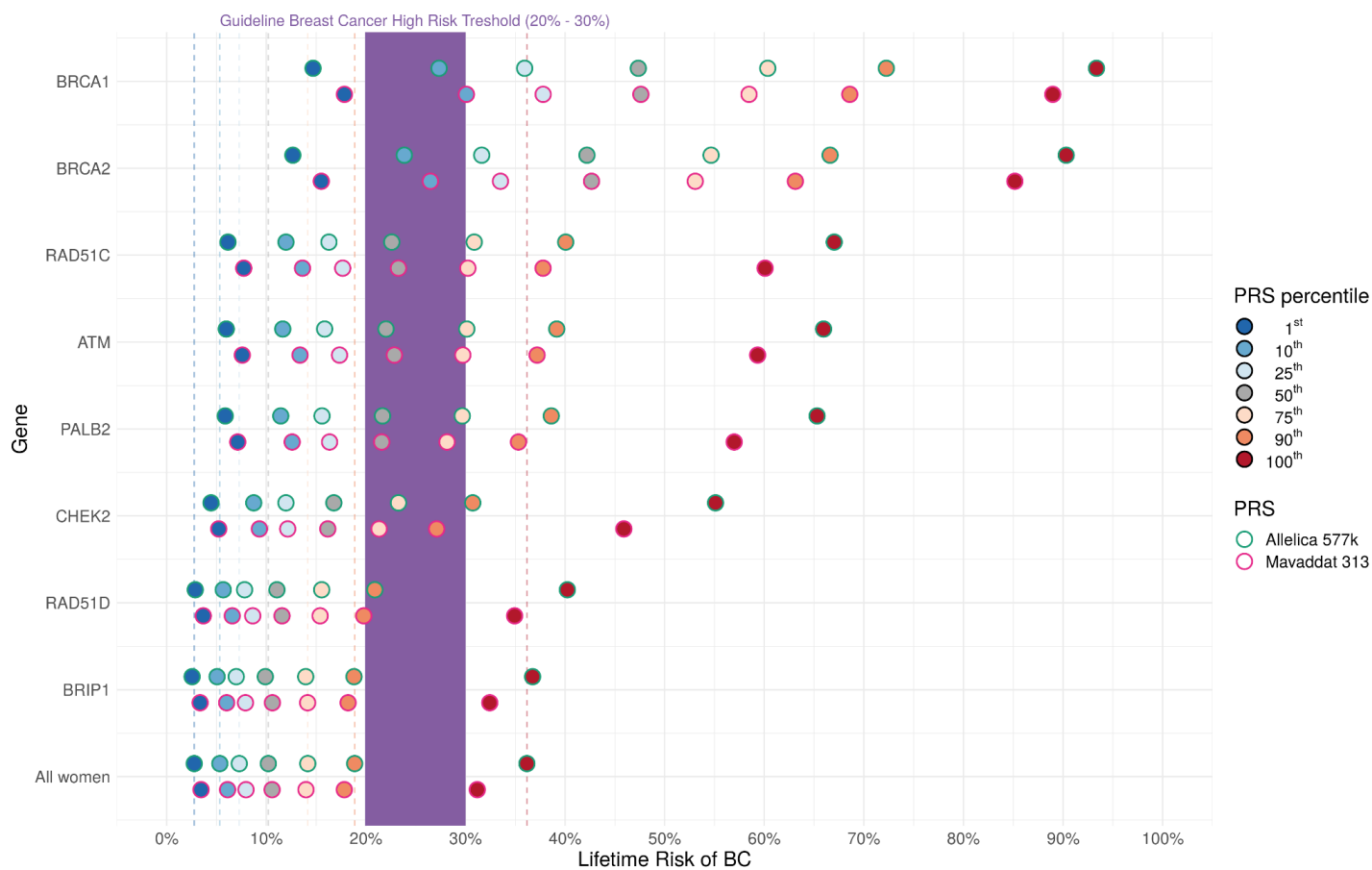
Supplementary Figure: PRS modulates the penetrance of 8 BC susceptibility genes. As Figure 1 with the inclusion of percentiles of the Mavaddat 313 SNP PRS 17 . We identified carriers of pathogenic variants in 8 breast cancer susceptibility genes in whole exome sequence data in 86,385 women in the UK Biobank. For each gene we show the predicted lifetime risk for carriers across a range of different PRS percentiles for the Allelica 577k PRS. An equivalent model without carrier status was built using all Non carriers (Non carriers). Dashed lines show lifetime risk for percentiles of the Allelica 577k PRS distribution in Non-carriers. American Cancer Association guidelines state that a threshold of 20% lifetime risk equates to High Risk 20 . We estimated lifetime risk of BC with a Cox proportional hazards regression for each gene separately in a model that included case/control status, age of enrollment and age of disease in the survival function, and carrier status, PRS, 4 PCs and genotyping array as covariates.
