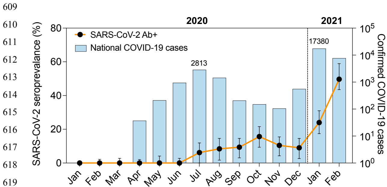
619 620 621 Figure 1. Overall SARS-CoV-2 adjusted seroprevalence over time superimposed on Malawi 622 national PCR-confirmed COVID-19 cases. Black dots (together with 95% CI) are estimated 623 seroprevalence at each timepoint (month), adjusted for assay sensitivity and specificity. The 624 histograms represent confirmed national COVID-19 cases per month, including 625 asymptomatic and symptomatic cases. Case frequency reported above histograms (June 626 2020 and February 2021) indicates reported cases at the peak of 1st and 2nd wave, 627 respectively. Vertical dotted line defines transition from 2020 to 2021. SARS-CoV-2 = Severe 628 acute respiratory syndrome coronavirus 2, COVID-19 = Coronavirus disease 2019, Ab+ = 629 Positive for detection of anti- SARS-CoV-2 receptor binding domain (RBD) antibody.
