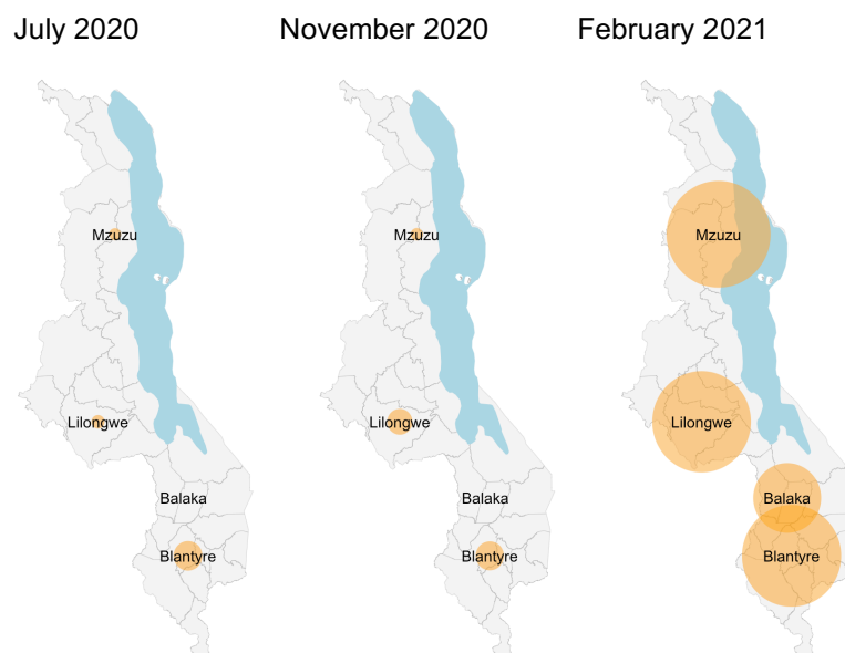
Figure 3. Seroprevalence bubble plot for overall seroprevalence at three snapshots in time. The size of the bubble is proportional to the prevalence of samples positive for anti-SARS-CoV-2 receptor binding domain (RBD) antibody within each location.
