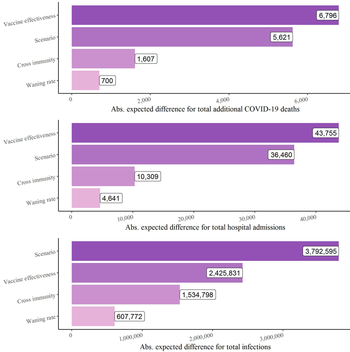
Figure S29: Absolute expected Shapley values for the model with pessimistic assumptions for total additional COVID-19 deaths (top), hospital admissions (middle), and COVID-19 infections (bottom) by 1 June 2022 (counted from 19 July 2021). Each plot is ordered from most important variable (top) to least (bottom), according to the expected absolute Shapley value with expectations taken over feature levels.
