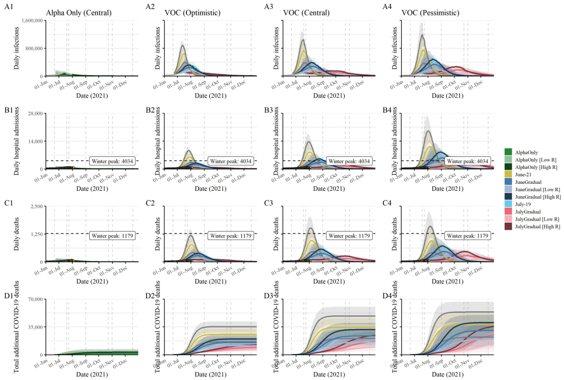
Figure S24: Forward projections for states under different assumptions and scenarios. (A1-D1) counterfactual without seeding of Delta. (A2-D2) scenarios with Delta under optimistic immunity assumptions. (A3-D3) scenarios with Delta under central immunity assumptions. (A4-D4) scenarios with Delta under pessimistic immunity assumptions. (A1-A4) projected daily infections. (B1-B4) projected daily hospital admissions. (C1-C4) projected daily deaths. (D1-D4) projected total COVID-19 deaths up to 11 months after full lift.
