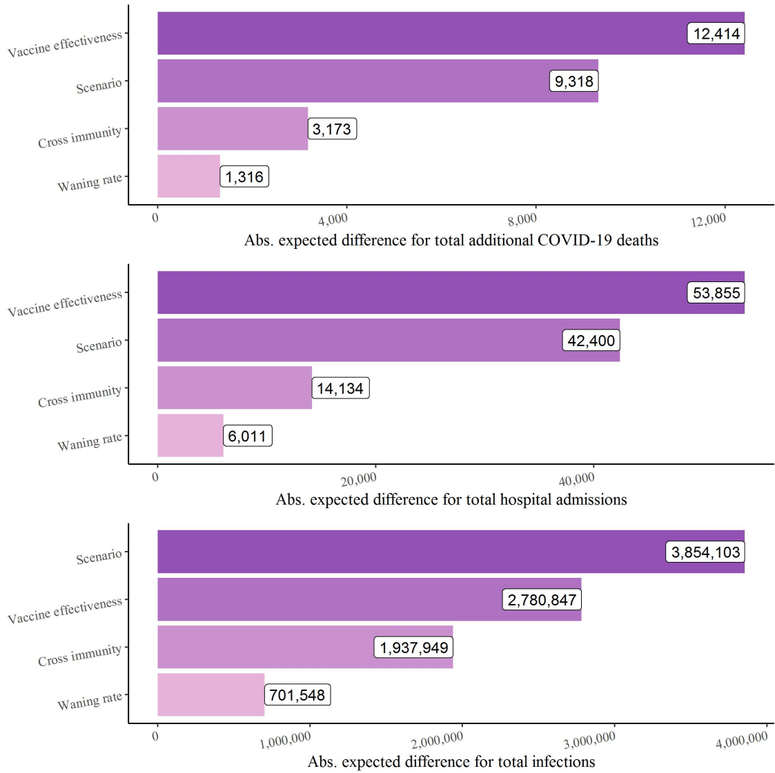
Figure S27: Absolute expected Shapley values for the model with central assumptions for total additional COVID-19 deaths (top), hospital admissions (middle), and COVID-19 infections (bottom) by 1 June 2022 (counted from 19 July 2021). Each plot is ordered from most important variable (top) to least (bottom), according to the expected absolute Shapley value with expectations taken over feature levels.
