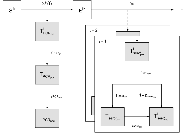
Figure S7: PCR positivity and seropositivity model structure flow diagram. Upon infection, an individual enters the pre-positive PCR compartment ( T_{PCR\_pre}^i ) before moving into the PCR positivity compartment ( T_{PCR\_pos}^i ) and then into the PCR negativity compartment ( T_{PCR\_neg}^i ). After a seroreversion period ( T_{sero\_pre}^i ), individuals can seroconvert ( T_{sero\_pos}^i ) or not ( T_{sero\_neg}^i ); if they do seroconvert, they eventually serorevert to T_{sero\_pos}^i .
