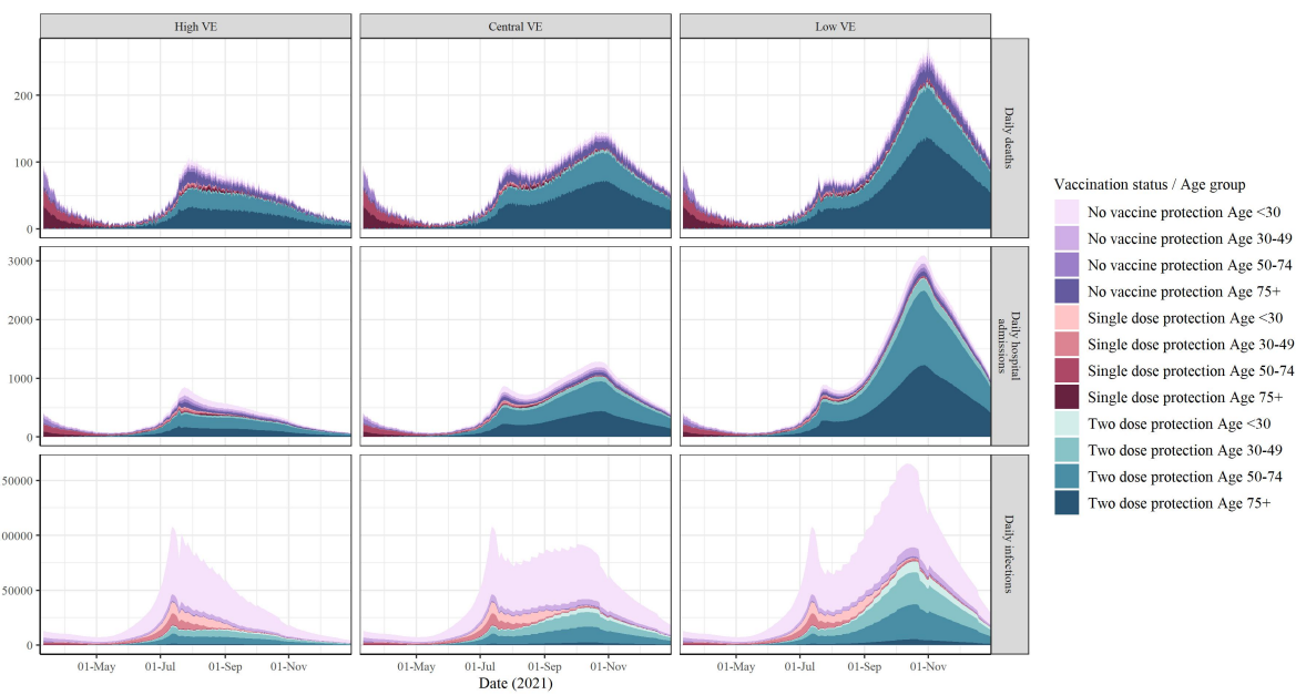
Figure S25: Simulations by age and vaccination status in the ‘July-19’ scenario. COVID-19 daily deaths (top), hospital admissions (middle), infections (bottom) by age group and vaccination status with optimistic (left), central (middle), and pessimistic (right) assumptions.
