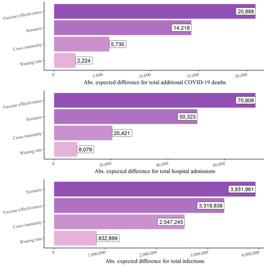
Figure S28: Absolute expected Shapley values for the model with optimistic assumptions for total additional COVID-19 deaths (top), hospital admissions (middle), and COVID-19 infections (bottom) by 1 June 2022 (counted from 19 July 2021). Each plot is ordered from most important variable (top) to least (bottom), according to the expected absolute Shapley value with expectations taken over feature levels.
