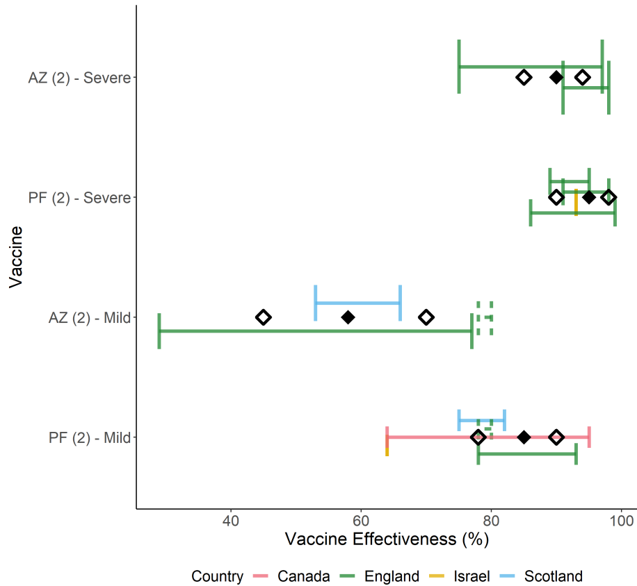
Figure S3: Comparison of our chosen Delta-specific VE values for two vaccine doses (Table S3) against associated 95% CrI values from the literature. Estimates taken from studies conducted in Canada [28], England [24, 22, 20, 27], Scotland [10], and Israel [29]. Black diamonds indicate our central assumptions, and hollow diamonds our pessimistic/optimistic assumptions. Dashed lines indicate a study that reported combined AZ/PF effect.
