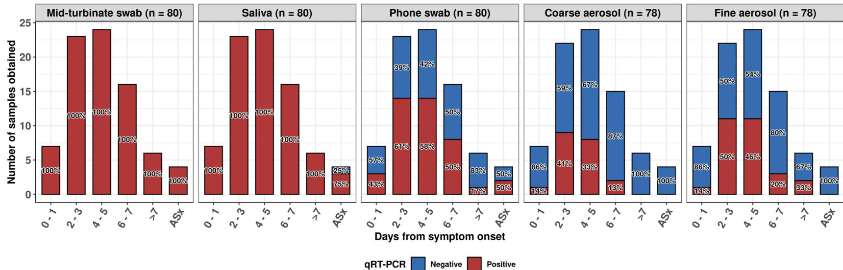
Figure S7. Positive and negative samples by day since onset.
