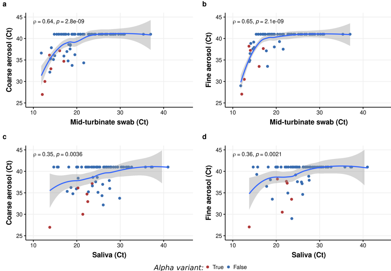
Figure S10. Correlation between the cycle threshold (Ct) values for SARS-CoV-2 N-gene in the upper respiratory samples (saliva and mid-turbinate swabs) and exhaled breath samples. Data shown are for samples collected without mask wearing. \rho = Spearman correlation coefficient.
