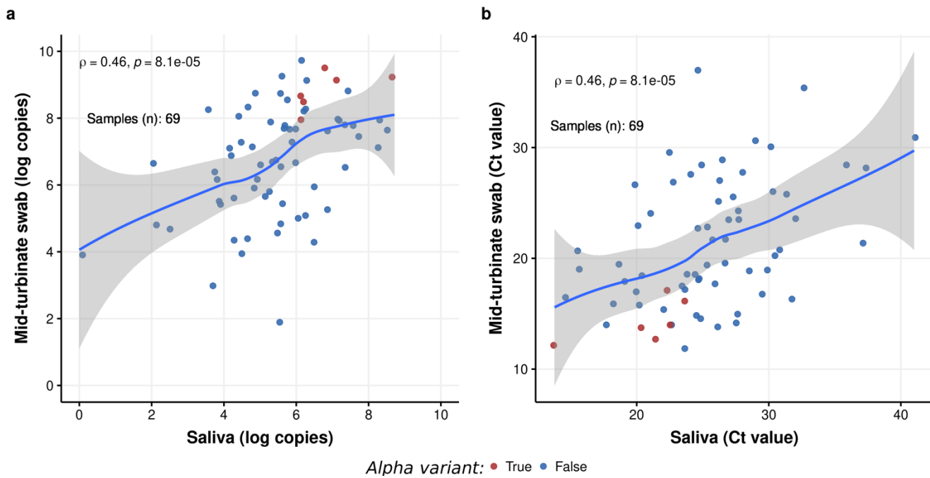
Figure S8. Correlation between saliva and mid-turbinate swab RNA measurements
