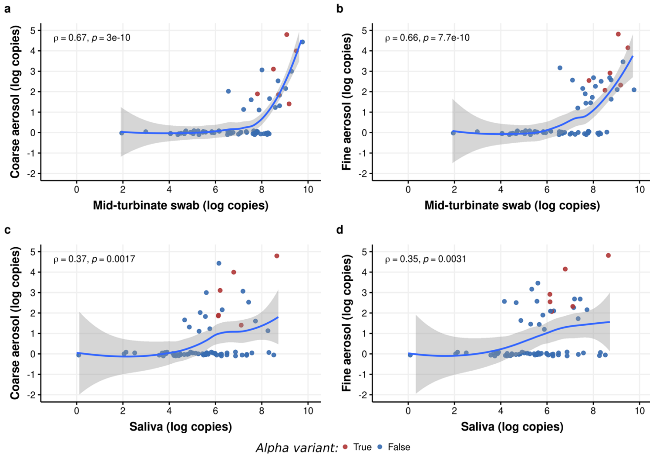
Figure S9. Correlation between the SARS-CoV-2 RNA copy numbers detected by qRT-PCR in upper respiratory samples (saliva and mid-turbinate swabs) and exhaled breath samples Data shown are for samples collected without mask wearing. \rho = Spearman\ correlation\ coefficient.
